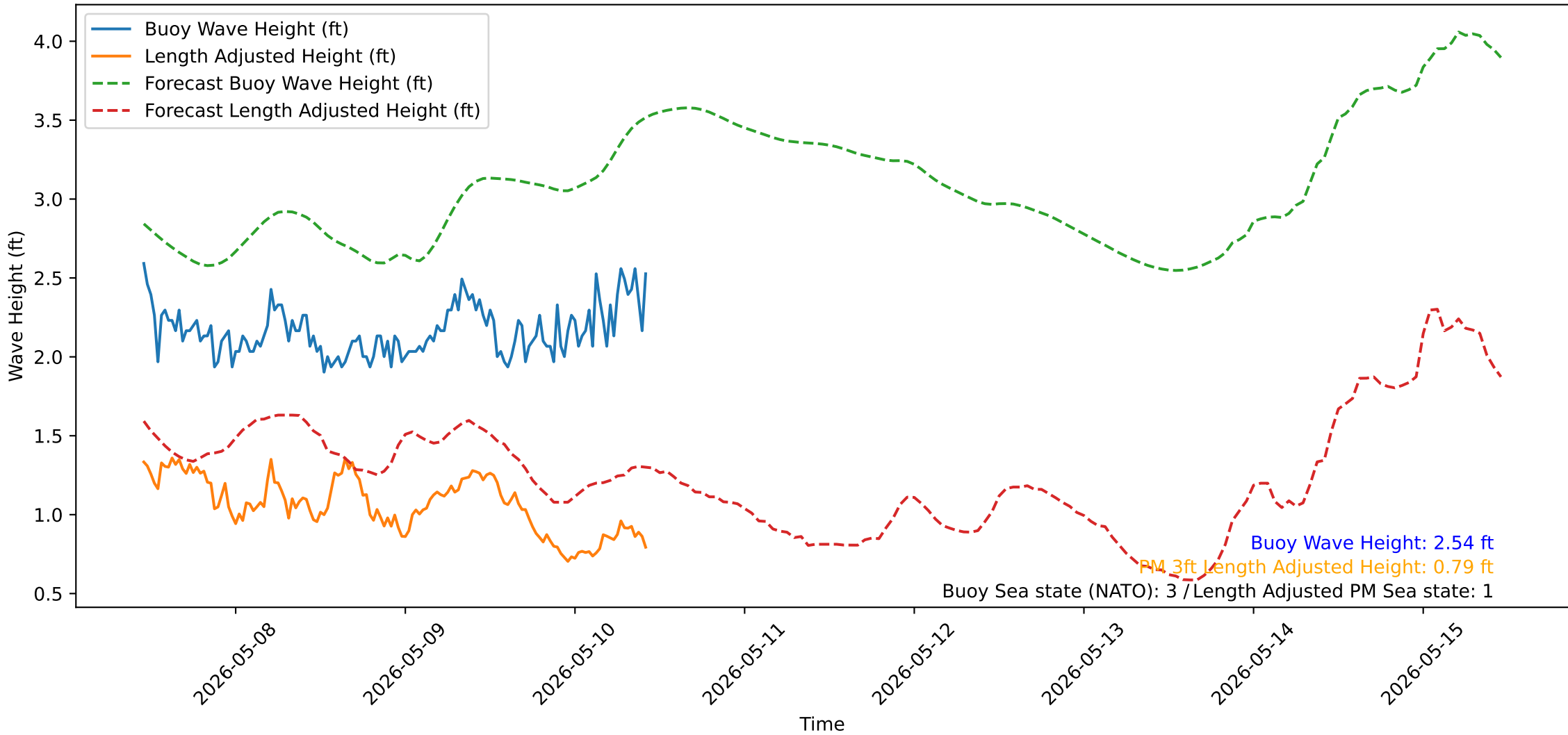
Wave Heights over Time for Red Beach at 2026-05-10 10:50:52
