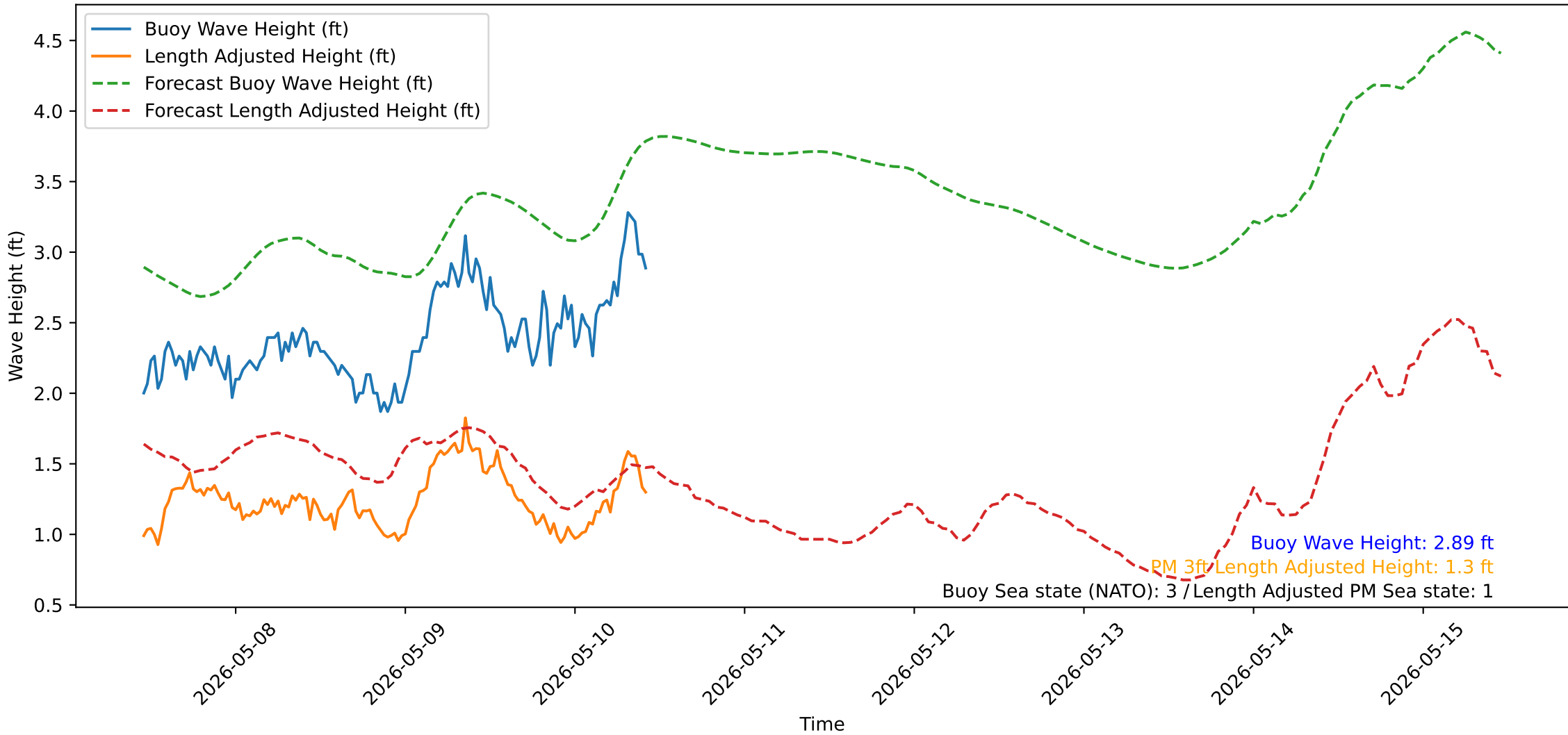
Wave Heights over Time for Oceanside Harbor at 2026-05-10 10:50:31
