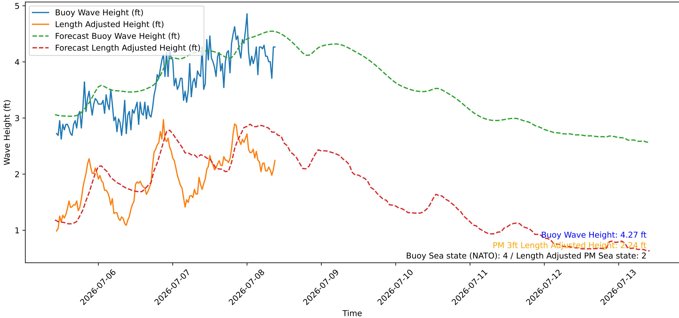
Wave Heights over Time for Red Beach at 2026-07-08 10:20:46
