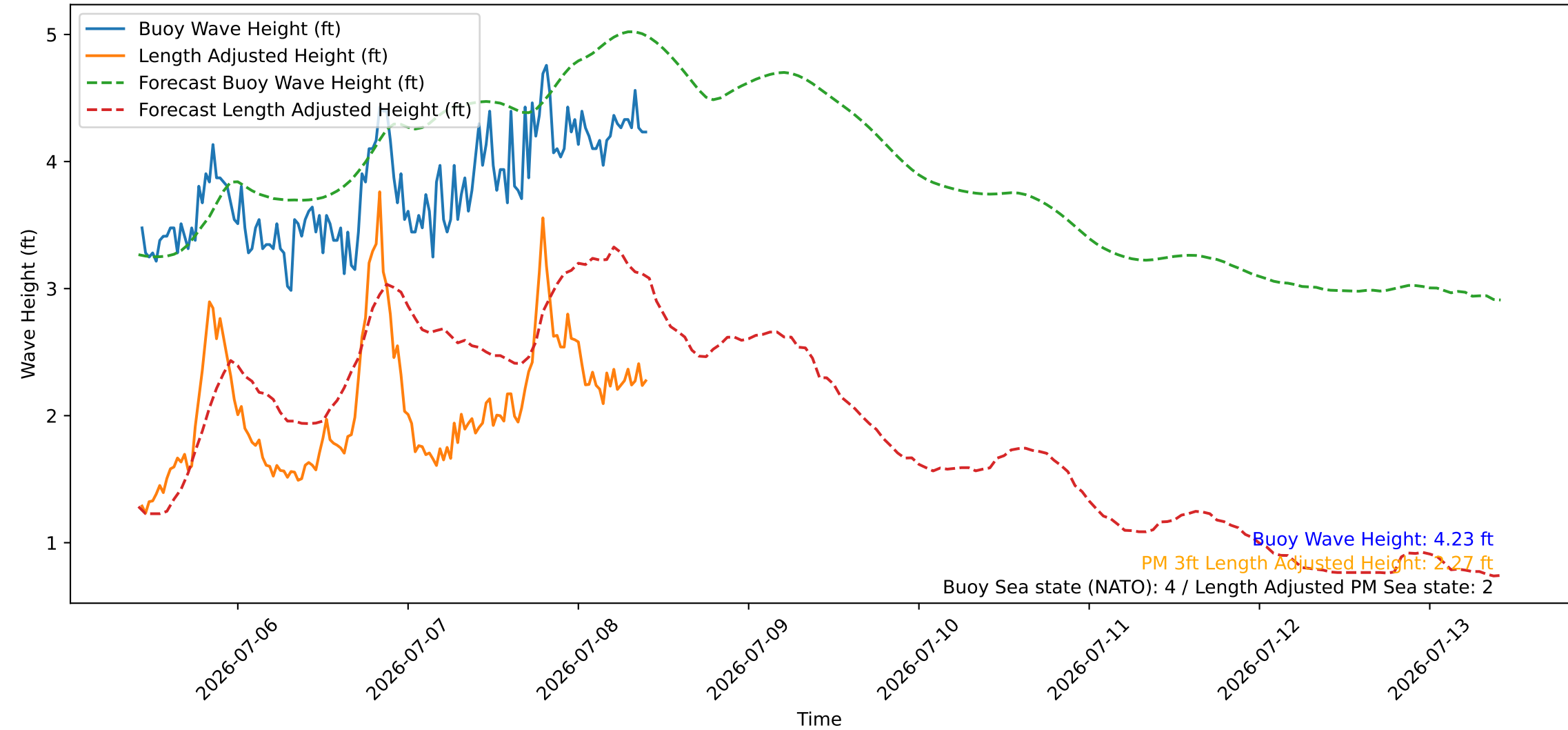
Wave Heights over Time for Green Beach at 2026-07-08 10:21:08
