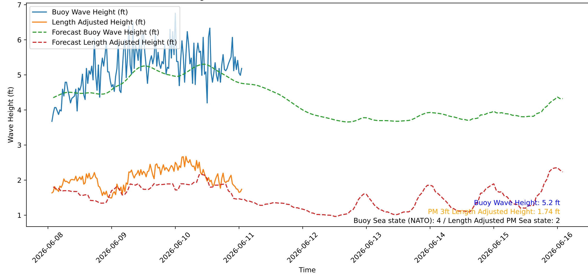
Wave Heights over Time for Oceanside Harbor at 2026-06-11 01:40:27
