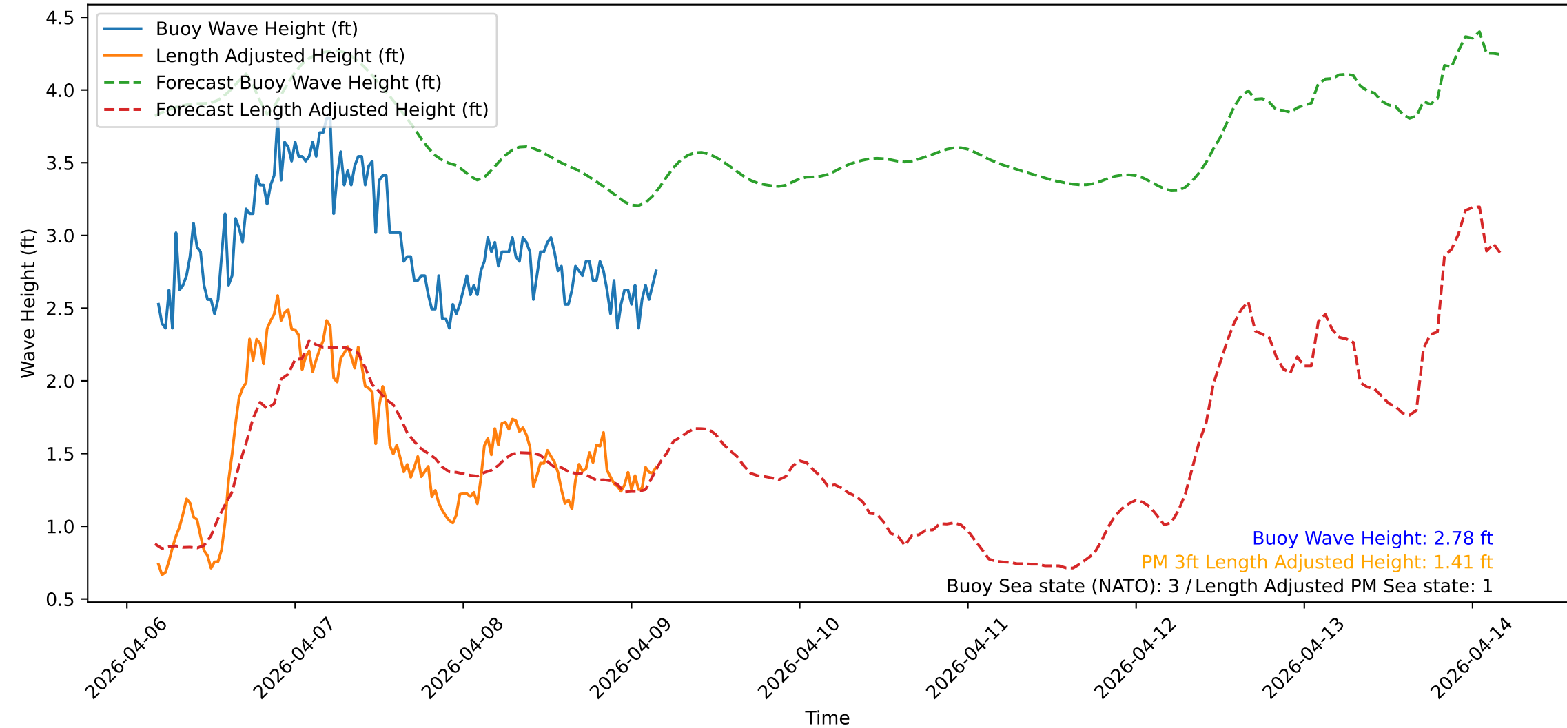
Wave Heights over Time for Green Beach at 2026-04-09 04:21:10
