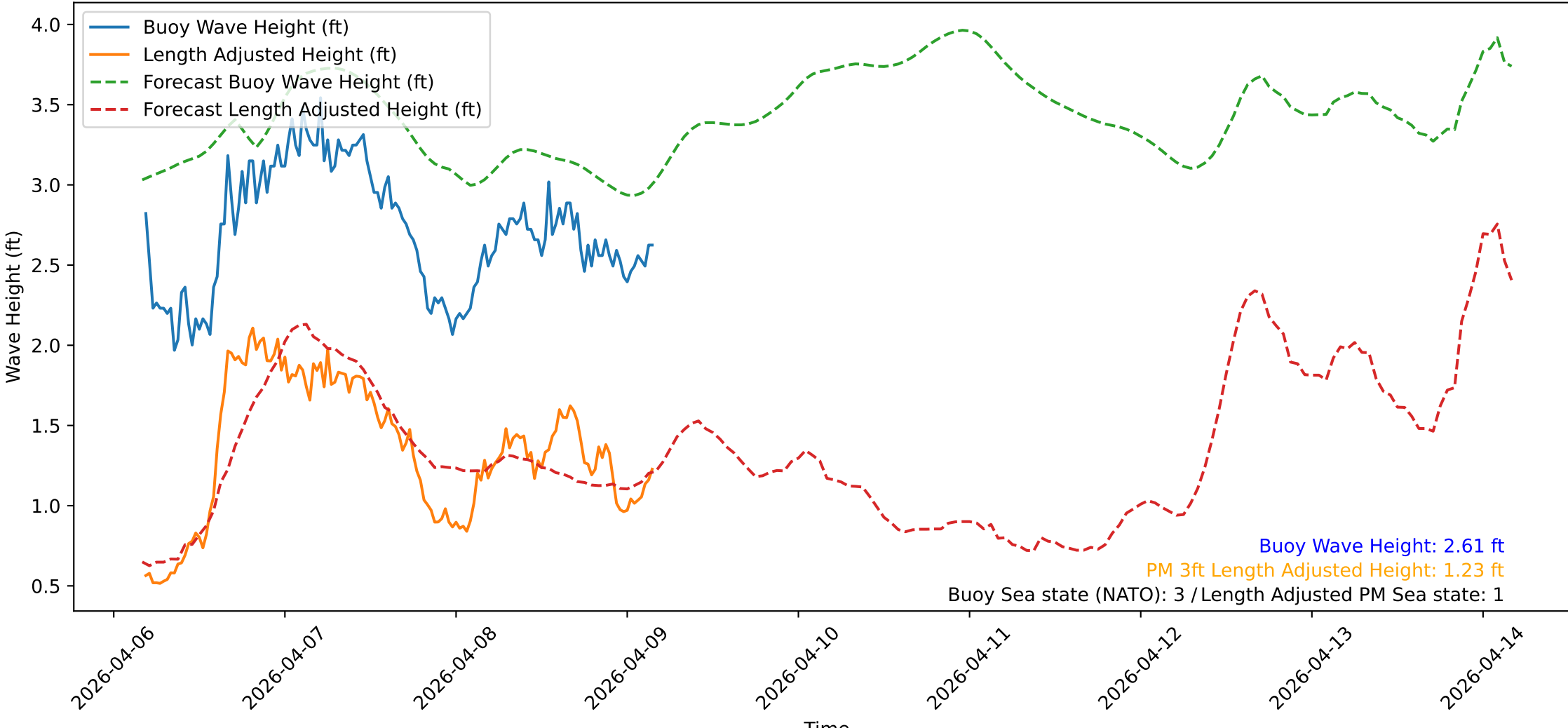
Wave Heights over Time for Red Beach at 2026-04-09 04:20:48
