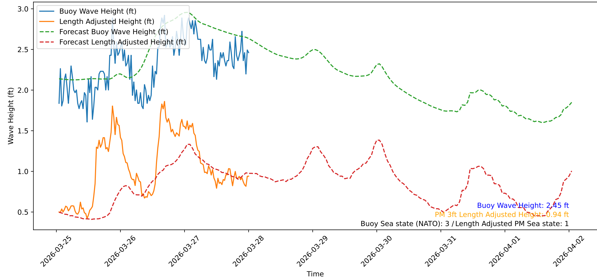
Wave Heights over Time for Oceanside Harbor at 2026-03-28 00:50:31
