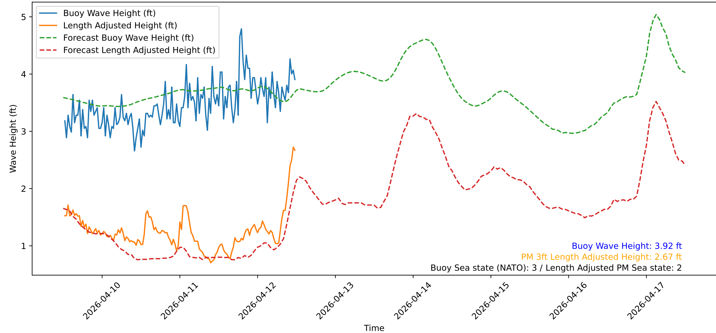
Wave Heights over Time for Oceanside Harbor at 2026-04-12 12:20:31
