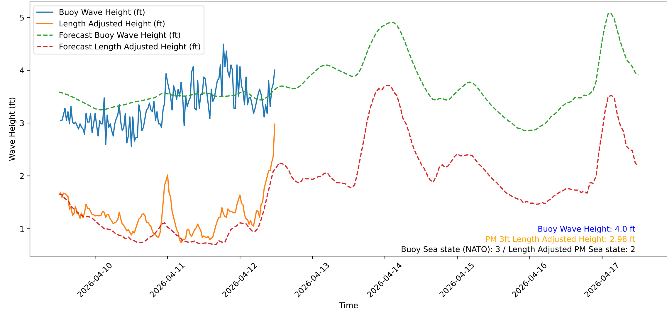
Wave Heights over Time for Green Beach at 2026-04-12 12:21:13
