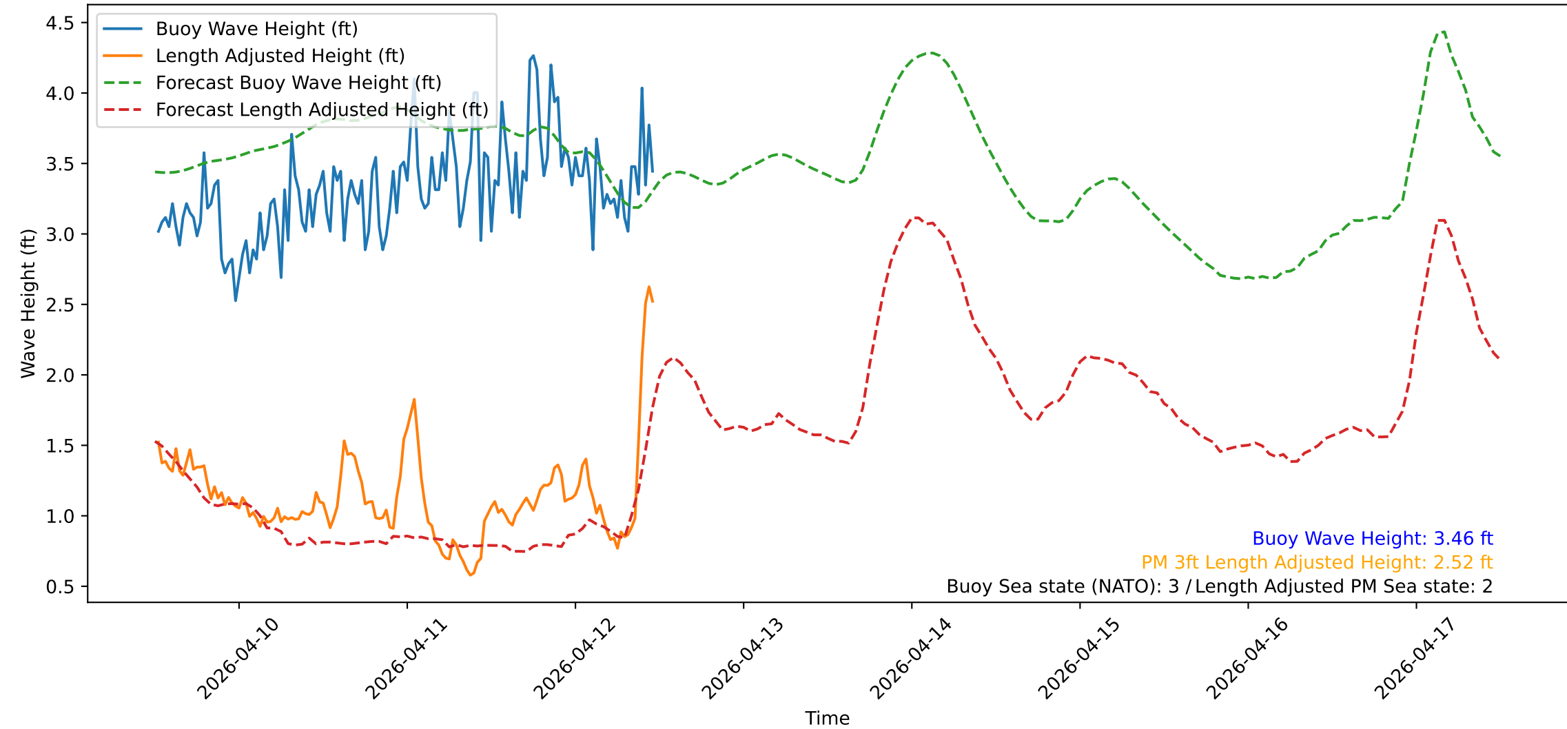
Wave Heights over Time for Red Beach at 2026-04-12 12:20:51
