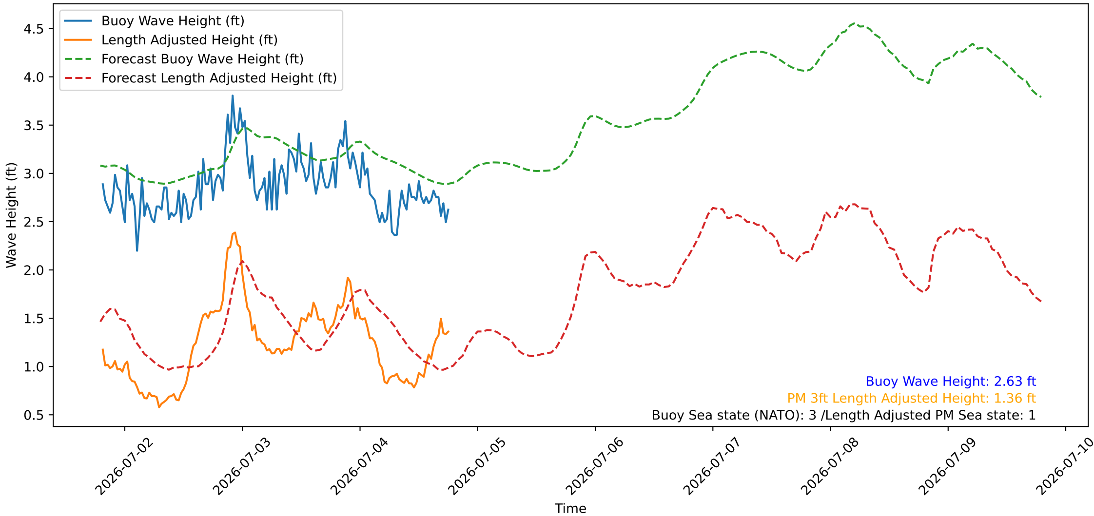
Wave Heights over Time for Red Beach at 2026-07-04 19:20:48
