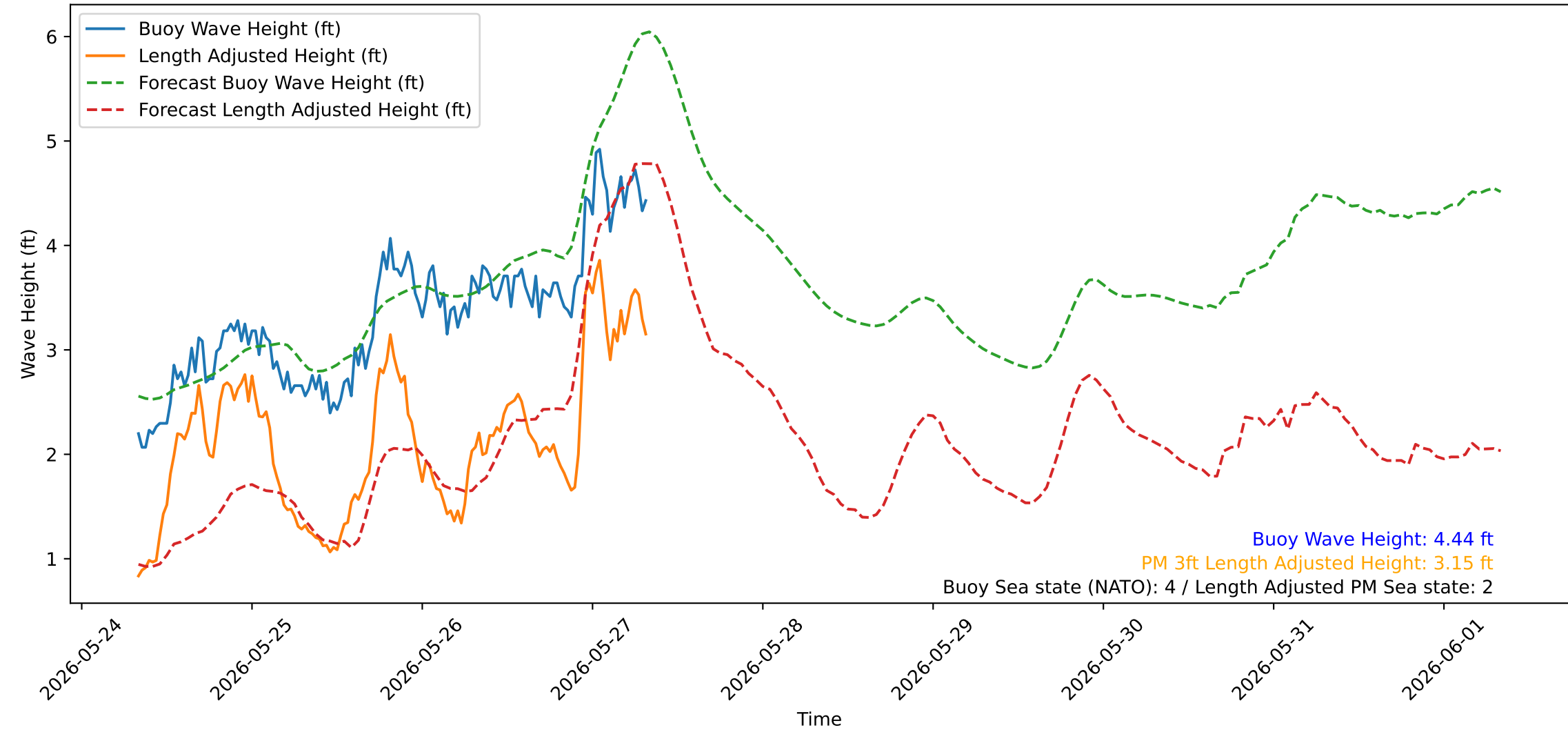
Wave Heights over Time for Green Beach at 2026-05-27 08:11:07
