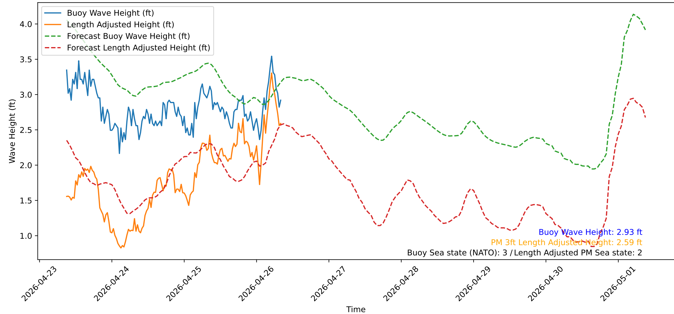
Wave Heights over Time for Red Beach at 2026-04-26 08:50:52
