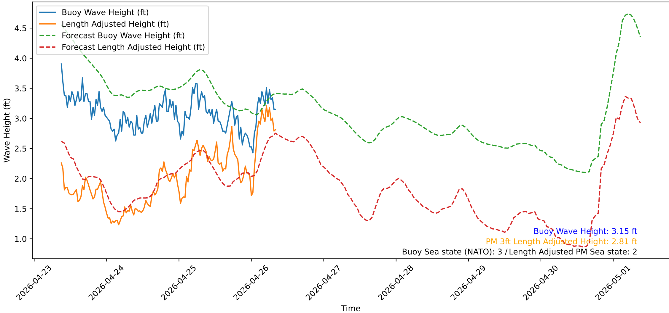
Wave Heights over Time for Green Beach at 2026-04-26 08:51:14
