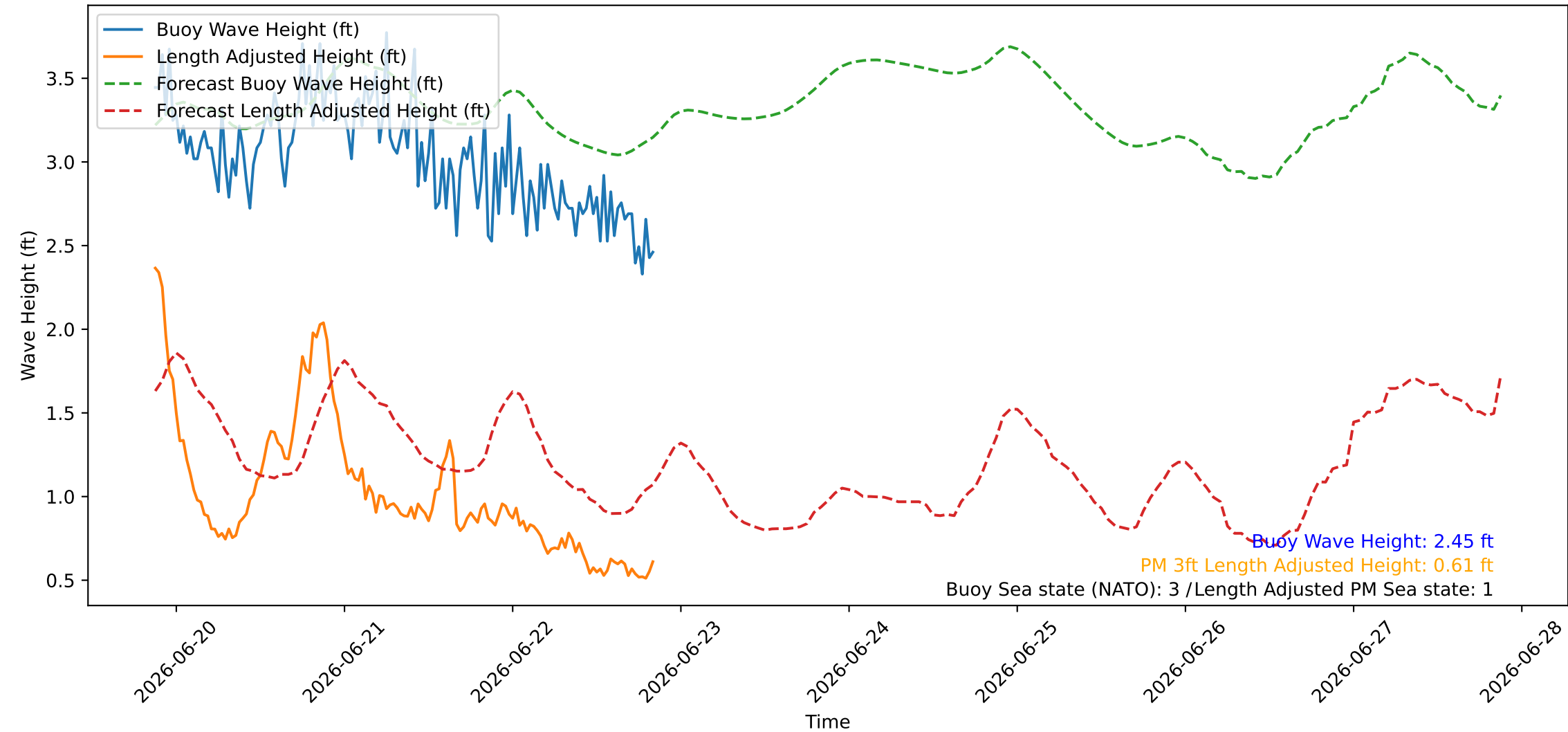
Wave Heights over Time for Red Beach at 2026-06-22 20:50:47
