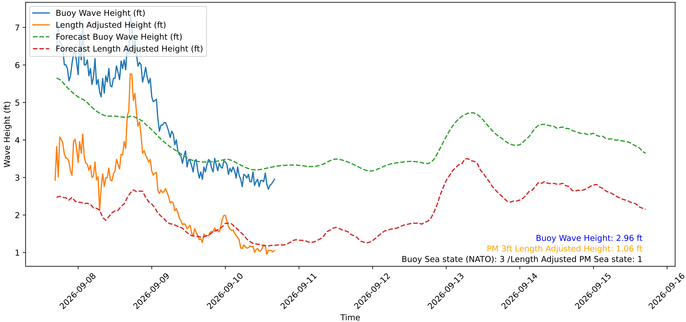
Wave Heights over Time for Oceanside Harbor at 2026-09-10 16:40:29
