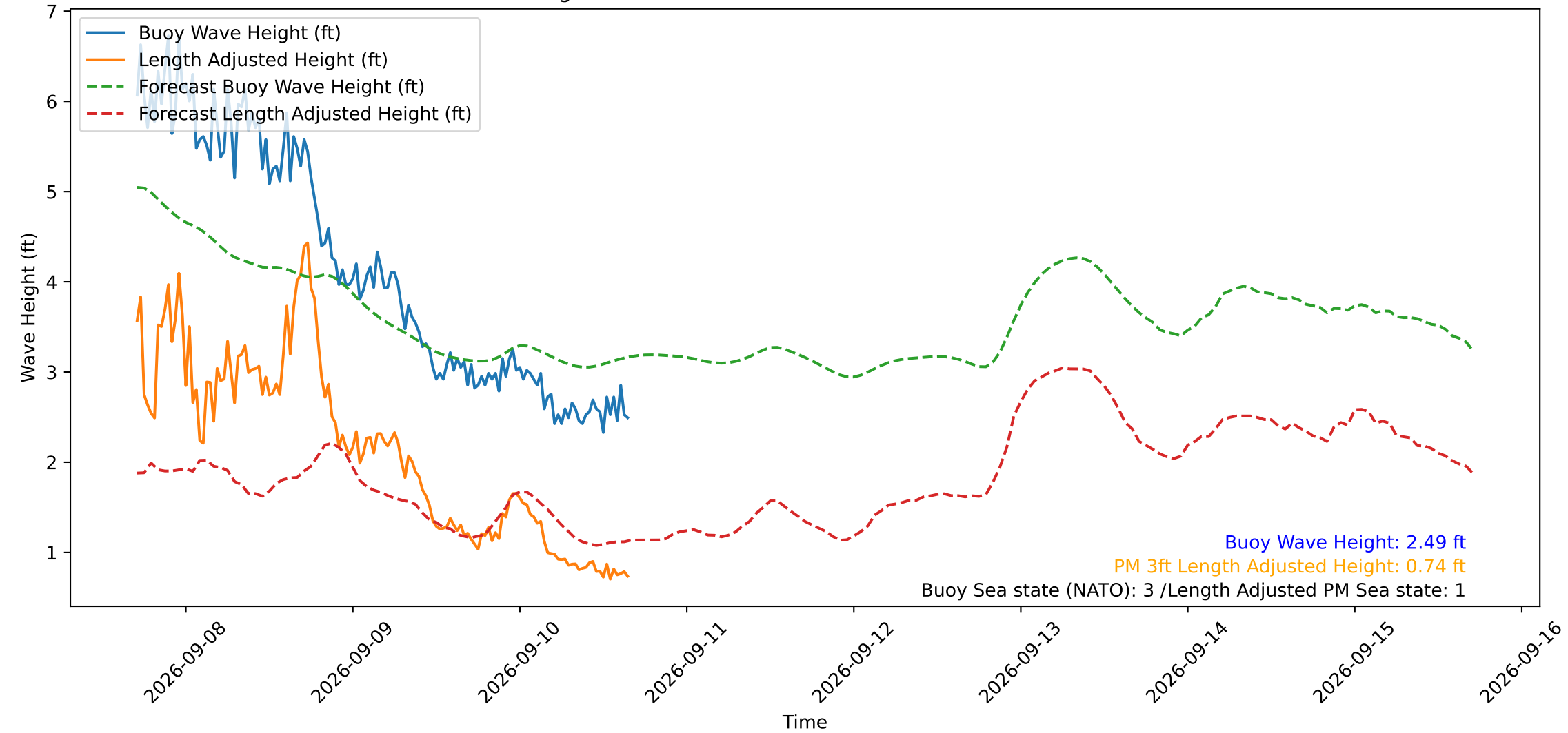
Wave Heights over Time for Red Beach at 2026-09-10 16:40:48
