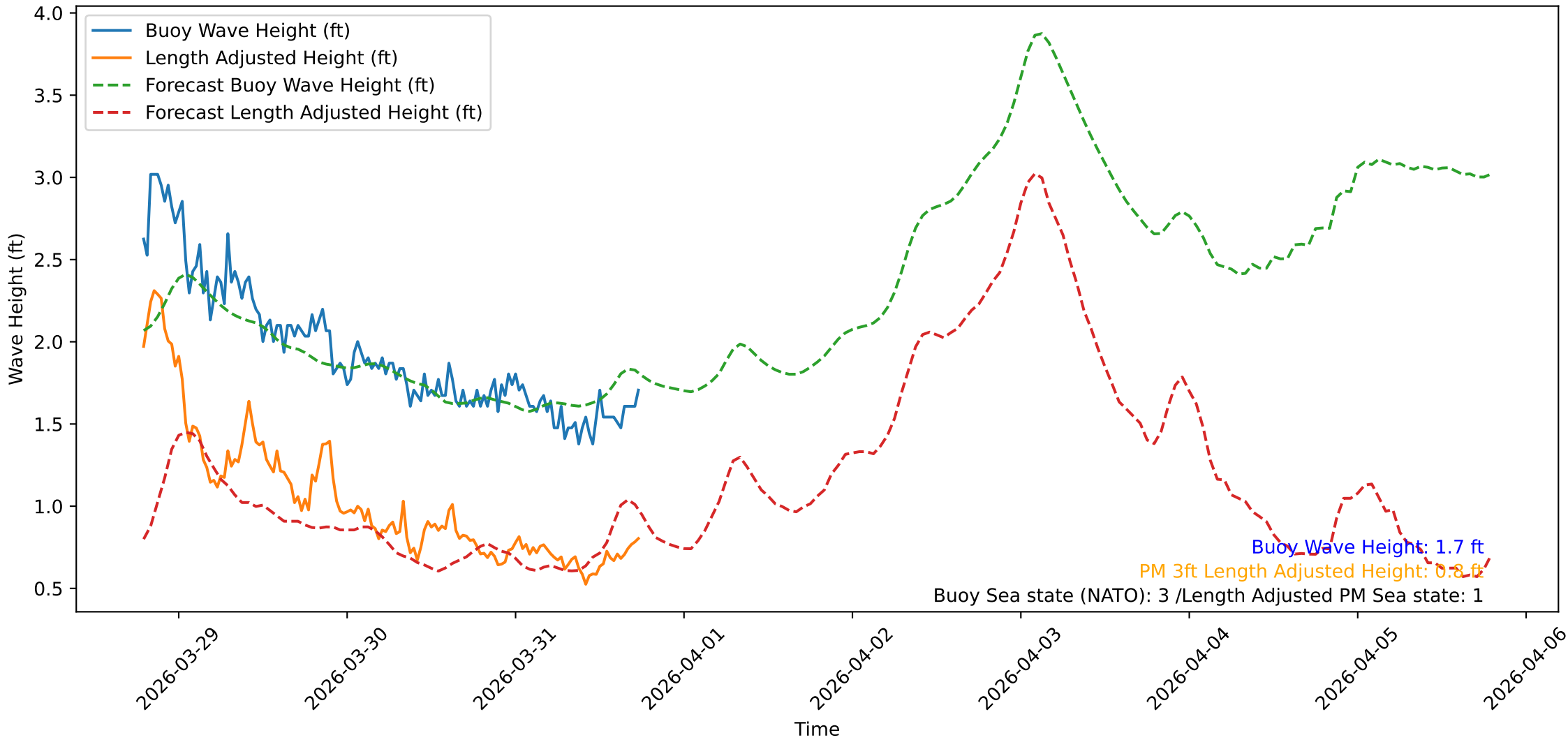
Wave Heights over Time for Red Beach at 2026-03-31 18:30:47
