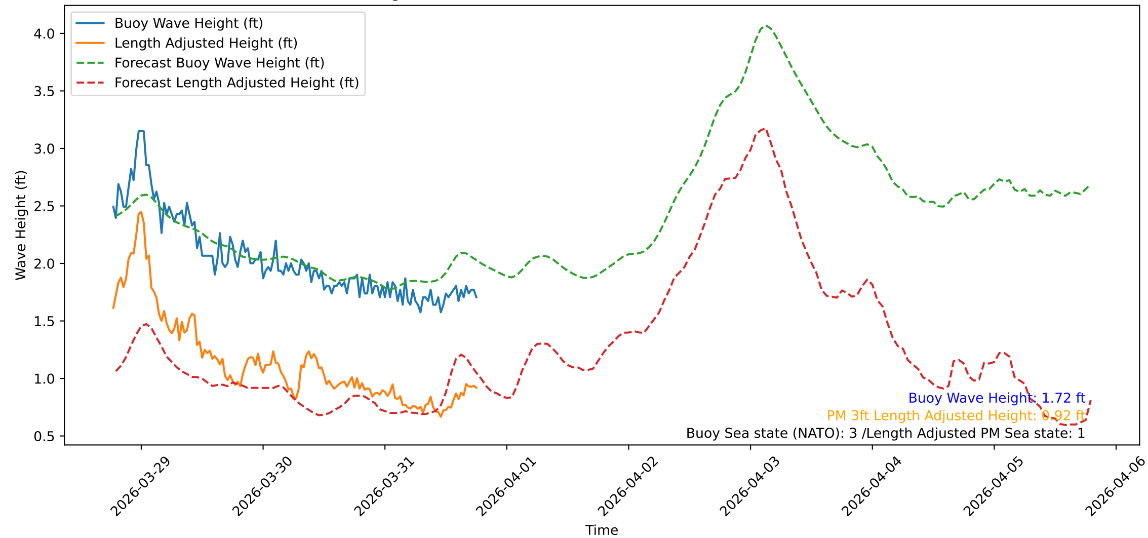
Wave Heights over Time for Oceanside Harbor at 2026-03-31 18:30:31
