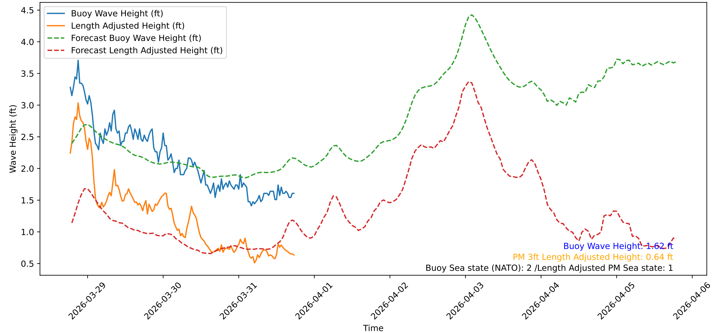
Wave Heights over Time for Green Beach at 2026-03-31 18:31:10
