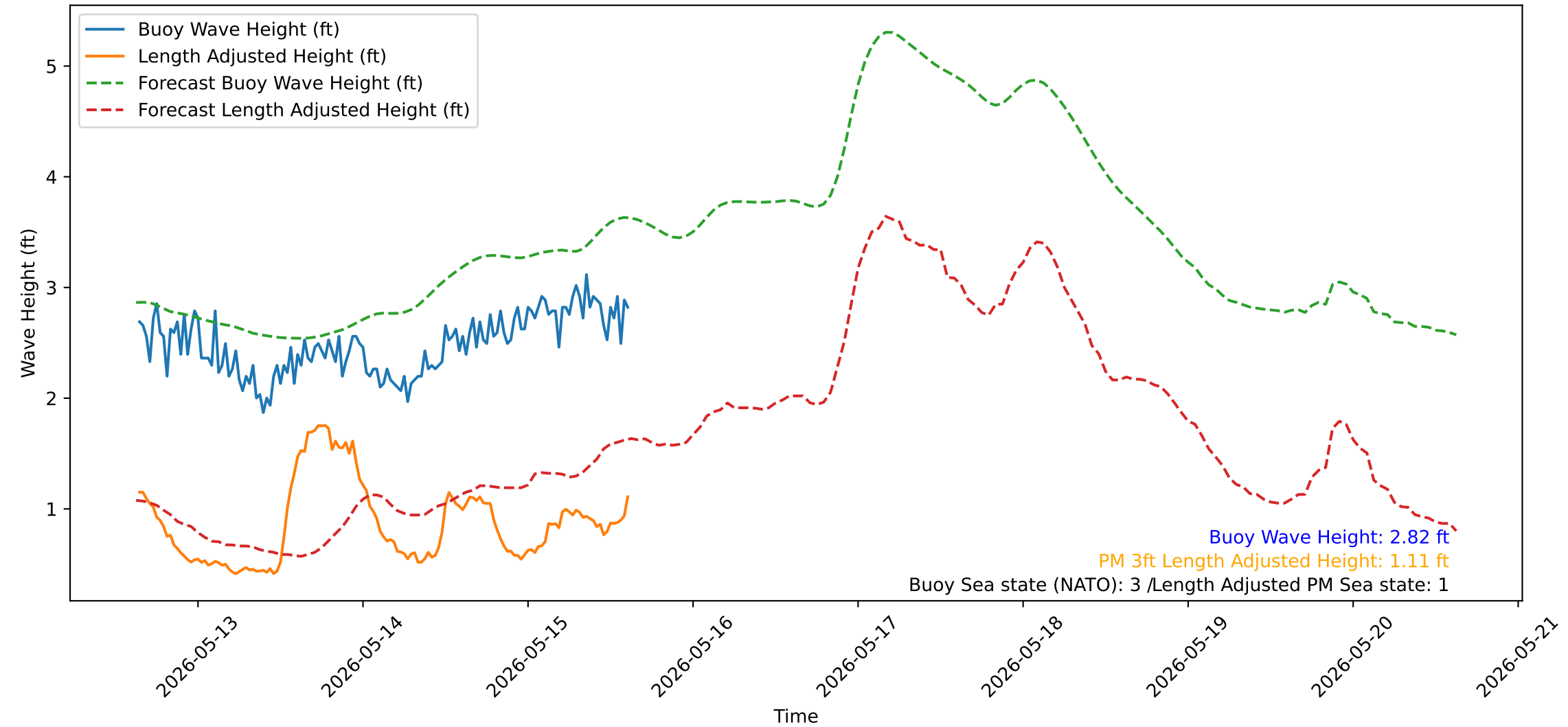
Wave Heights over Time for Red Beach at 2026-05-15 15:20:54
