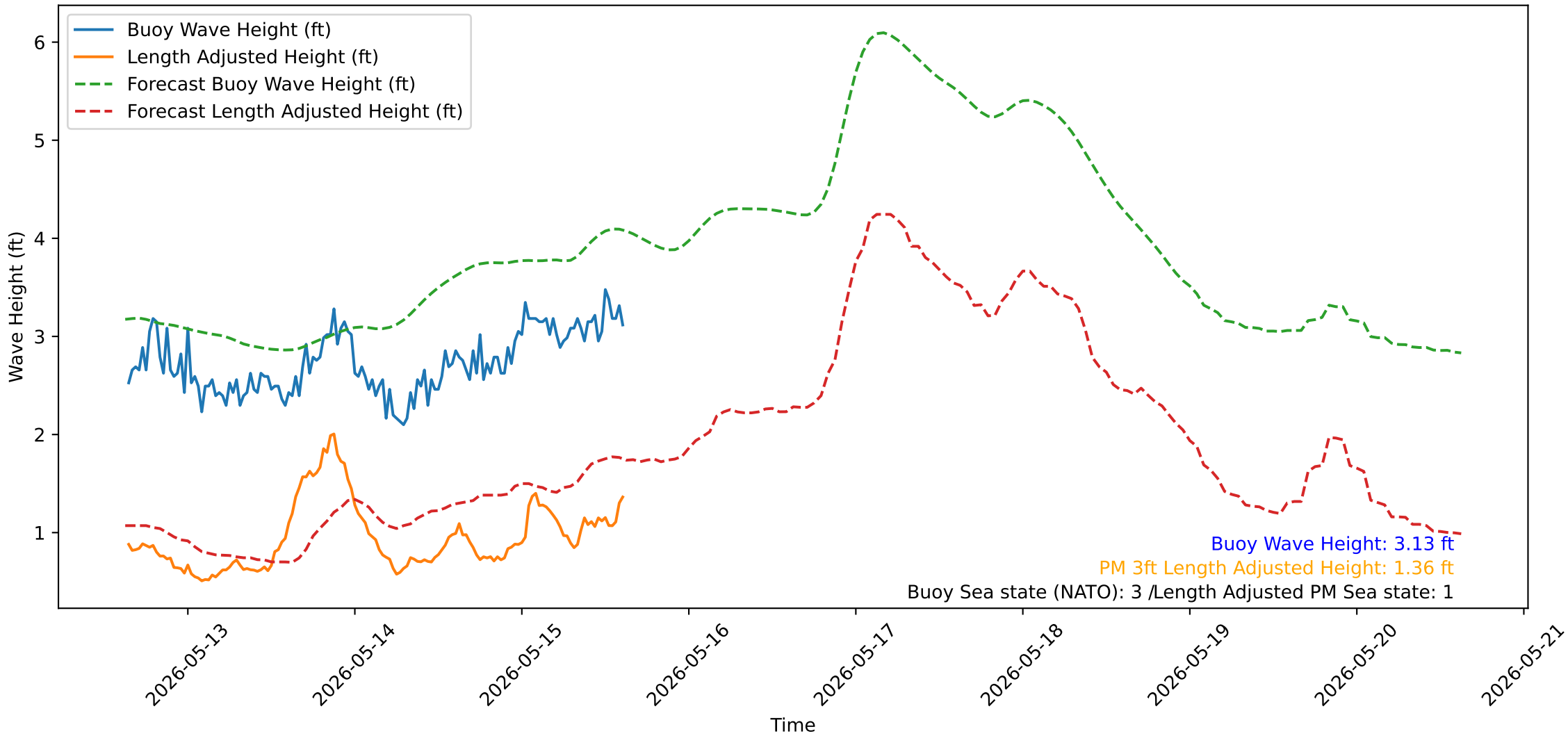
Wave Heights over Time for Green Beach at 2026-05-15 15:21:16
