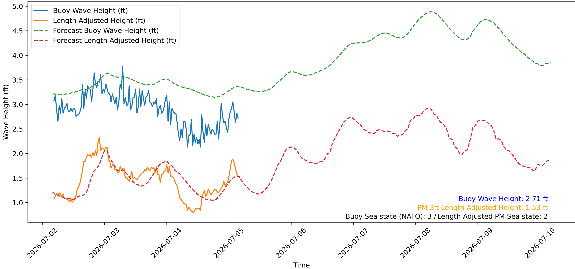
Wave Heights over Time for Oceanside Harbor at 2026-07-05 04:20:26
