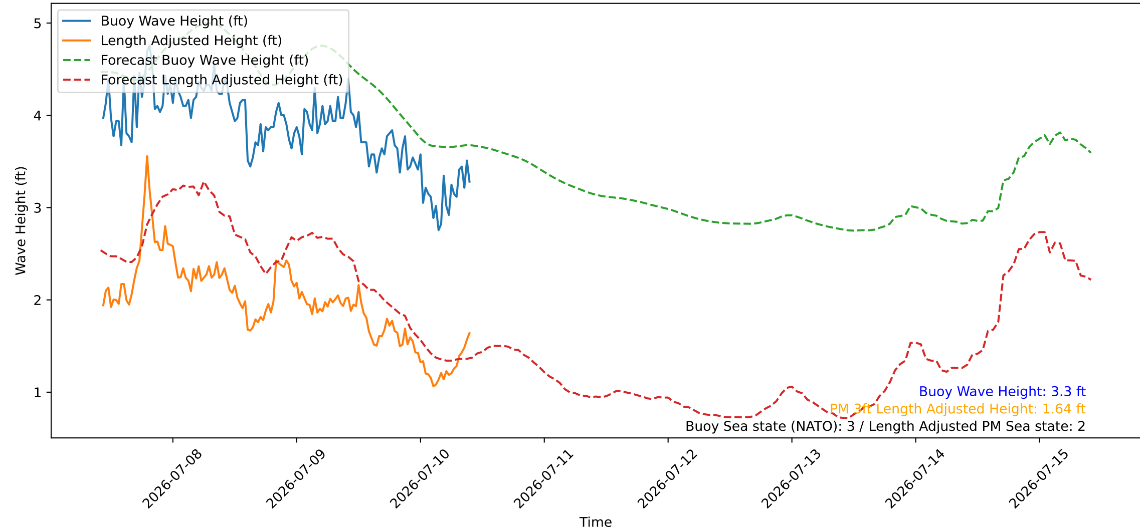
Wave Heights over Time for Green Beach at 2026-07-10 10:21:08
