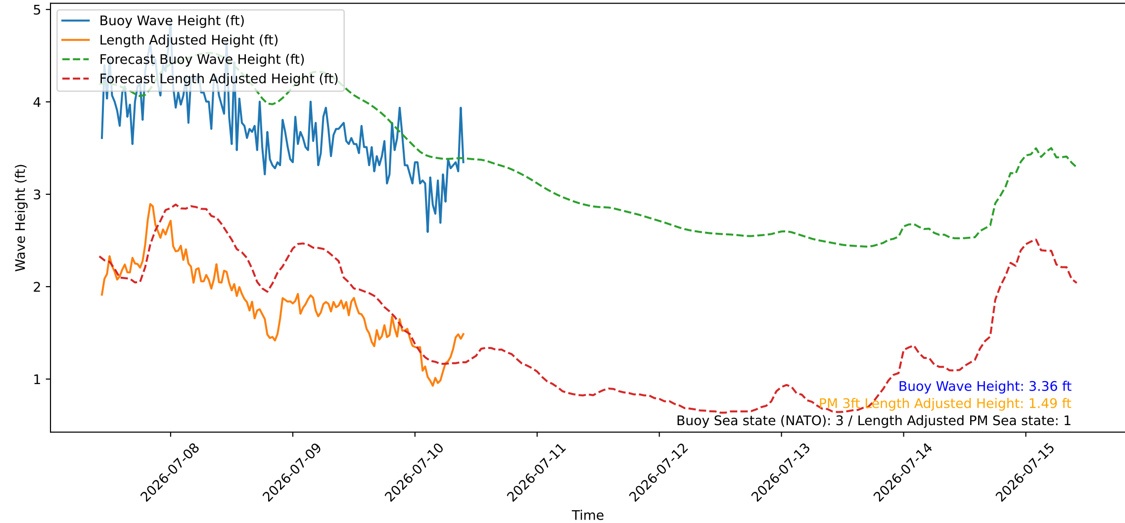
Wave Heights over Time for Red Beach at 2026-07-10 10:20:46
