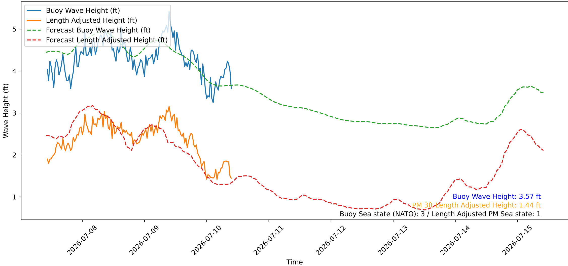
Wave Heights over Time for Oceanside Harbor at 2026-07-10 10:20:25
