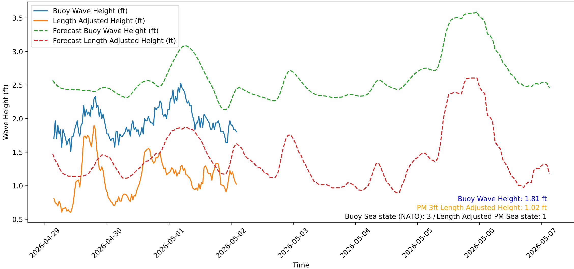
Wave Heights over Time for Red Beach at 2026-05-02 03:00:51
