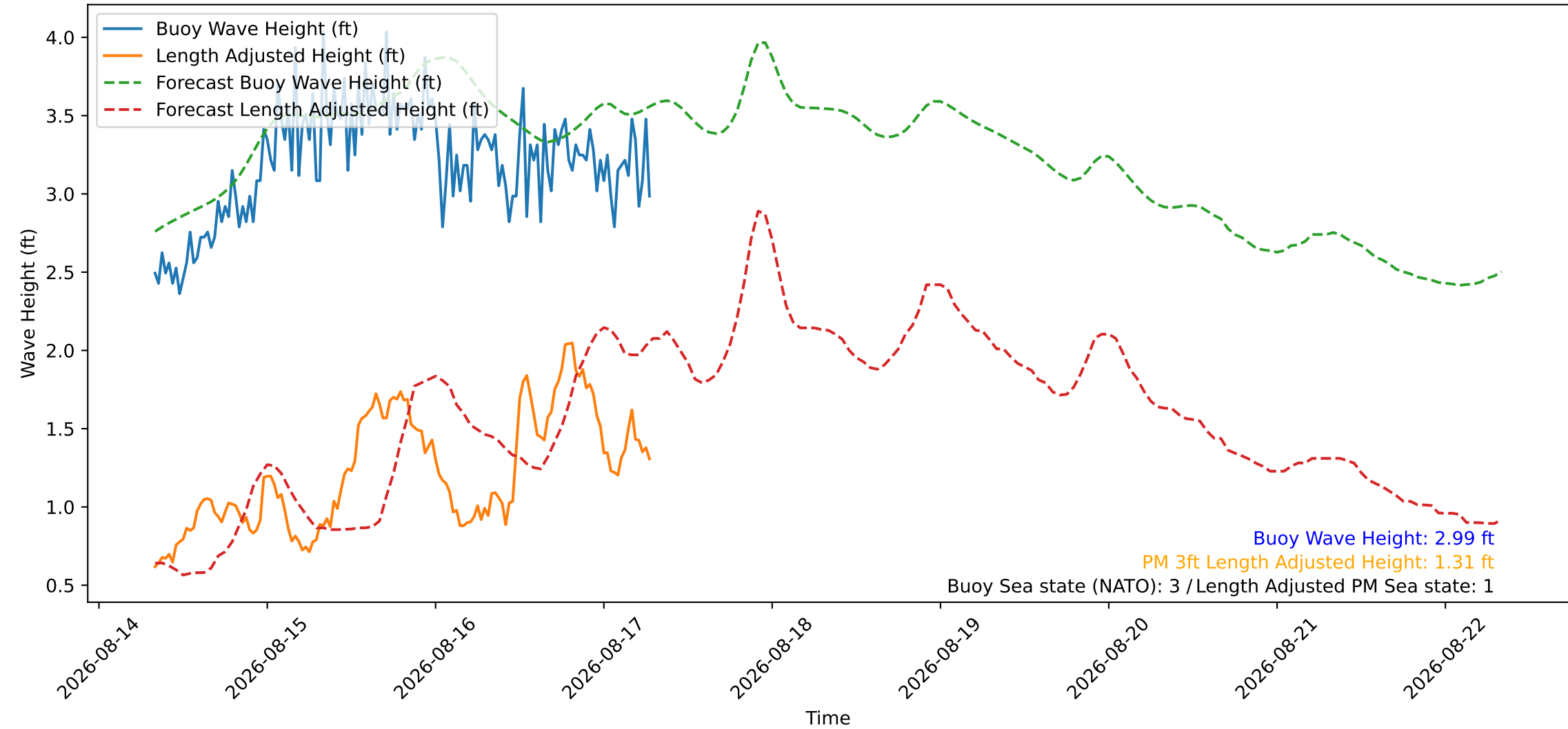
Wave Heights over Time for Red Beach at 2026-08-17 07:30:46
