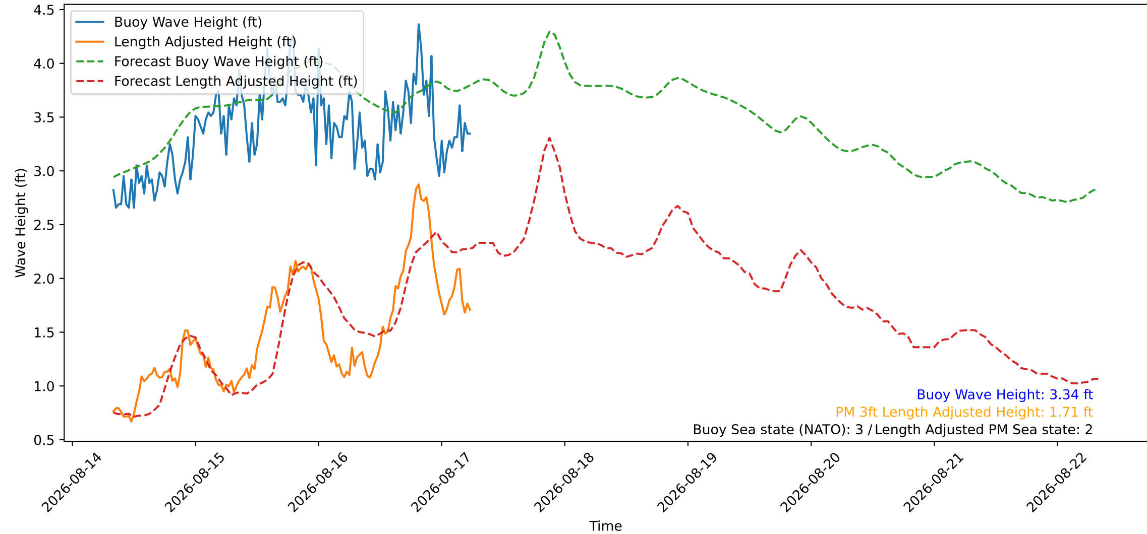
Wave Heights over Time for Green Beach at 2026-08-17 07:31:08
