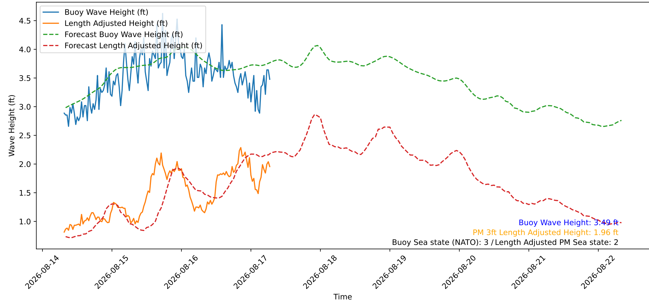
Wave Heights over Time for Oceanside Harbor at 2026-08-17 07:30:26
