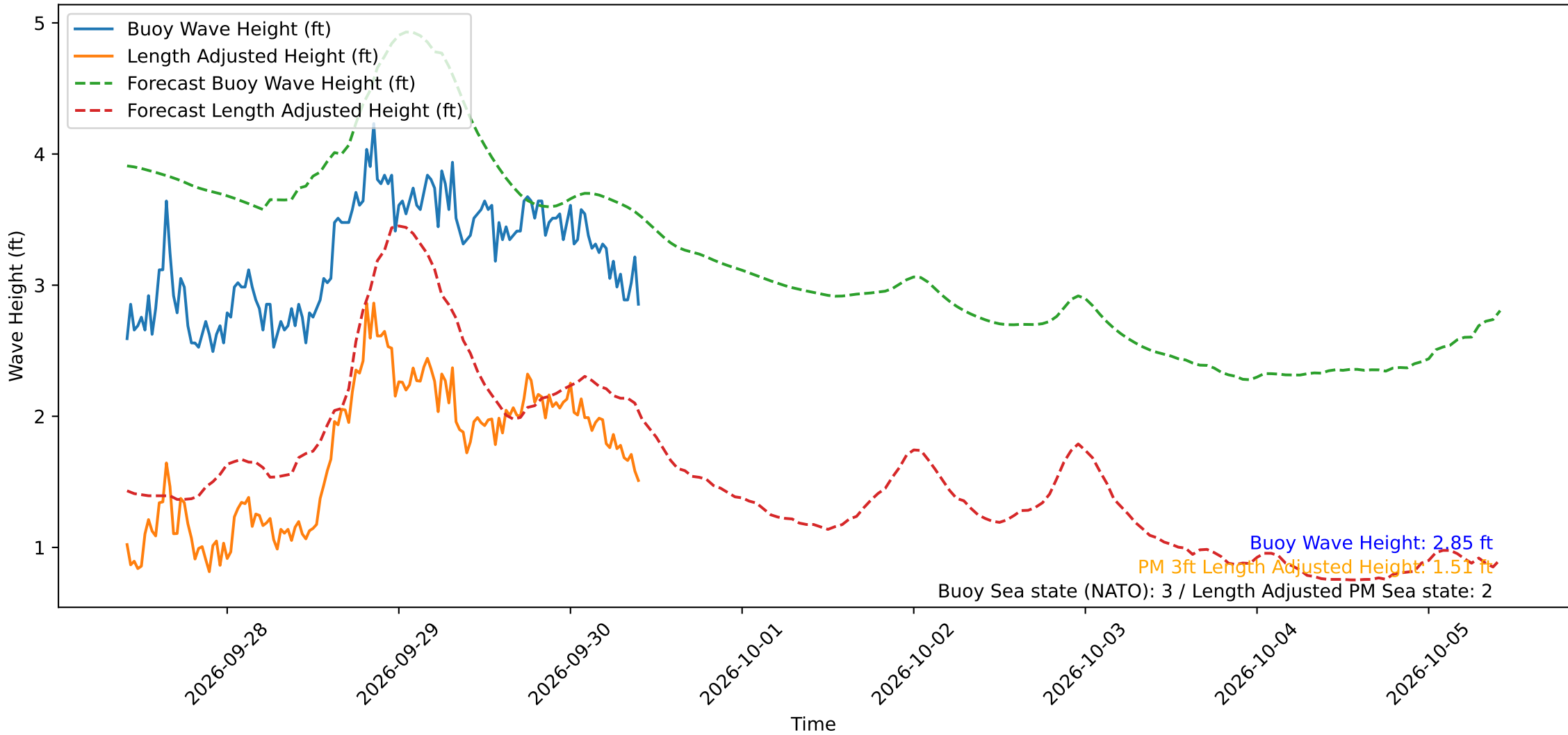
Wave Heights over Time for Oceanside Harbor at 2026-09-30 10:00:30
