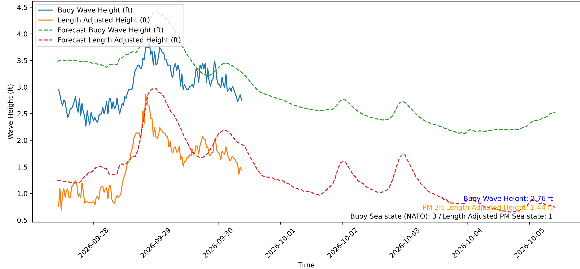
Wave Heights over Time for Red Beach at 2026-09-30 10:00:49
