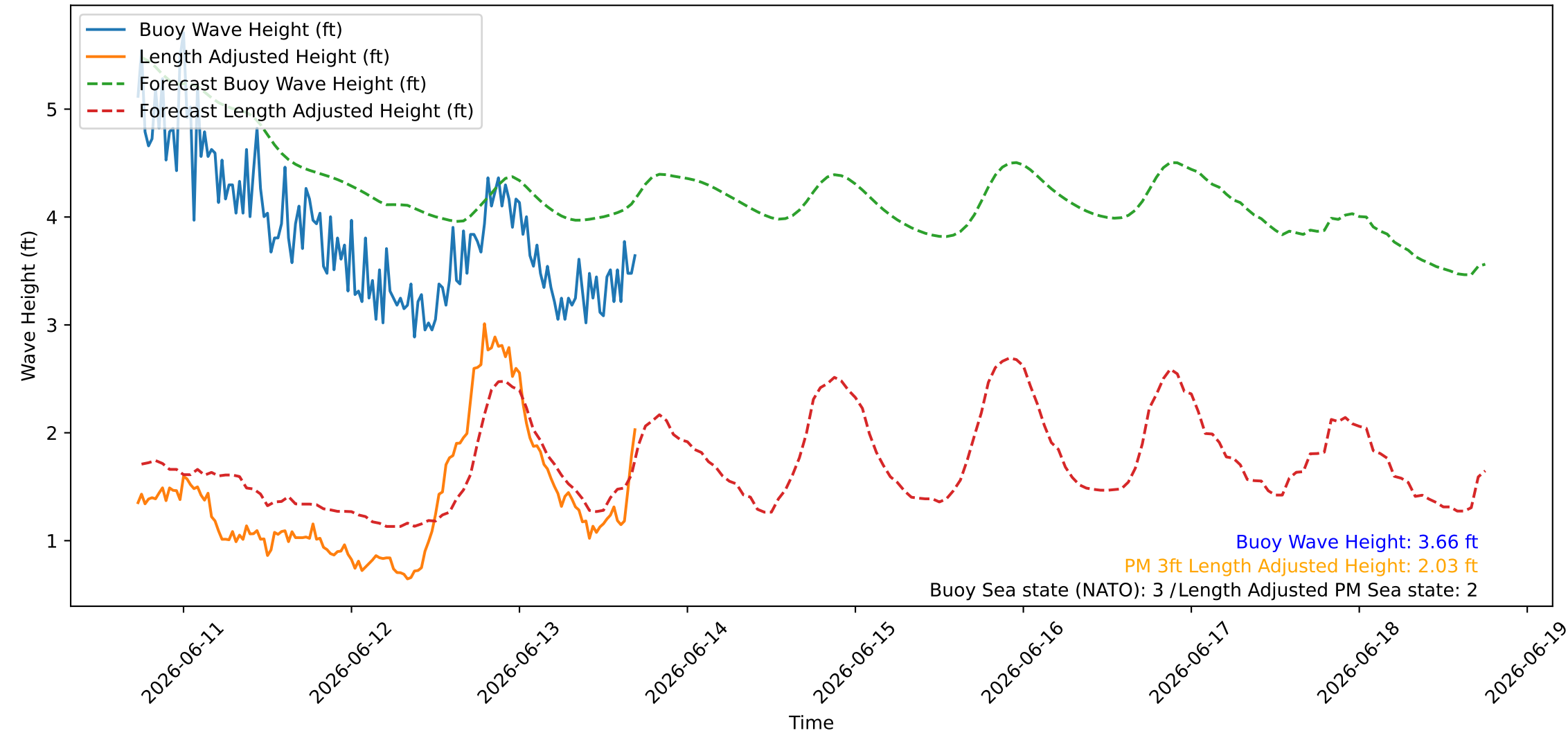
Wave Heights over Time for Green Beach at 2026-06-13 17:31:07
