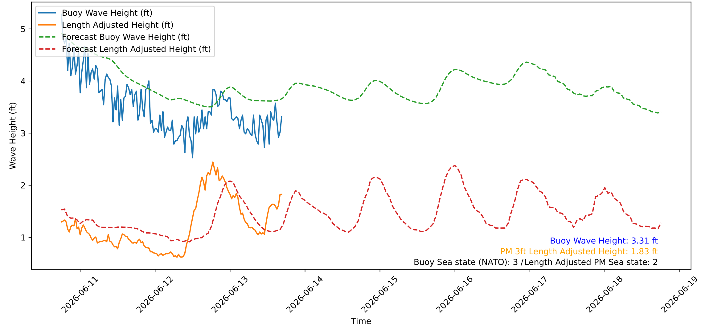
Wave Heights over Time for Red Beach at 2026-06-13 17:30:45
