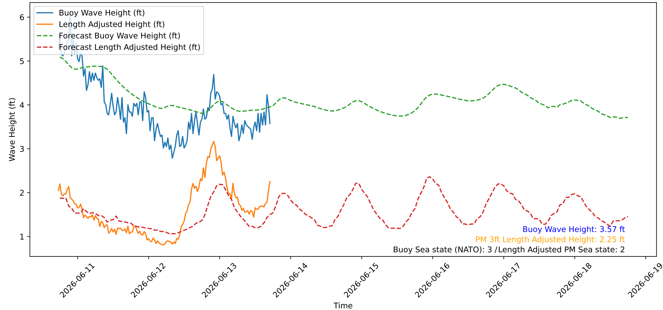
Wave Heights over Time for Oceanside Harbor at 2026-06-13 17:30:26
