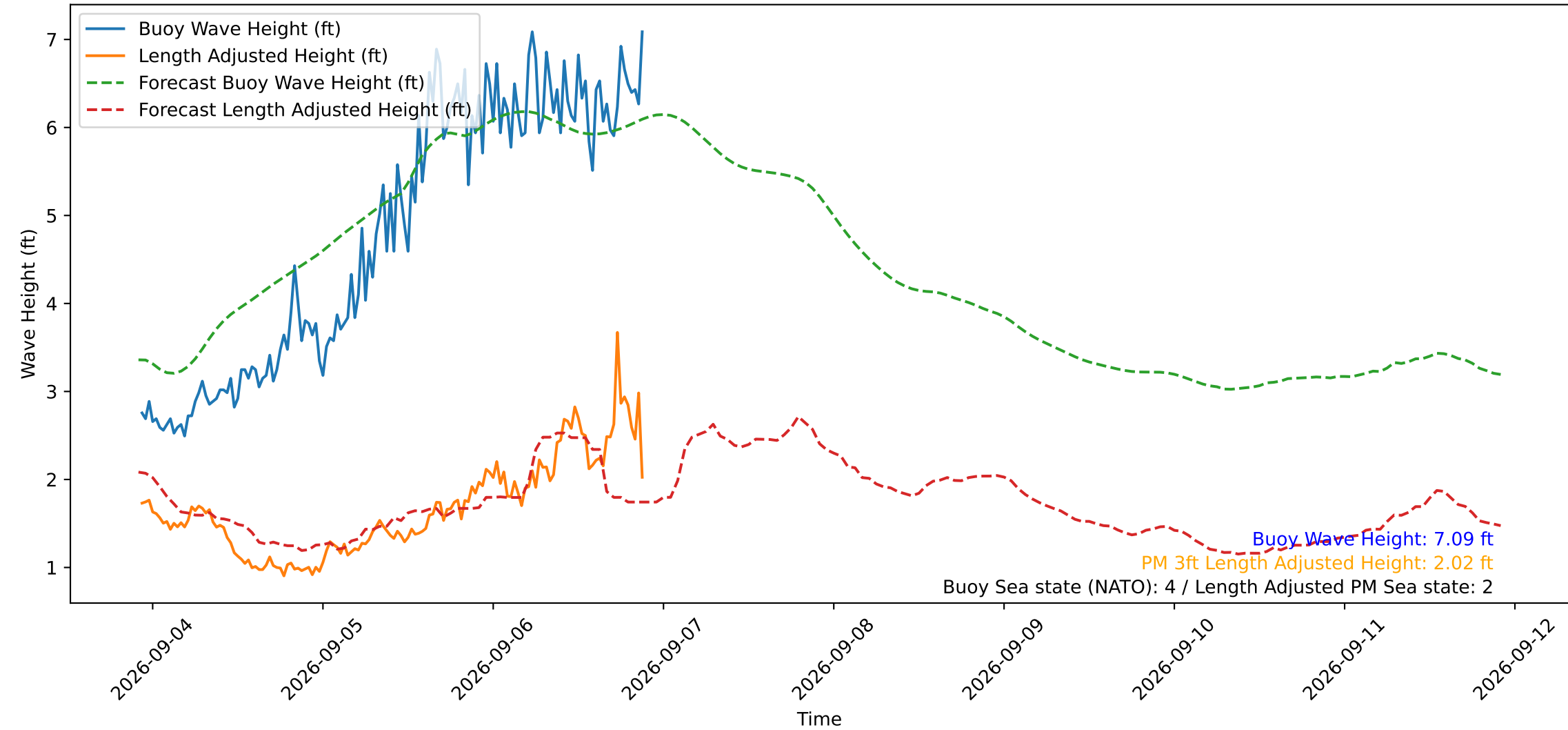
Wave Heights over Time for Green Beach at 2026-09-06 22:01:13
