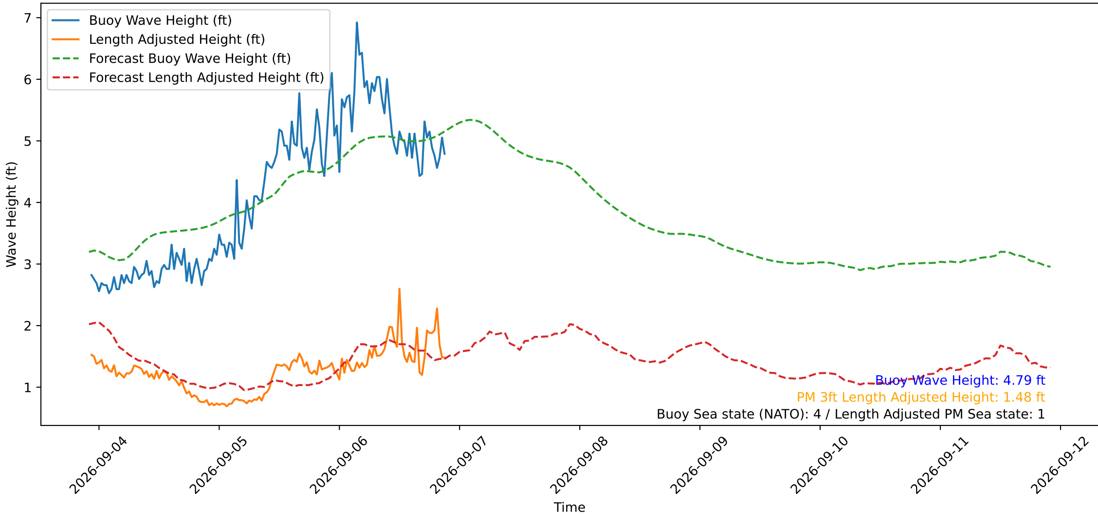
Wave Heights over Time for Red Beach at 2026-09-06 22:00:50
