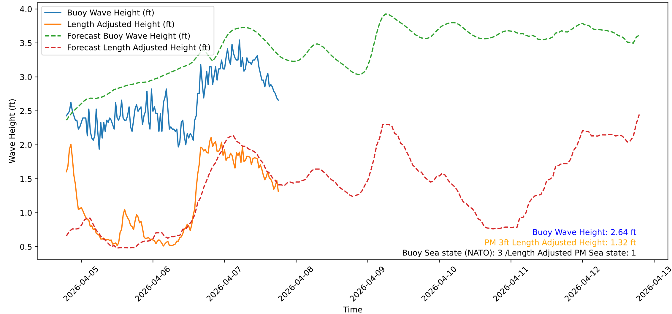
Wave Heights over Time for Red Beach at 2026-04-07 18:50:47
