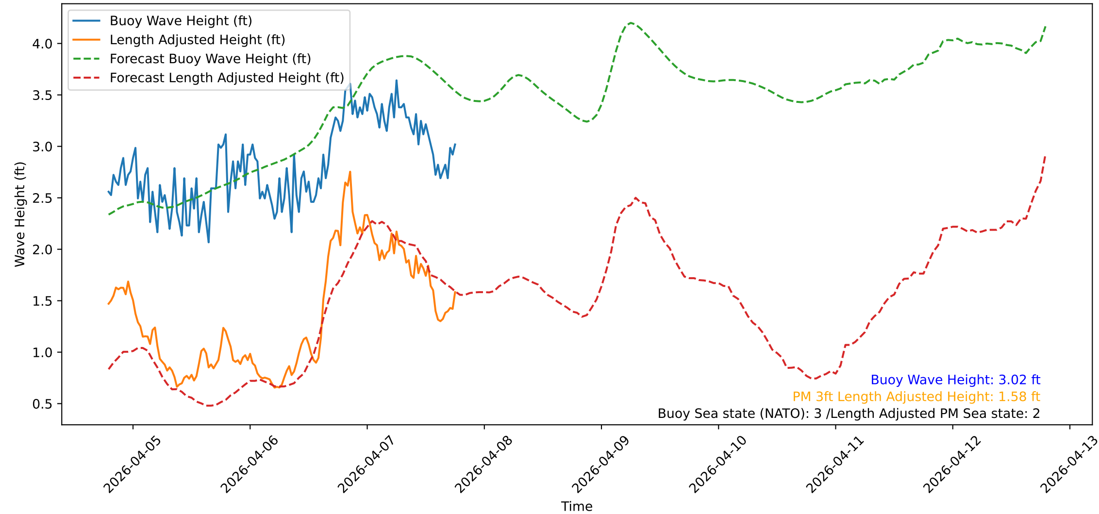
Wave Heights over Time for Oceanside Harbor at 2026-04-07 18:50:31
