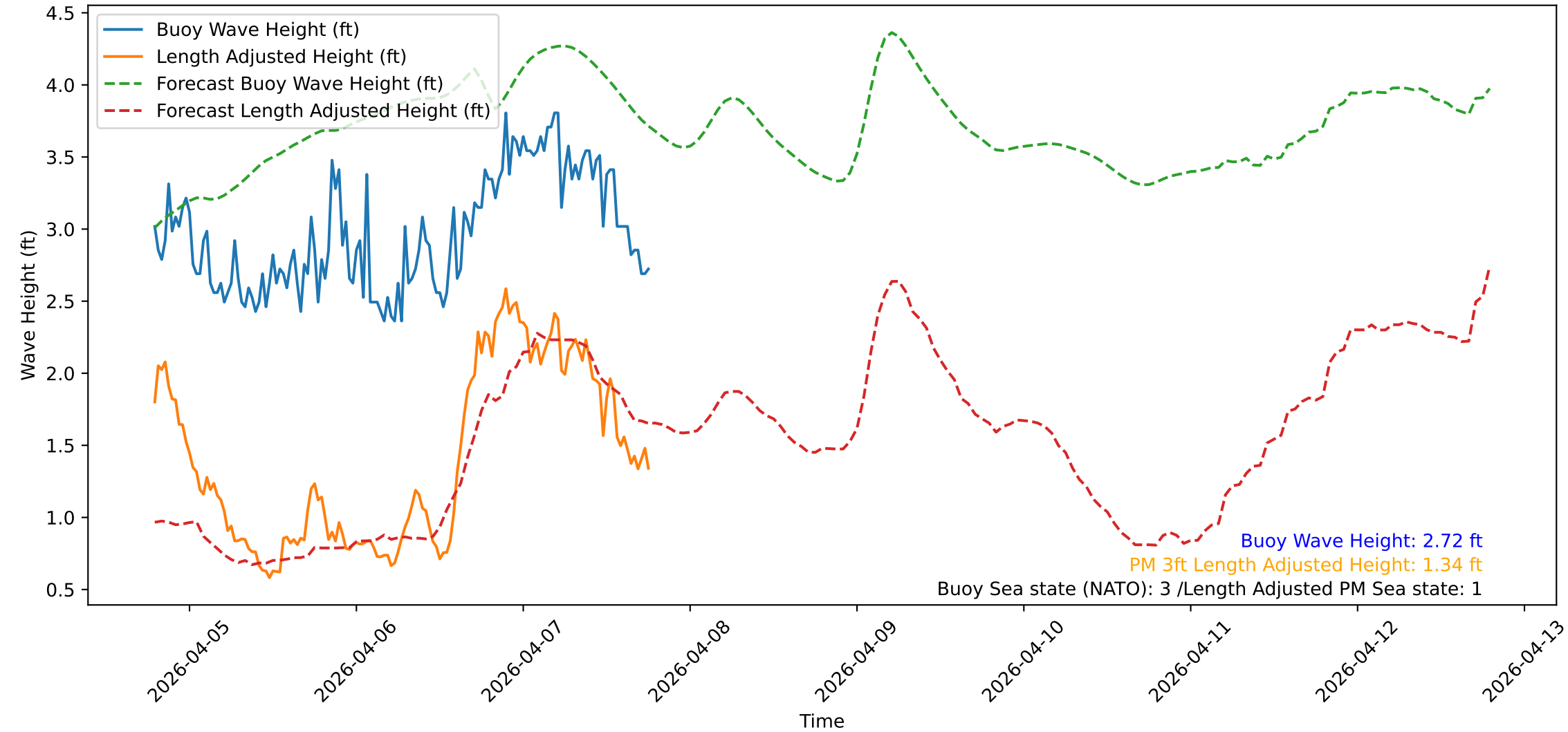
Wave Heights over Time for Green Beach at 2026-04-07 18:51:10
