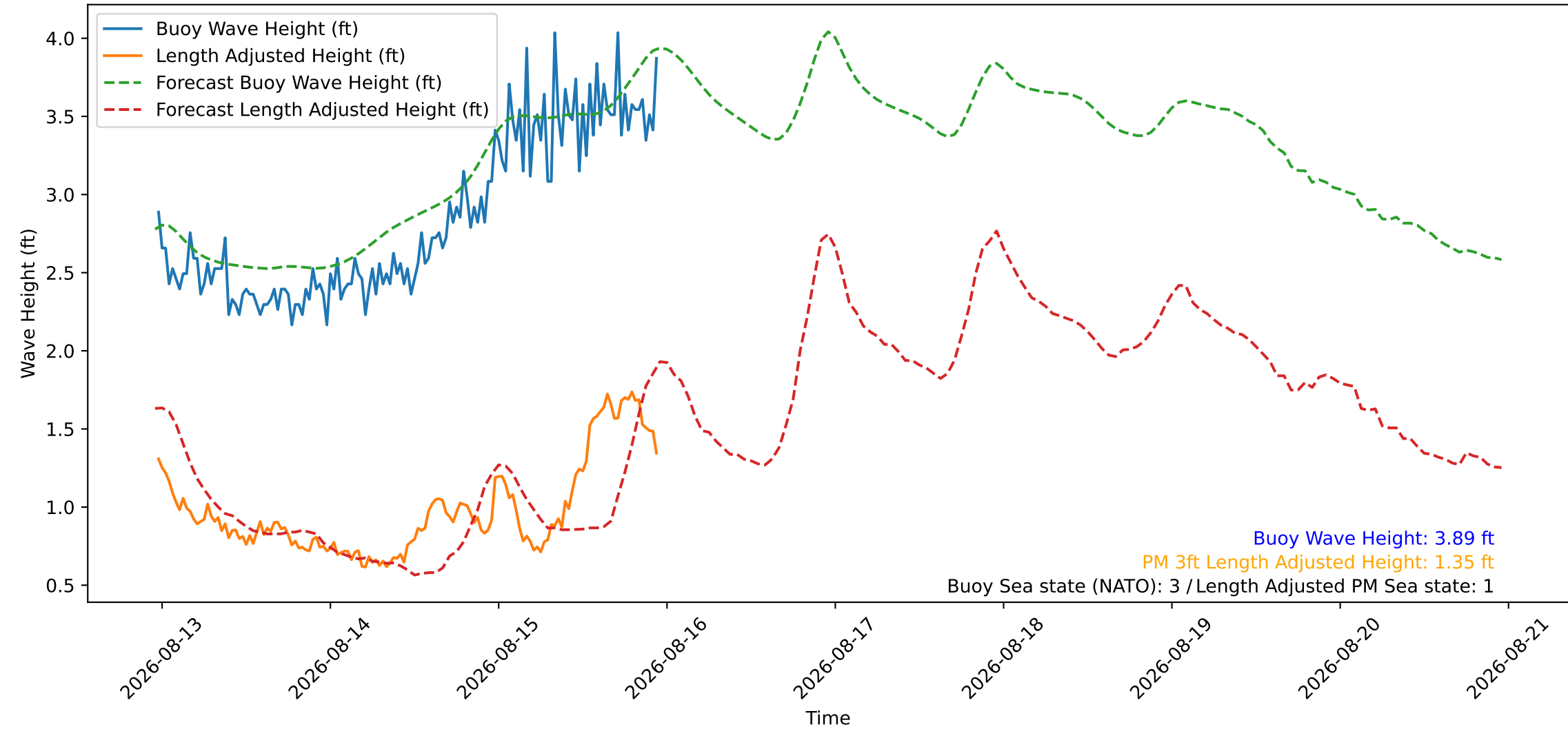
Wave Heights over Time for Red Beach at 2026-08-15 23:10:46
