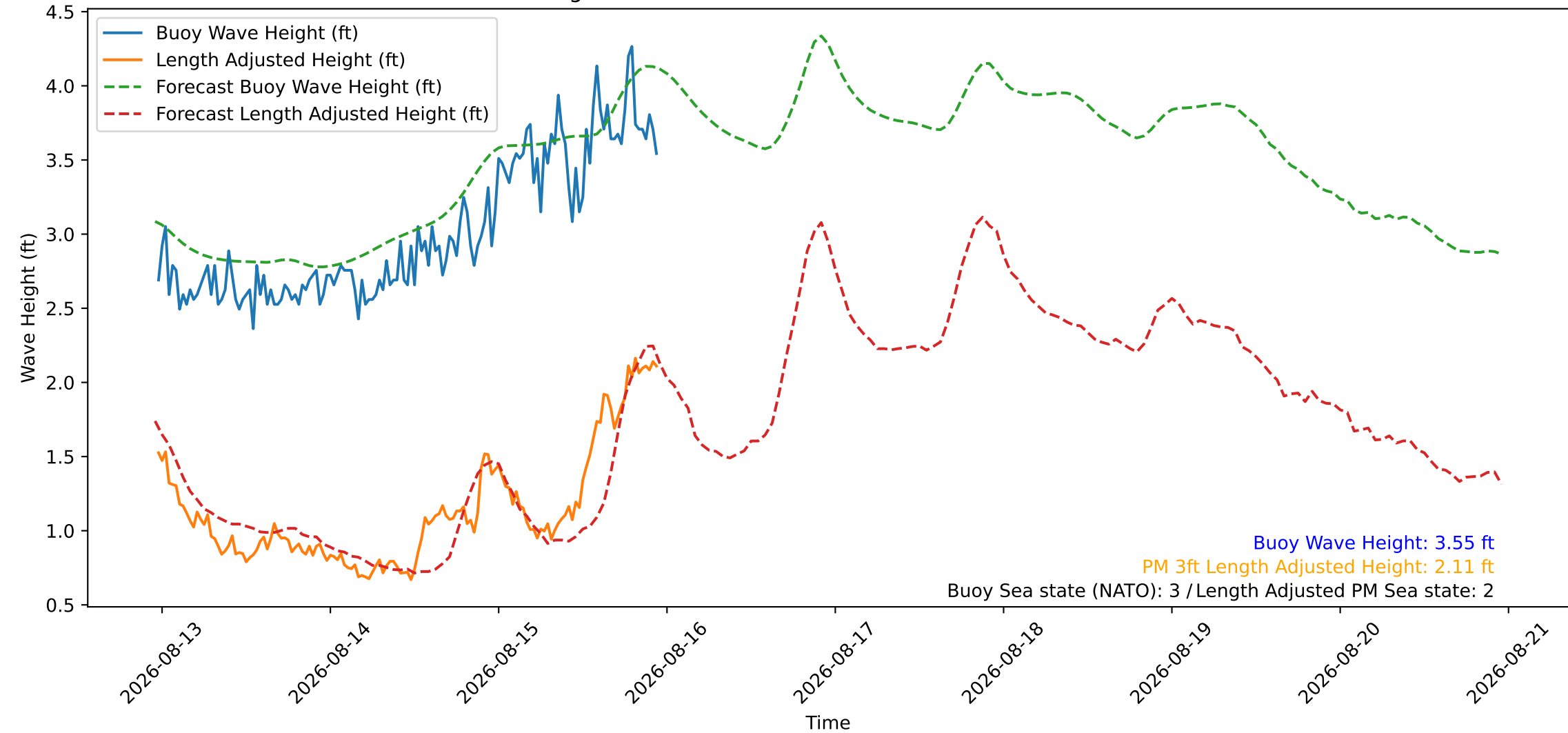
Wave Heights over Time for Green Beach at 2026-08-15 23:11:08
