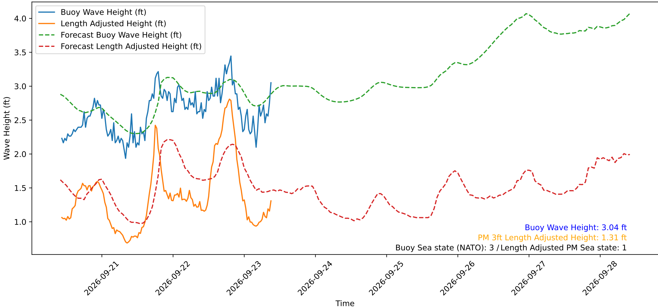
Wave Heights over Time for Green Beach at 2026-09-23 10:01:11
