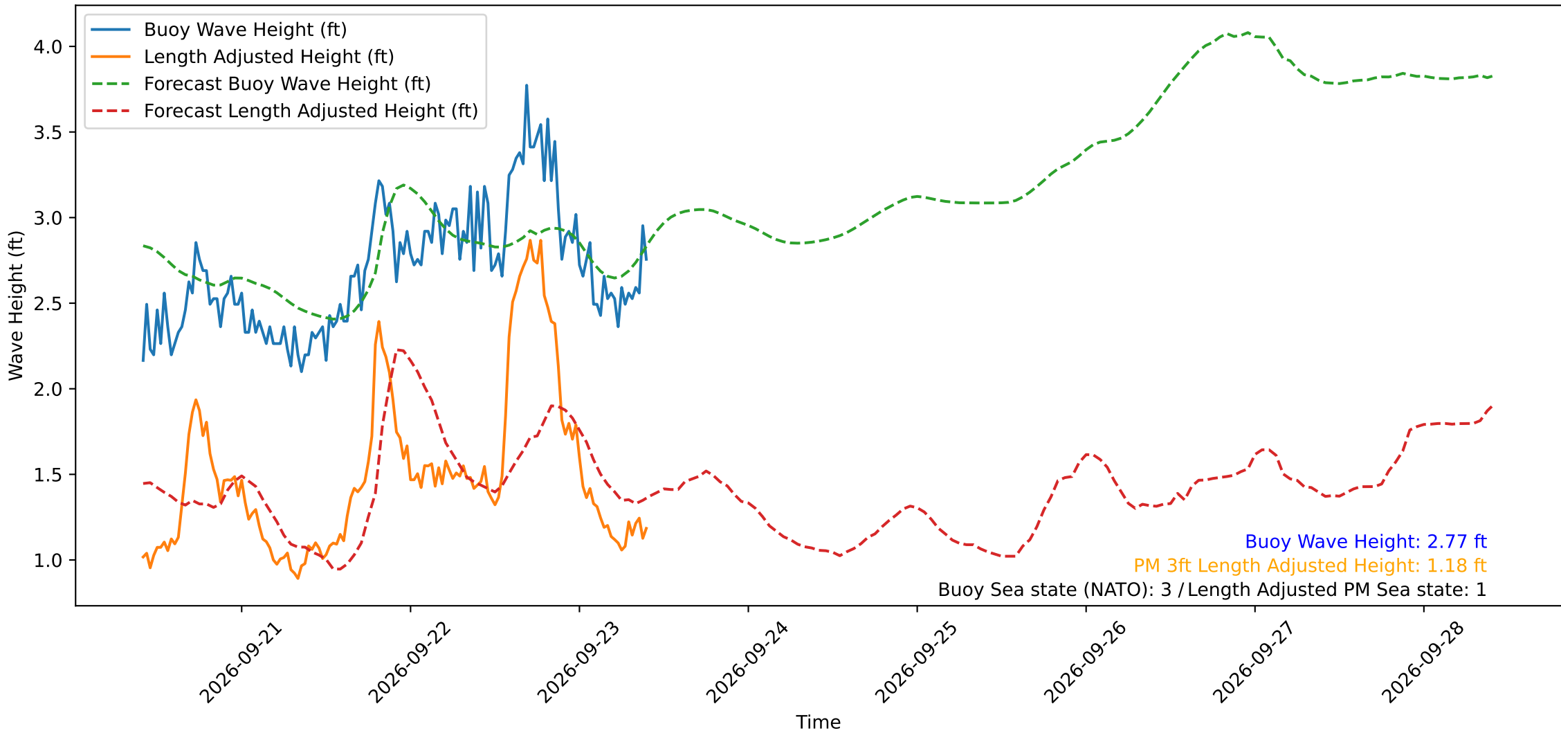
Wave Heights over Time for Oceanside Harbor at 2026-09-23 10:00:29
