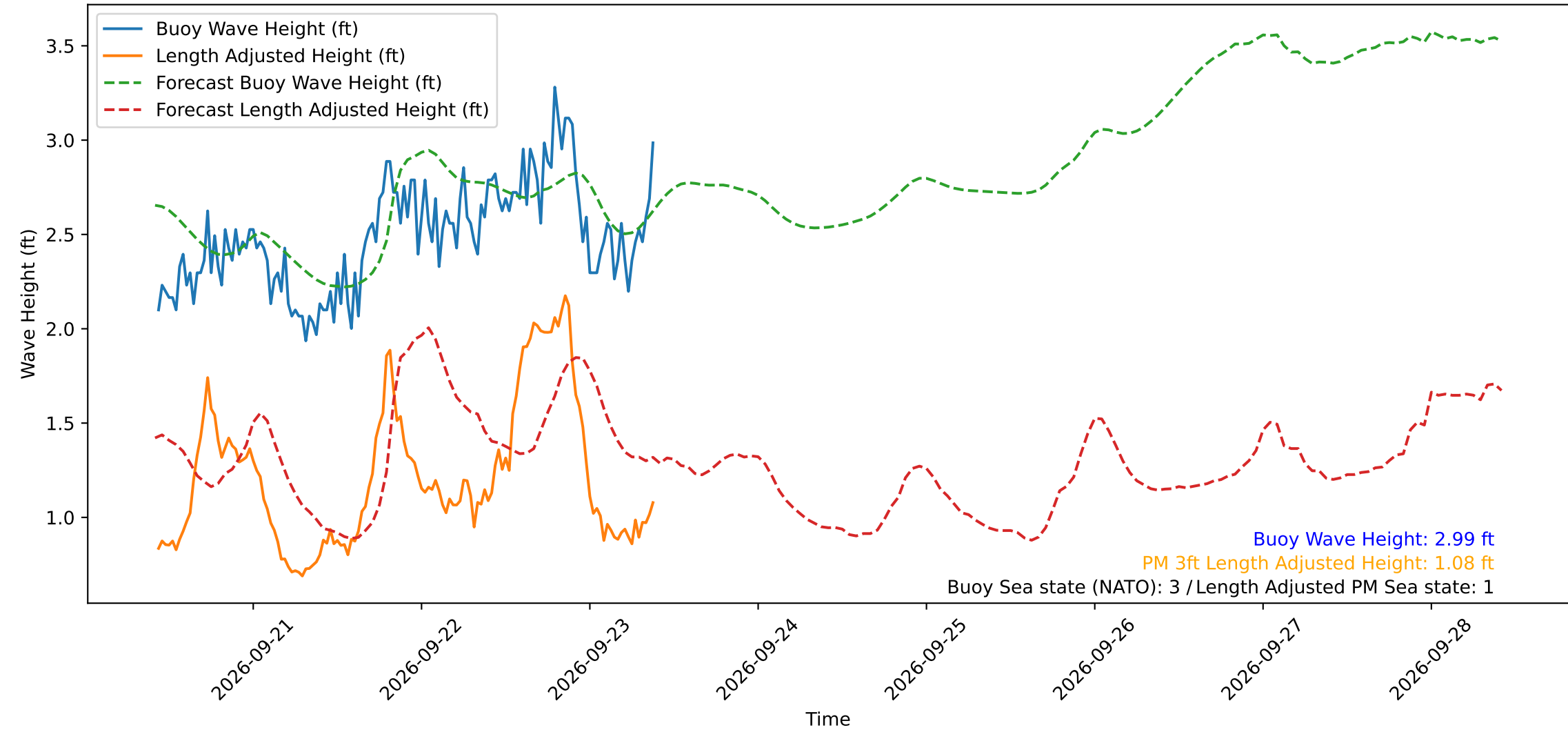
Wave Heights over Time for Red Beach at 2026-09-23 10:00:49
