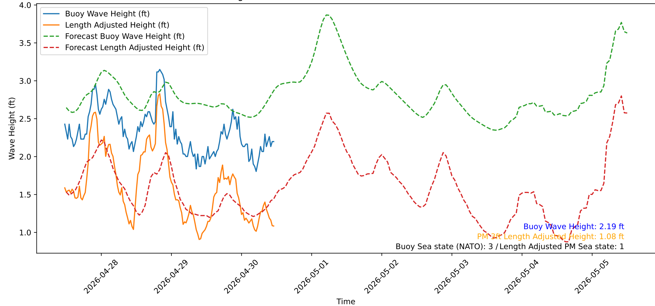
Wave Heights over Time for Green Beach at 2026-04-30 11:41:13
