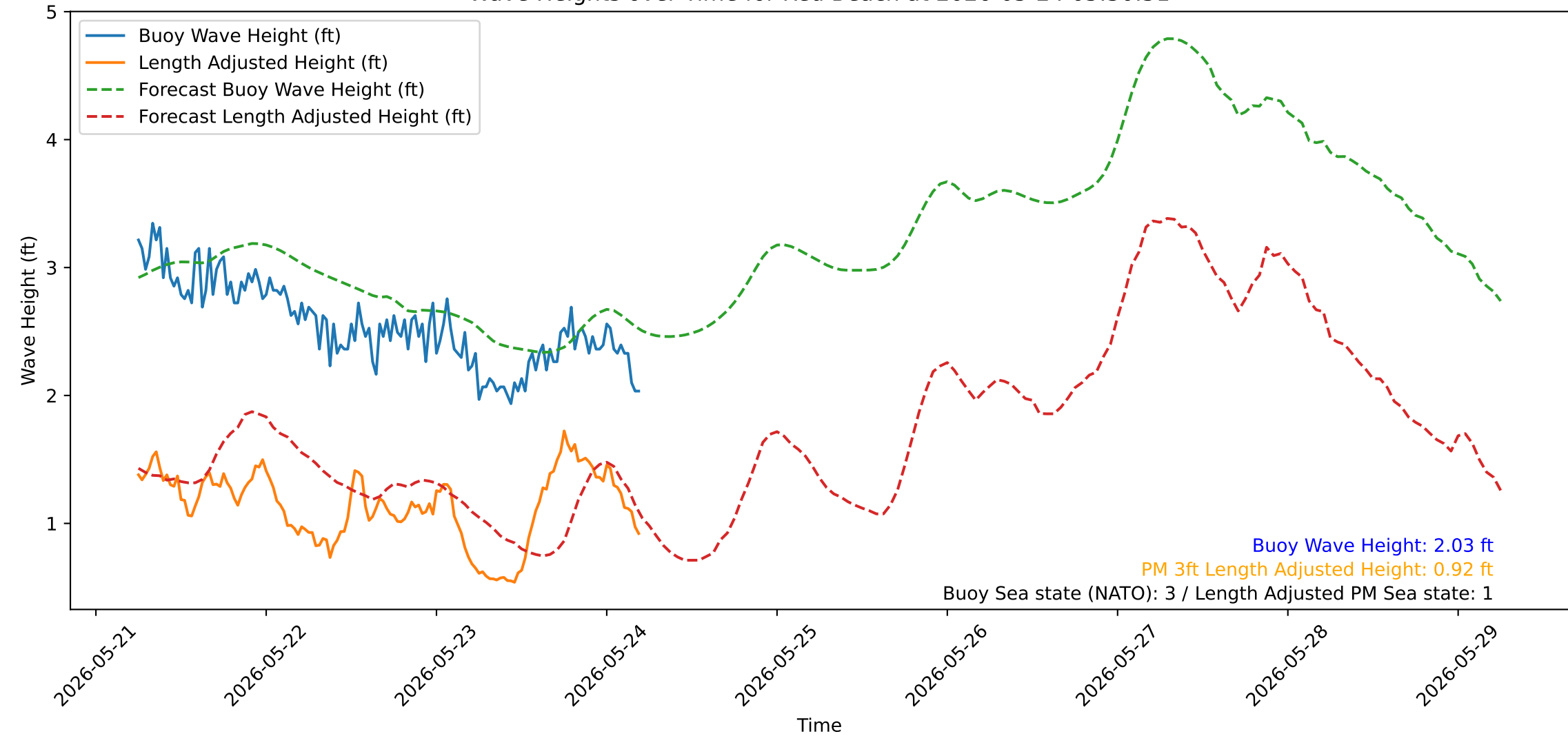
Wave Heights over Time for Red Beach at 2026-05-24 05:30:51
