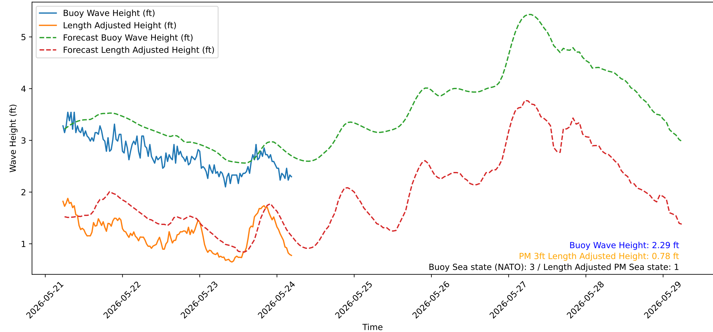
Wave Heights over Time for Green Beach at 2026-05-24 05:31:14
