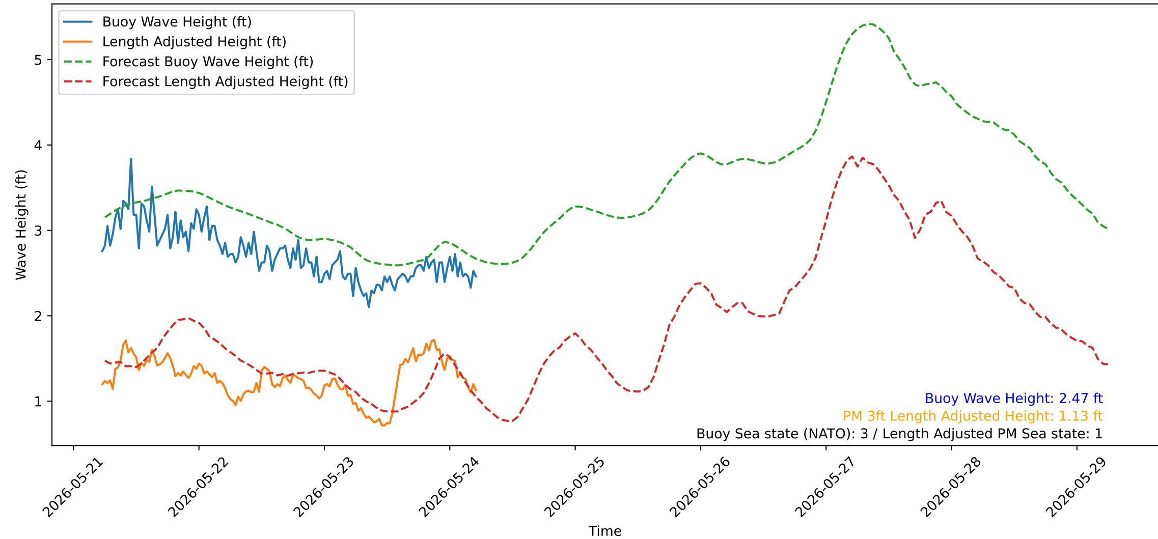
Wave Heights over Time for Oceanside Harbor at 2026-05-24 05:30:32
