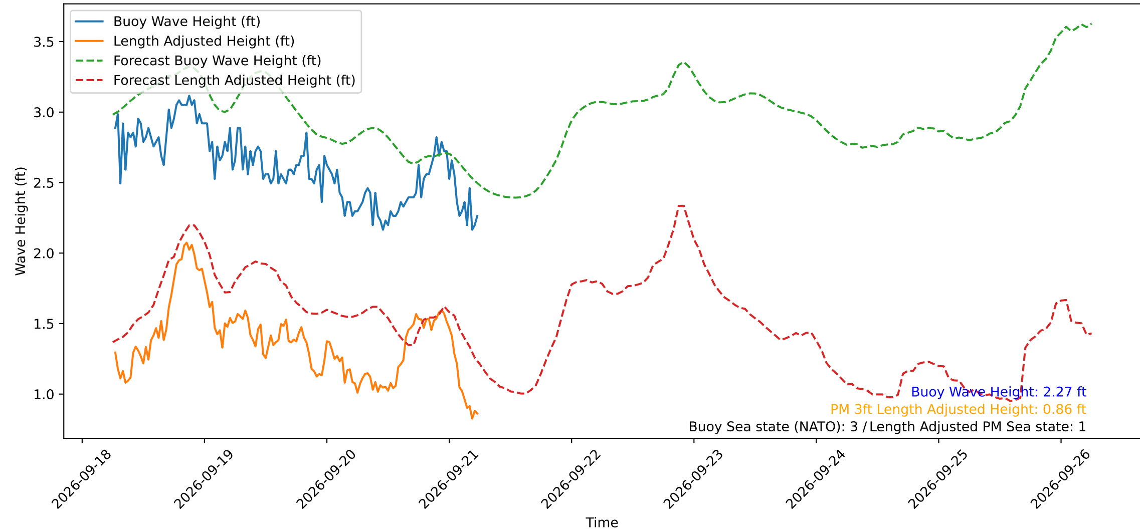
Wave Heights over Time for Green Beach at 2026-09-21 06:21:16
