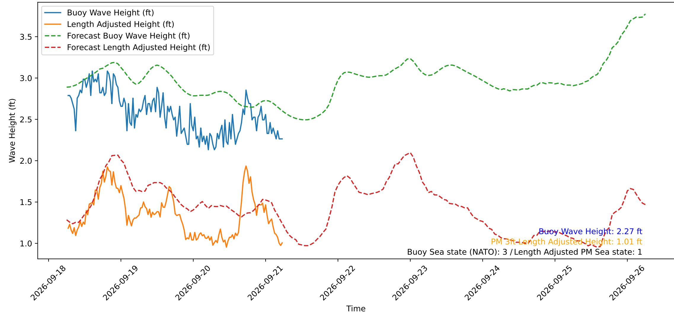
Wave Heights over Time for Oceanside Harbor at 2026-09-21 06:20:30
