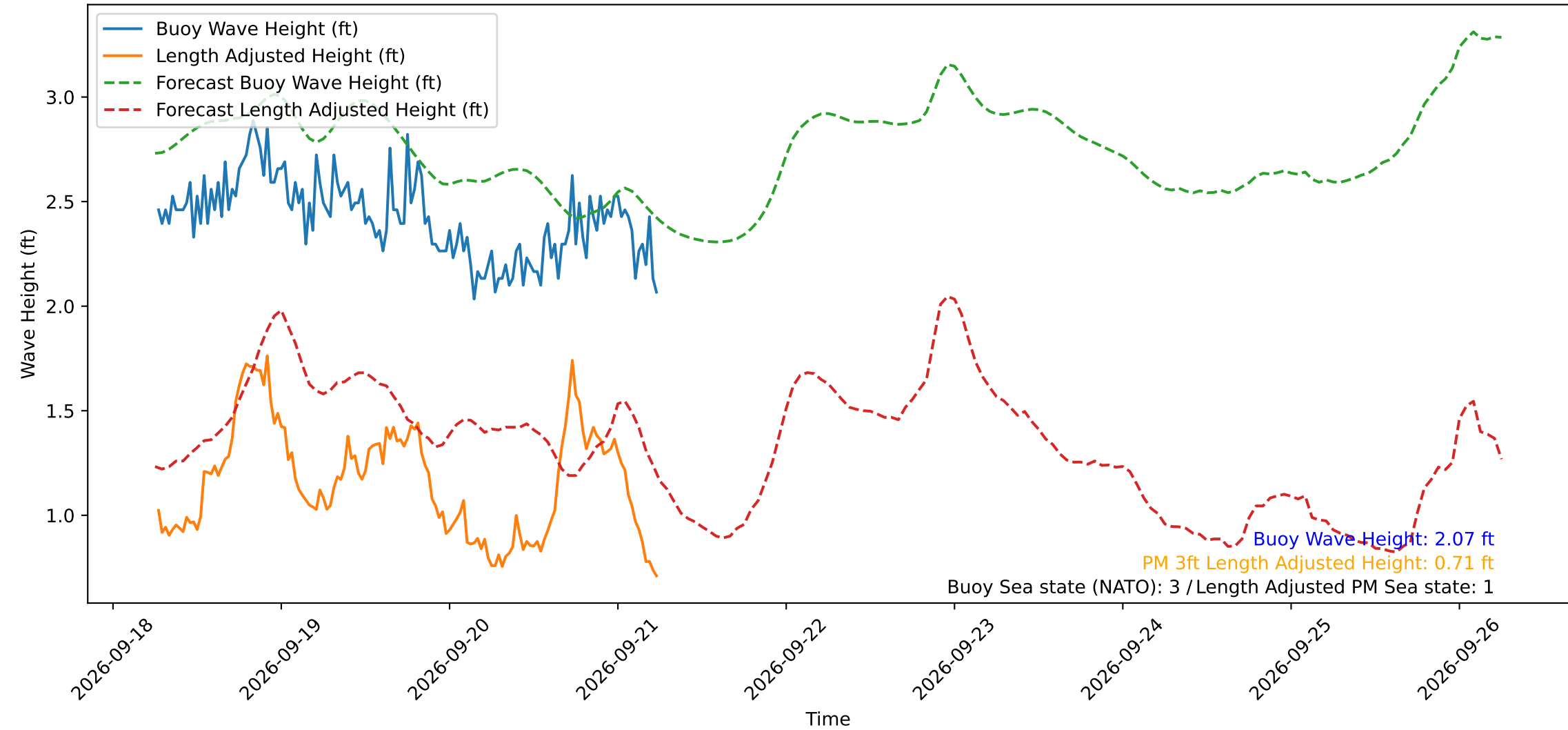
Wave Heights over Time for Red Beach at 2026-09-21 06:20:51
