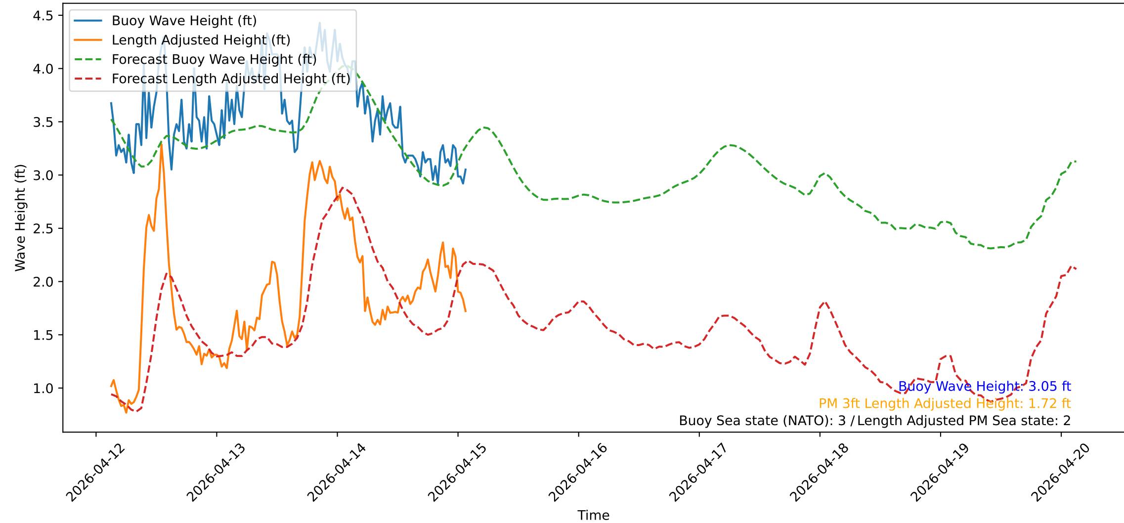
Wave Heights over Time for Red Beach at 2026-04-15 02:30:50
