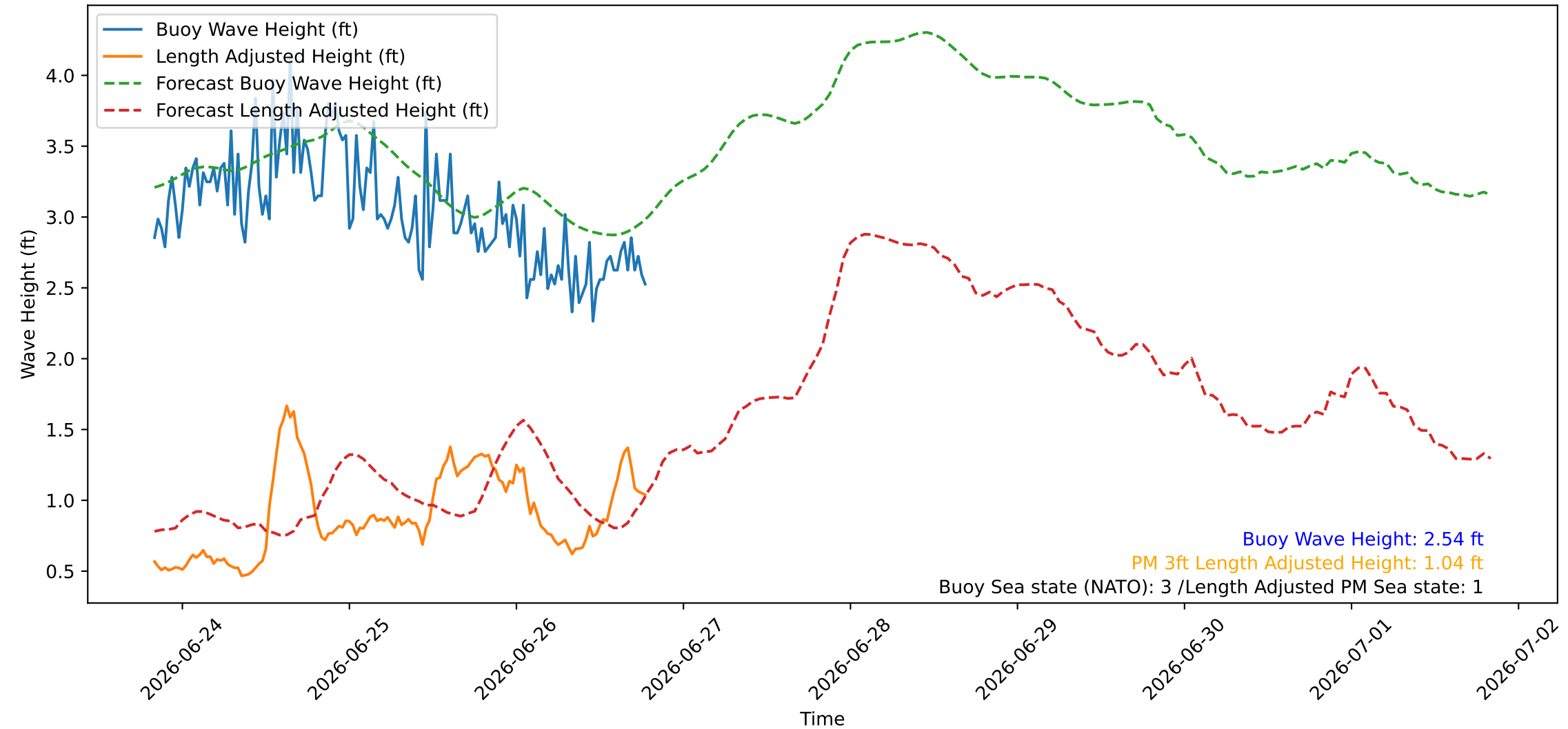
Wave Heights over Time for Red Beach at 2026-06-26 19:50:47
