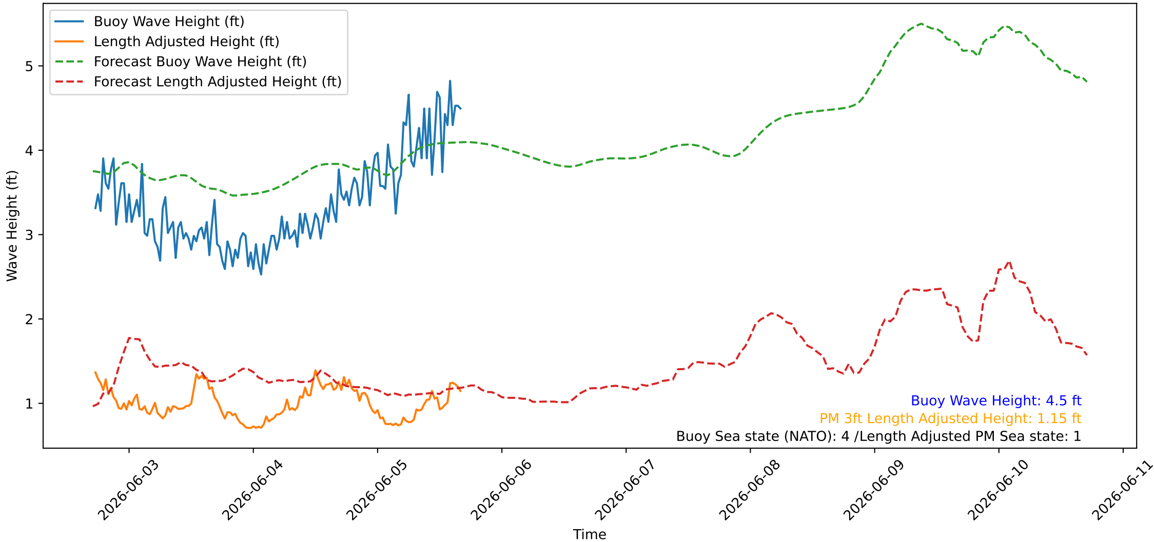
Wave Heights over Time for Red Beach at 2026-06-05 17:10:45
