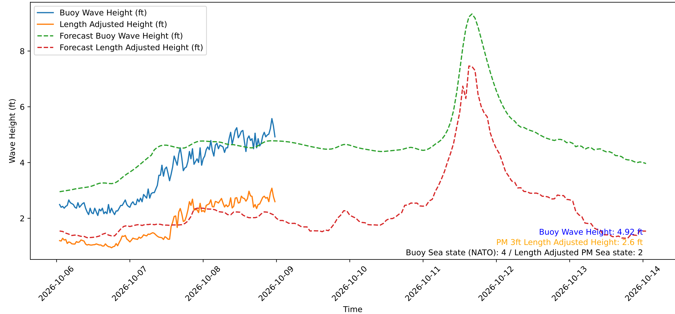
Wave Heights over Time for Green Beach at 2026-10-09 00:41:11
