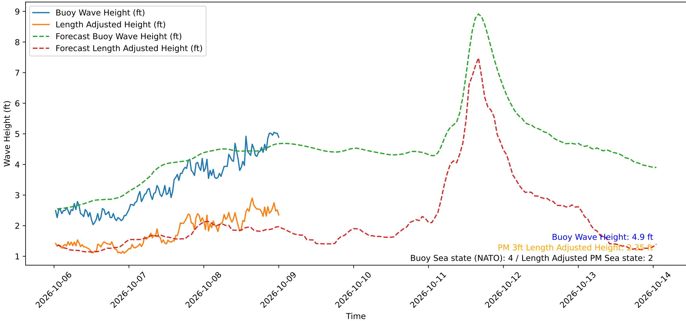
Wave Heights over Time for Oceanside Harbor at 2026-10-09 00:40:29
