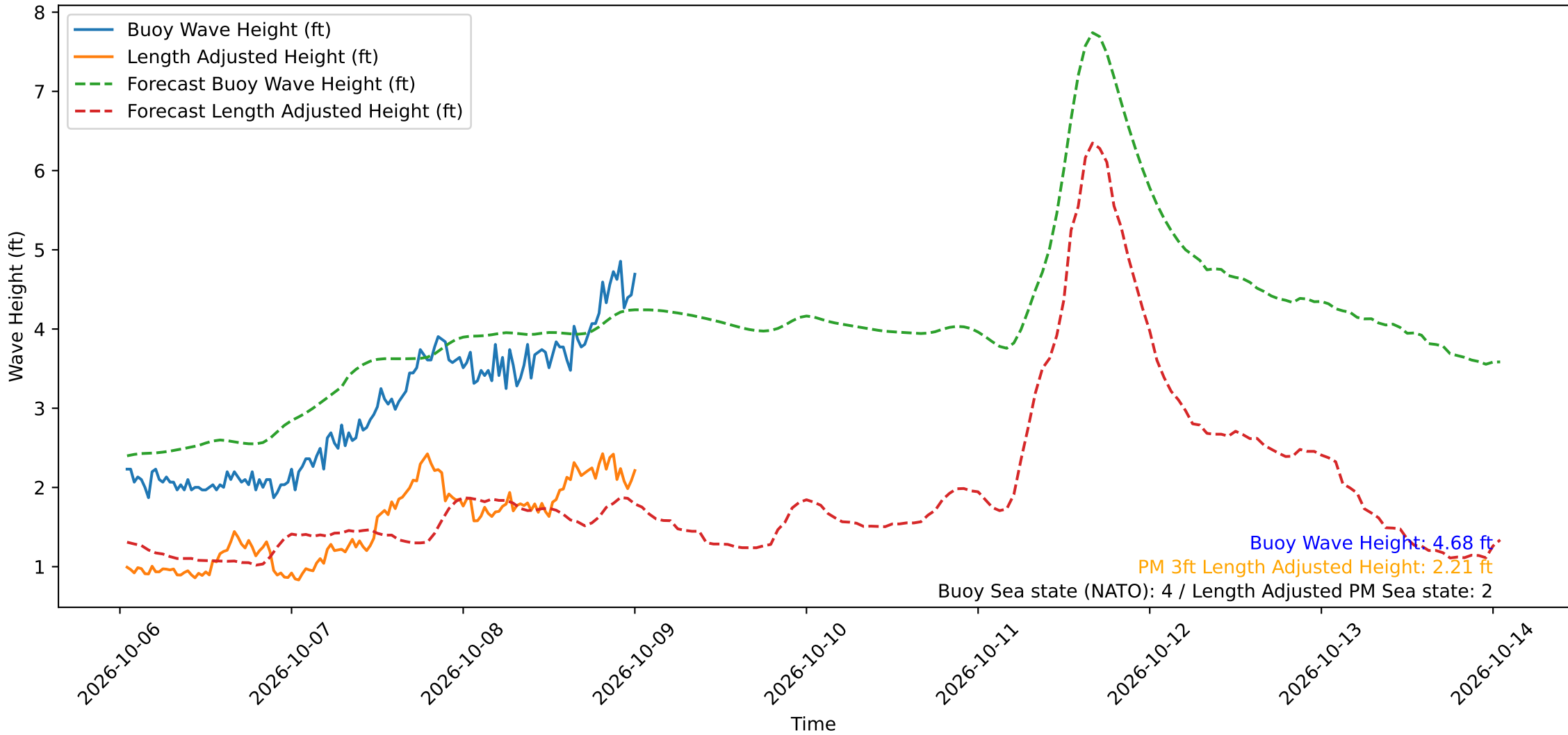
Wave Heights over Time for Red Beach at 2026-10-09 00:40:48
