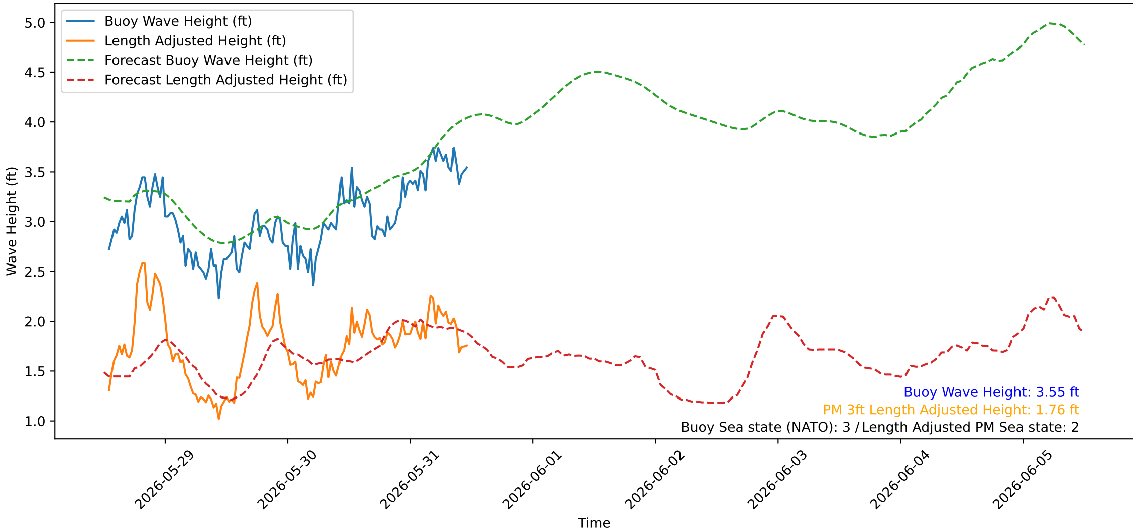
Wave Heights over Time for Oceanside Harbor at 2026-05-31 12:00:26
