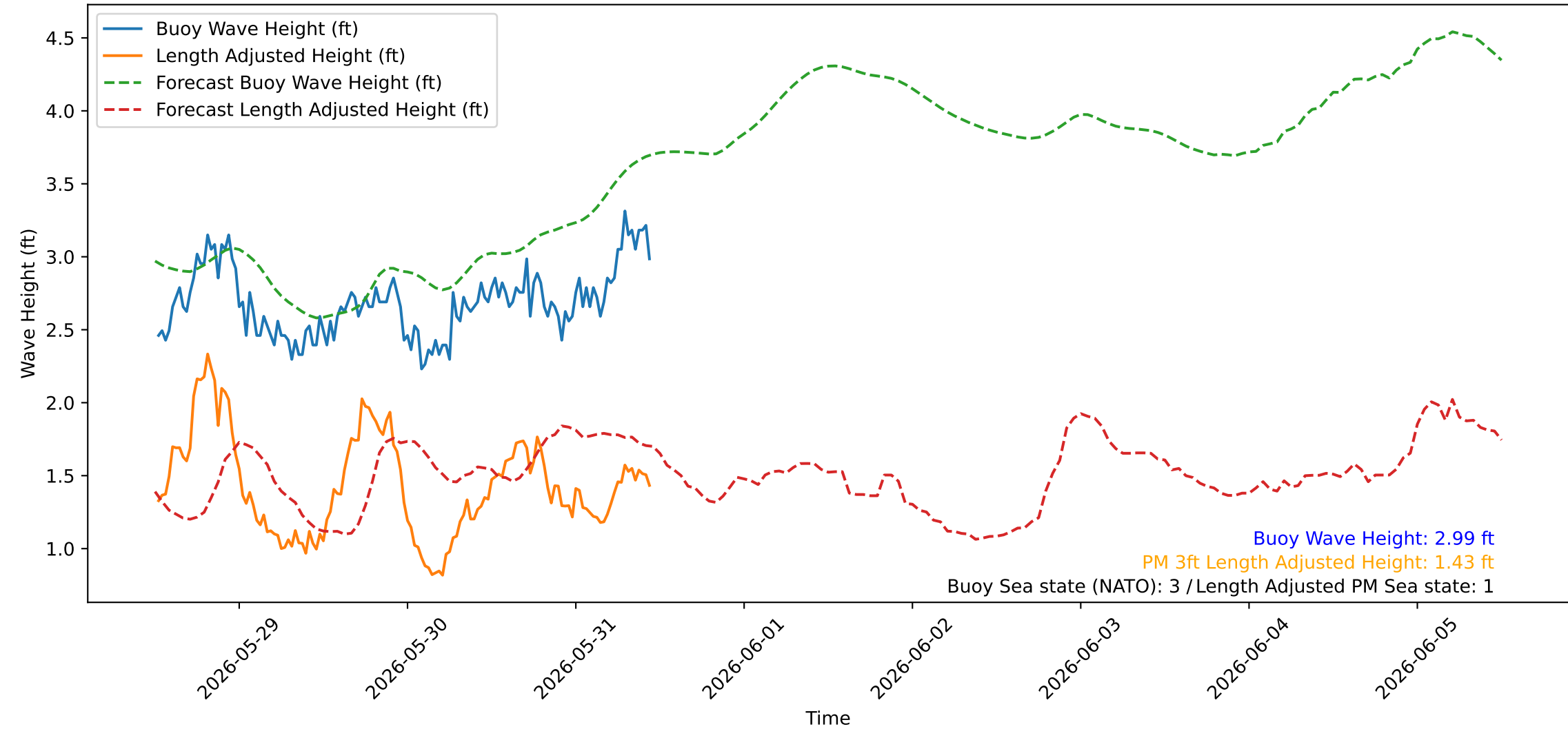
Wave Heights over Time for Red Beach at 2026-05-31 12:00:45
