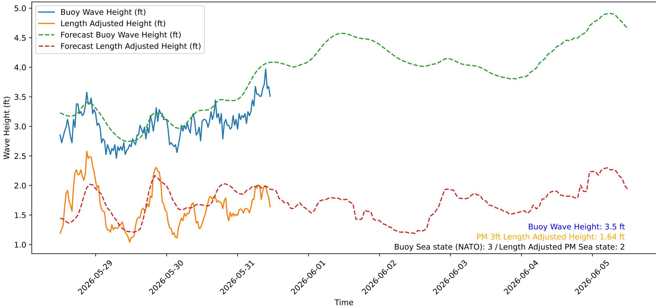
Wave Heights over Time for Green Beach at 2026-05-31 12:01:08
