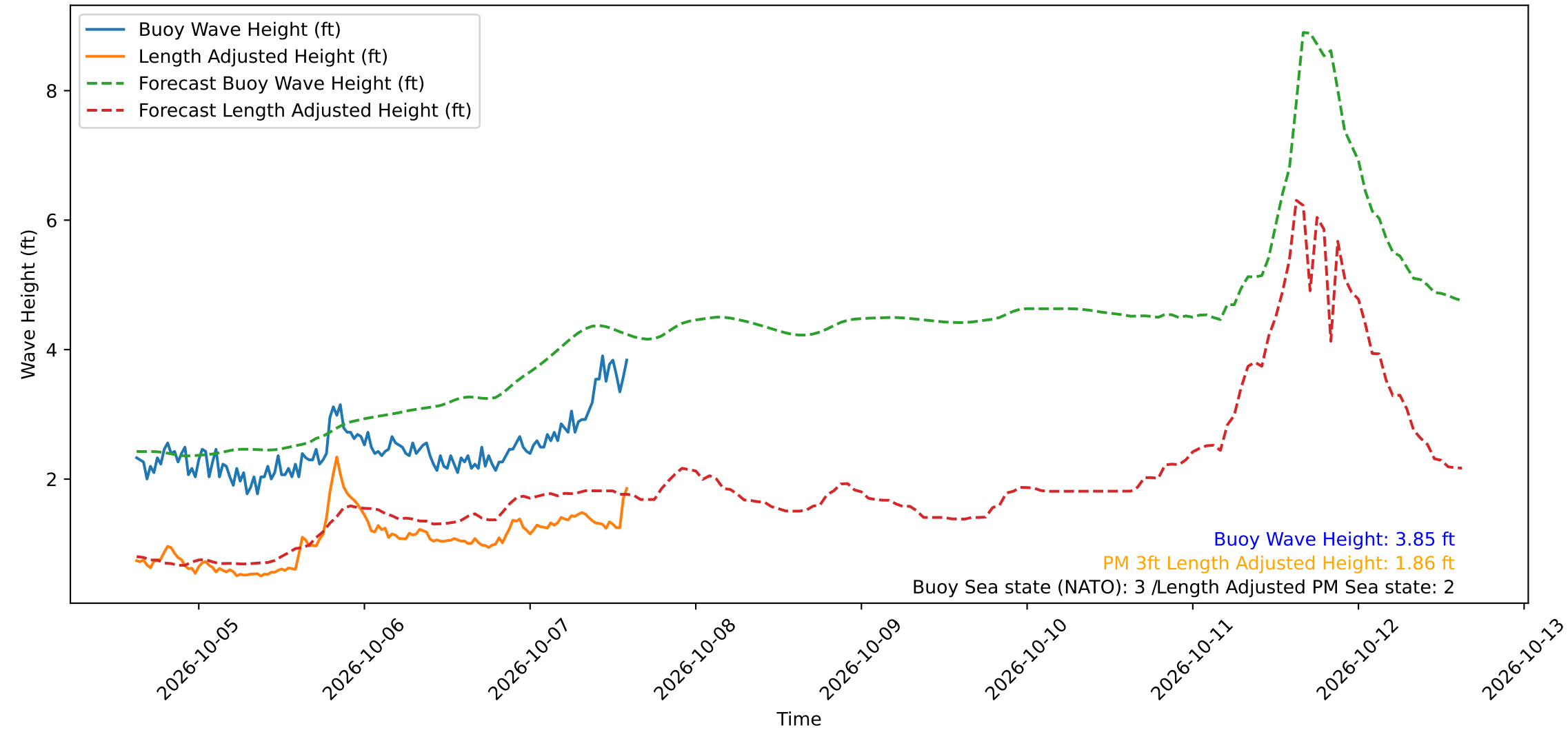
Wave Heights over Time for Green Beach at 2026-10-07 14:51:16
