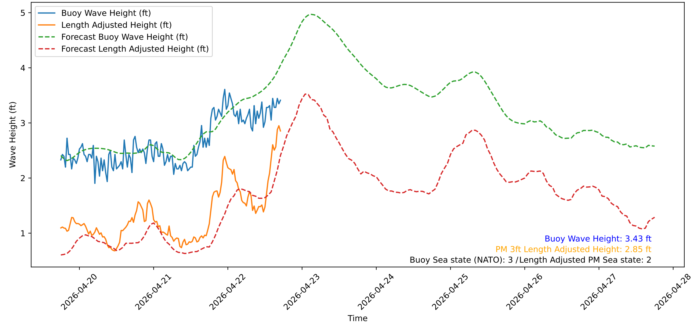
Wave Heights over Time for Oceanside Harbor at 2026-04-22 18:00:32
