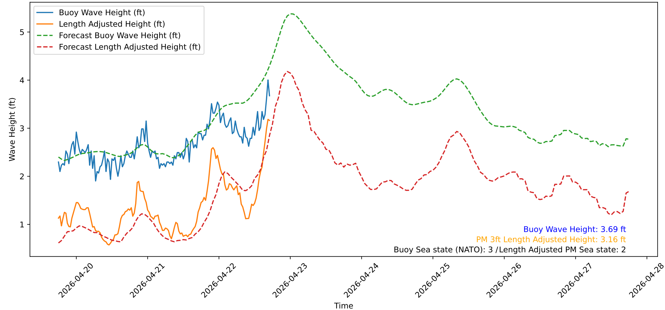
Wave Heights over Time for Green Beach at 2026-04-22 18:01:13
