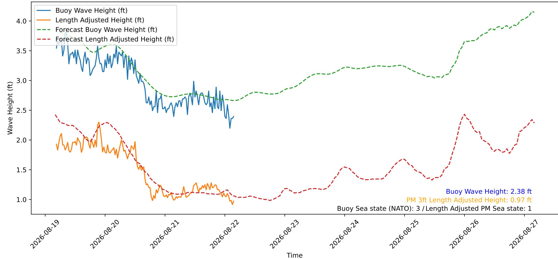
Wave Heights over Time for Oceanside Harbor at 2026-08-22 04:20:29
