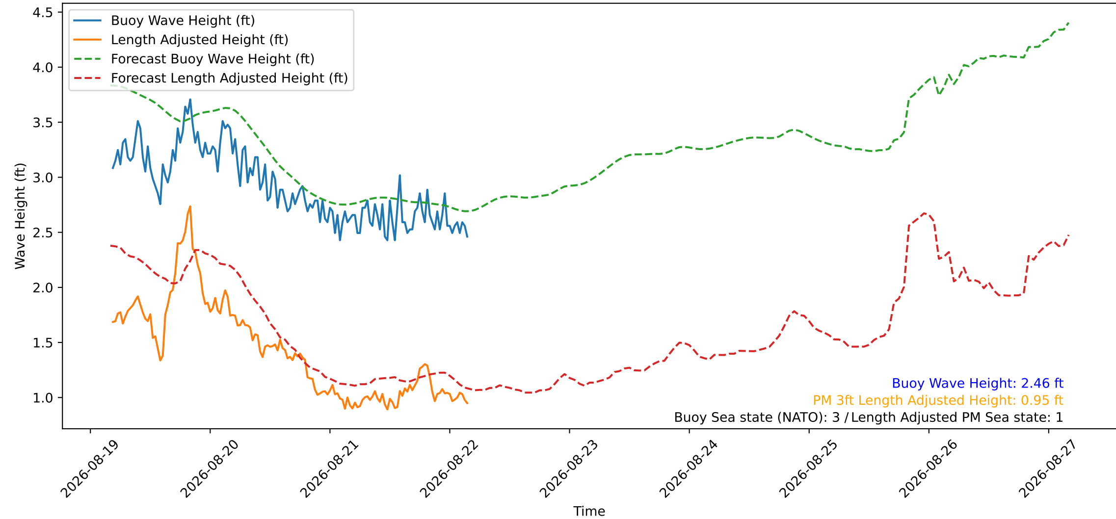
Wave Heights over Time for Green Beach at 2026-08-22 04:21:14
