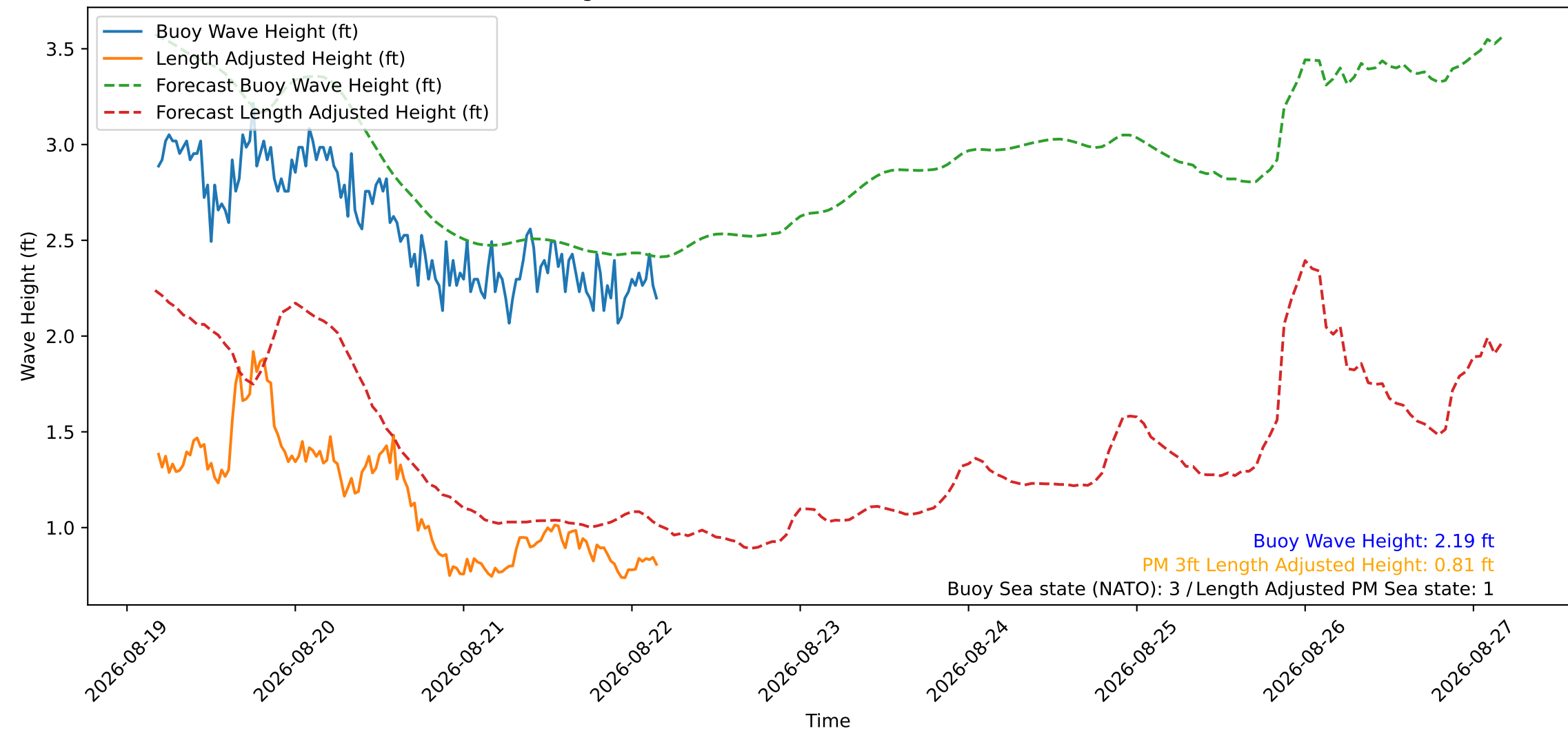
Wave Heights over Time for Red Beach at 2026-08-22 04:20:50
