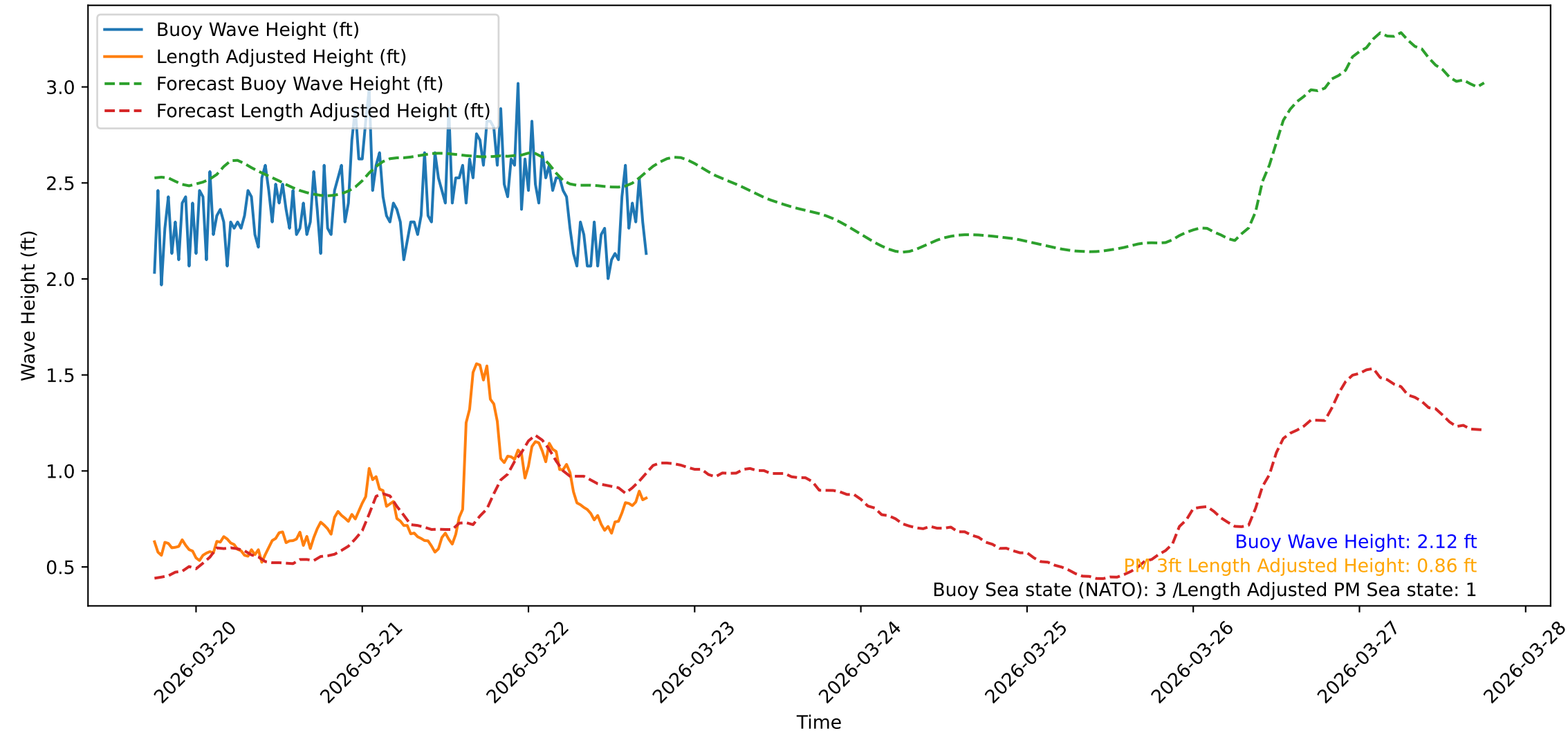
Wave Heights over Time for Oceanside Harbor at 2026-03-22 18:00:32
