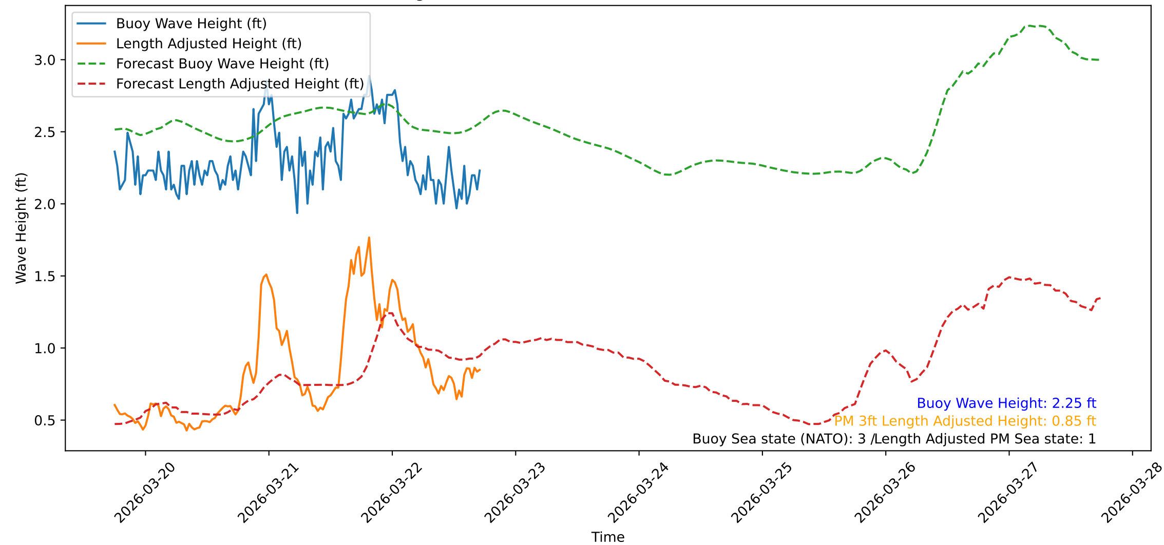
Wave Heights over Time for Green Beach at 2026-03-22 18:01:09
