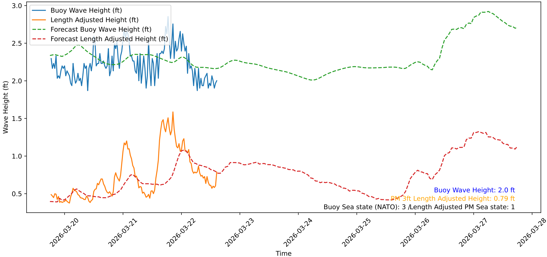
Wave Heights over Time for Red Beach at 2026-03-22 18:00:47
