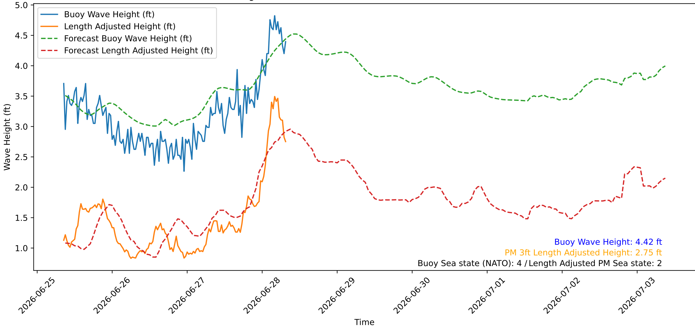
Wave Heights over Time for Green Beach at 2026-06-28 08:31:07
