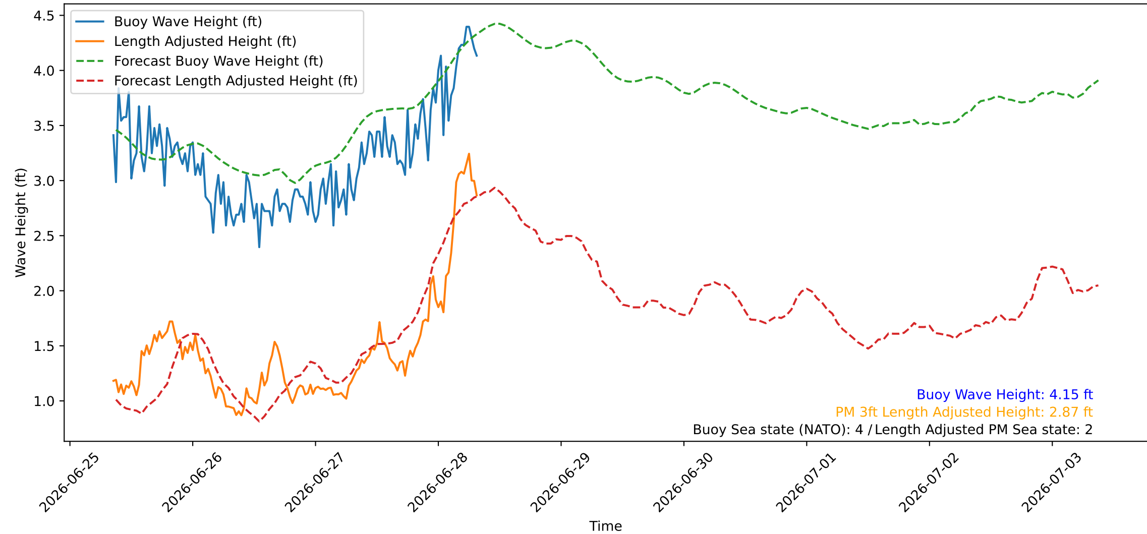
Wave Heights over Time for Oceanside Harbor at 2026-06-28 08:30:26
