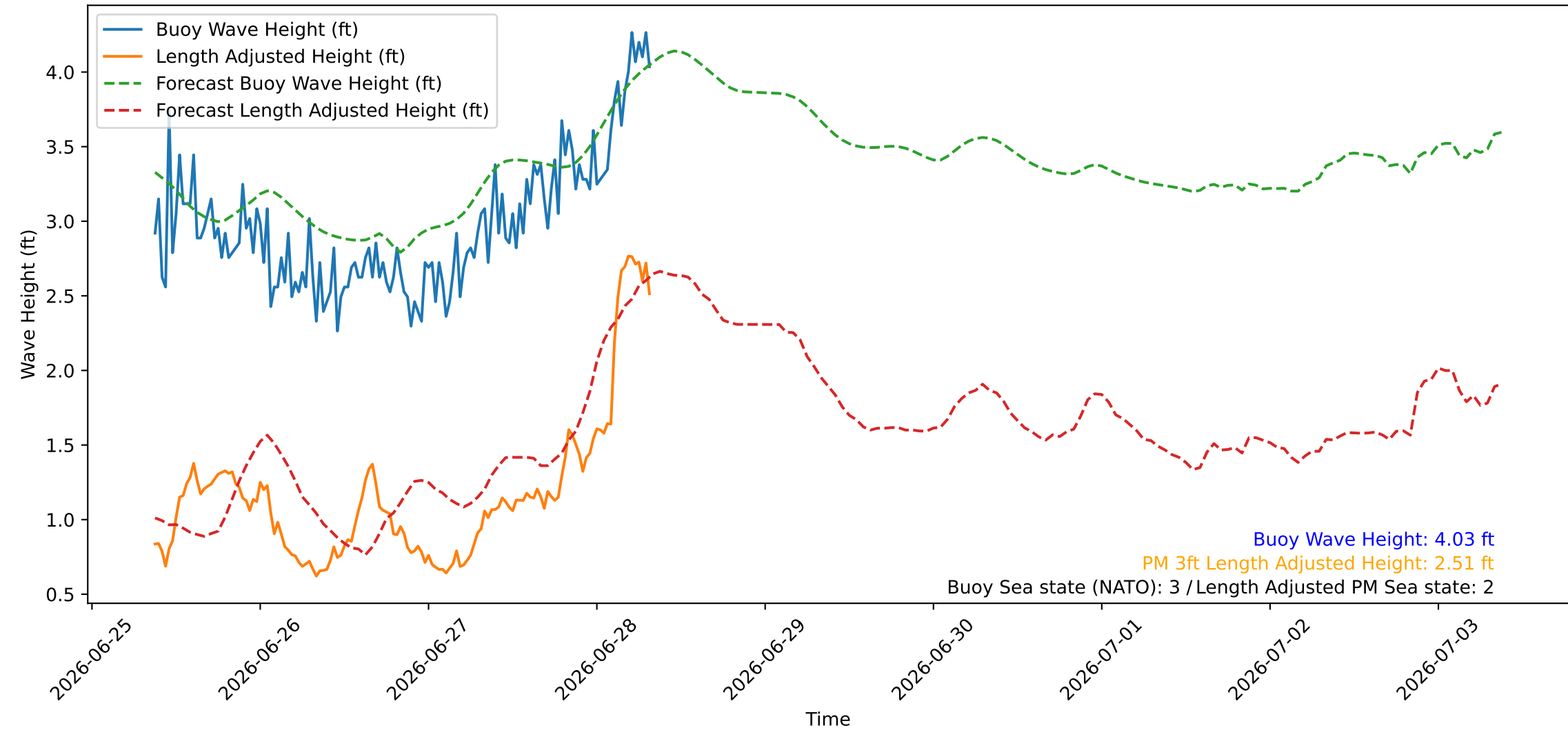
Wave Heights over Time for Red Beach at 2026-06-28 08:30:45
