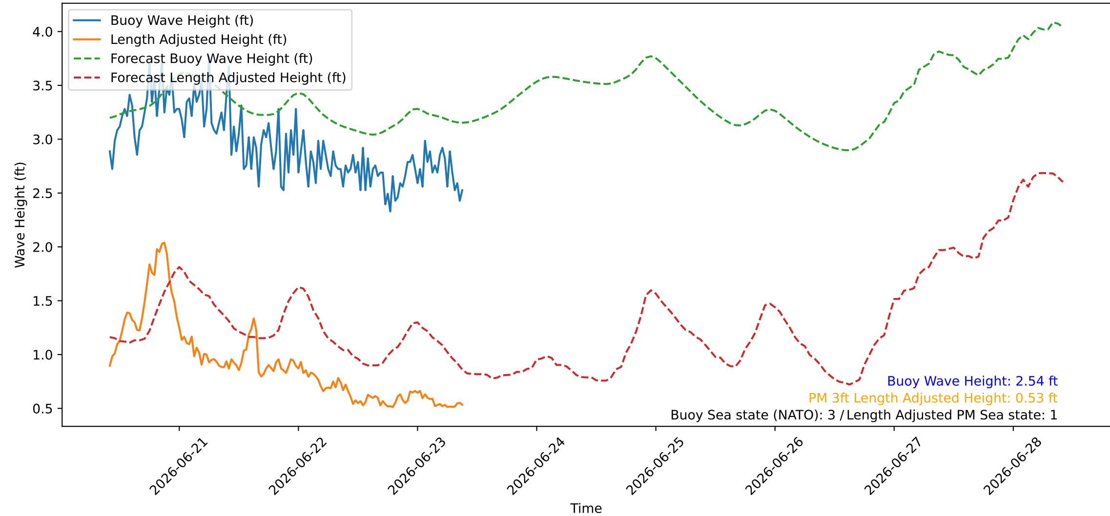
Wave Heights over Time for Red Beach at 2026-06-23 09:50:47
