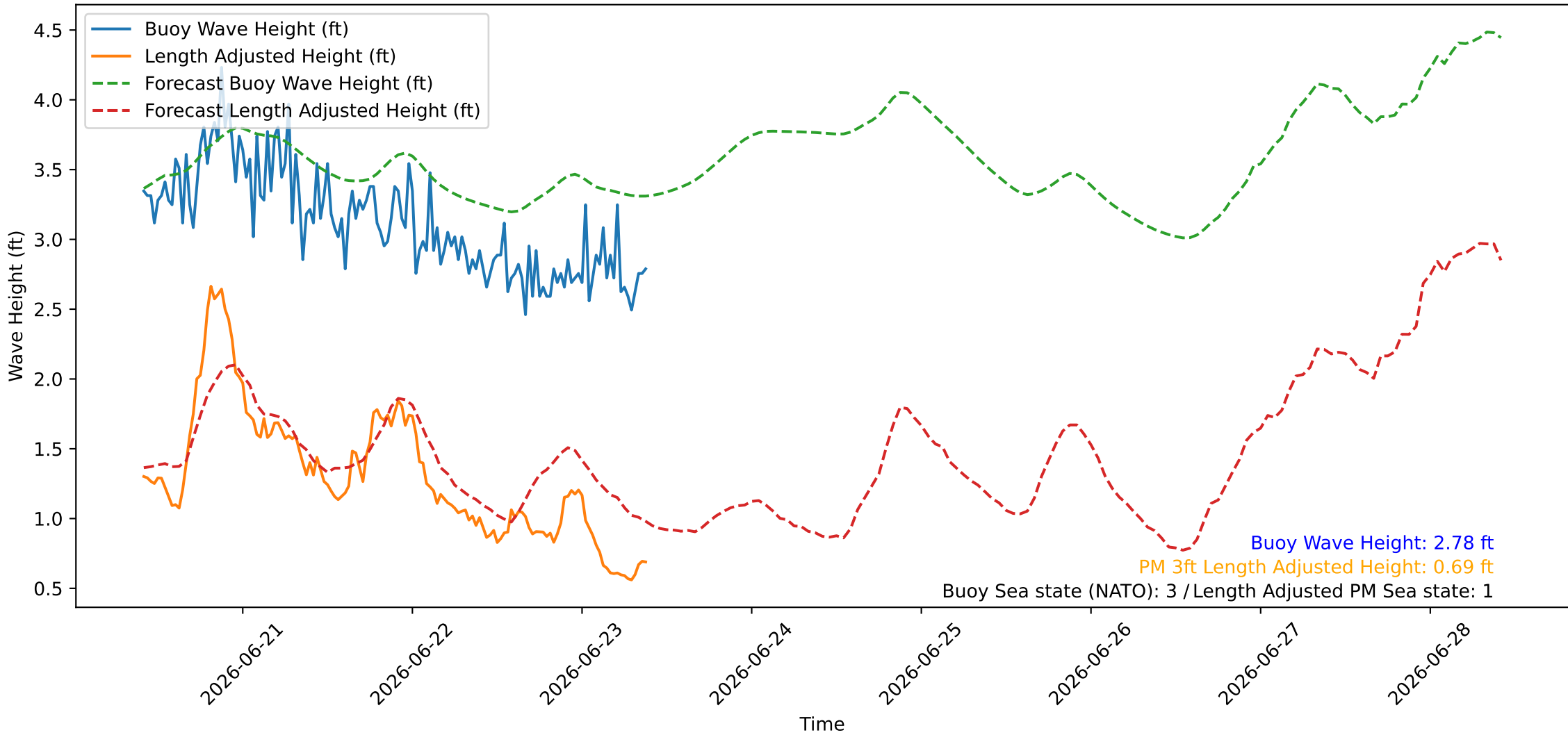
Wave Heights over Time for Green Beach at 2026-06-23 09:51:10
