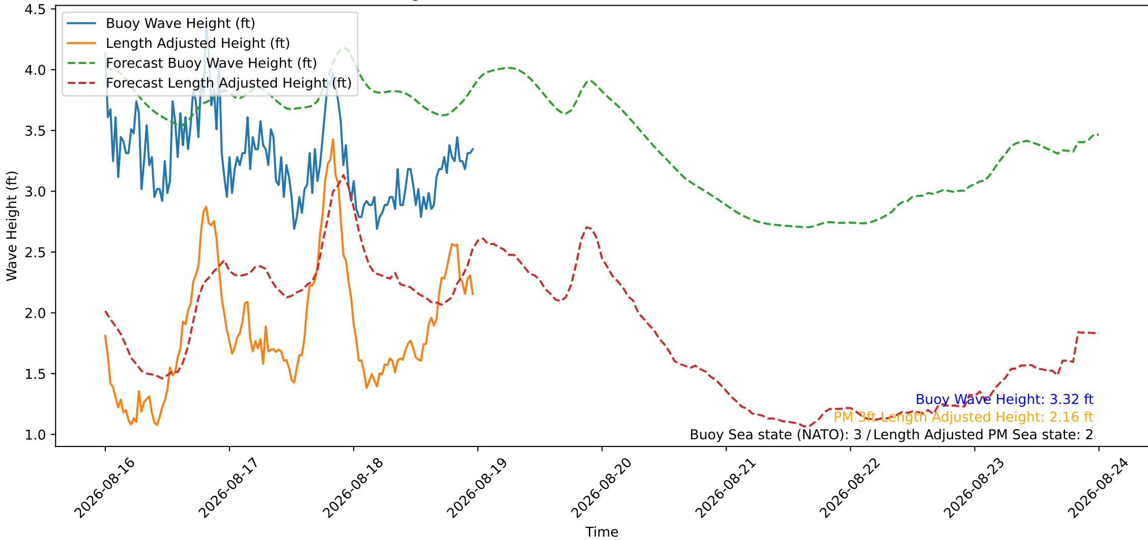
Wave Heights over Time for Green Beach at 2026-08-18 23:51:10
