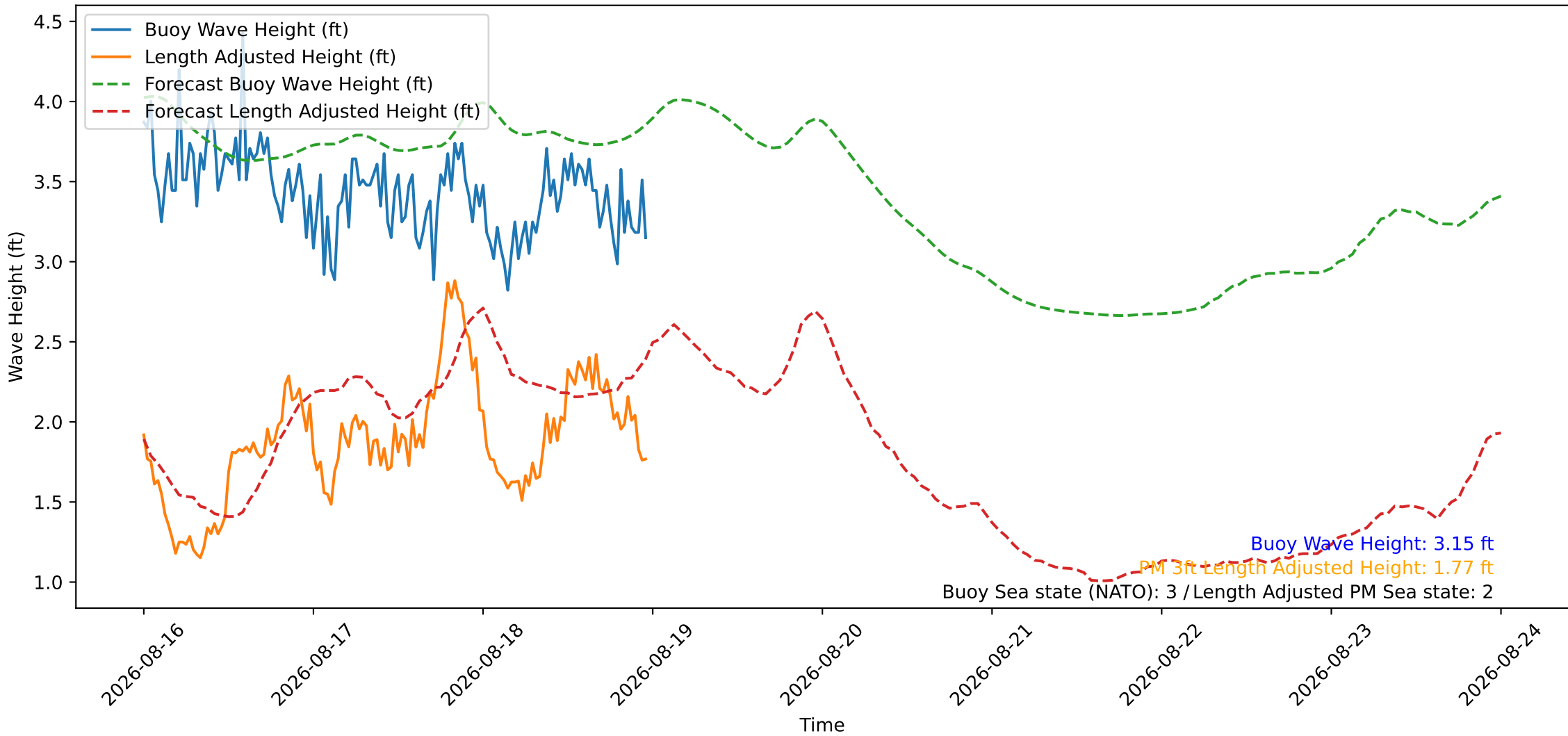
Wave Heights over Time for Oceanside Harbor at 2026-08-18 23:50:26
