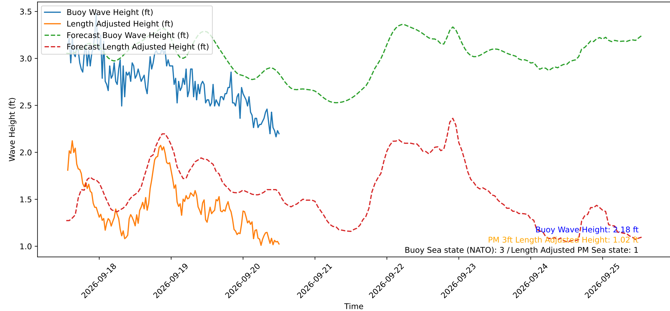
Wave Heights over Time for Green Beach at 2026-09-20 13:01:11
