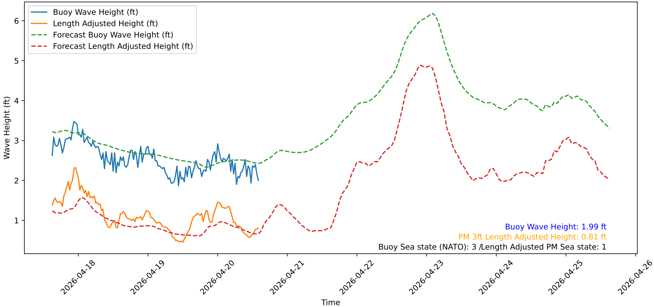
Wave Heights over Time for Green Beach at 2026-04-20 14:51:14
