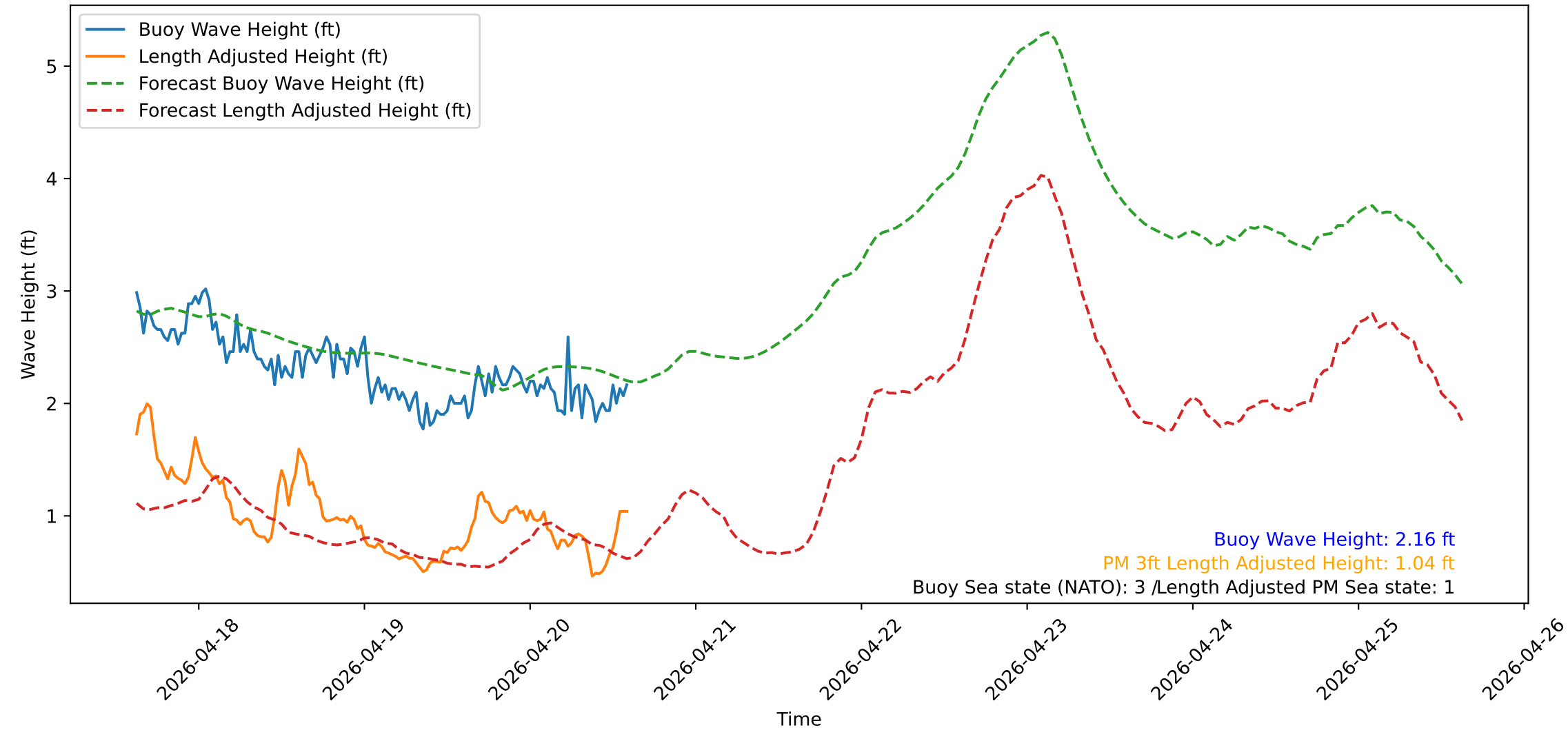
Wave Heights over Time for Red Beach at 2026-04-20 14:50:51
