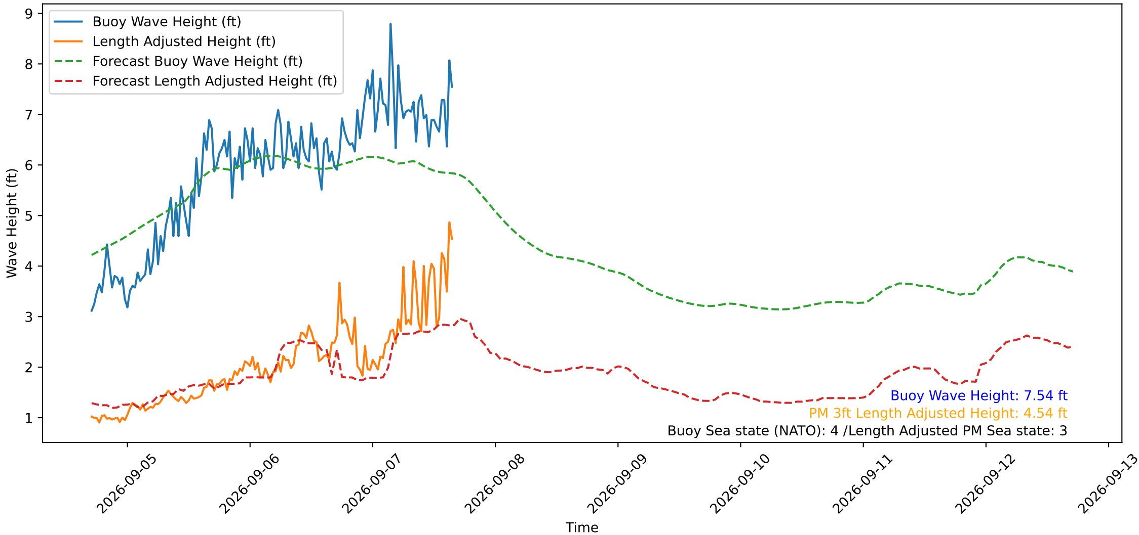
Wave Heights over Time for Green Beach at 2026-09-07 16:31:12
