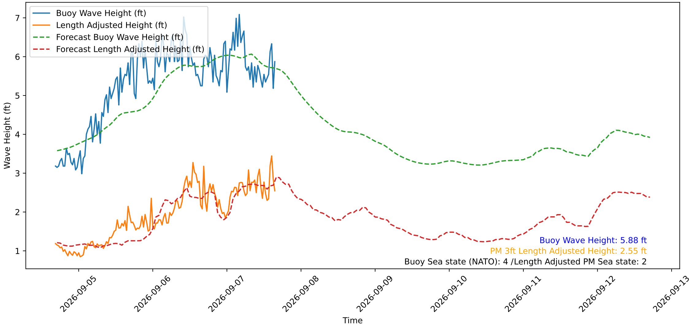
Wave Heights over Time for Oceanside Harbor at 2026-09-07 16:30:30
