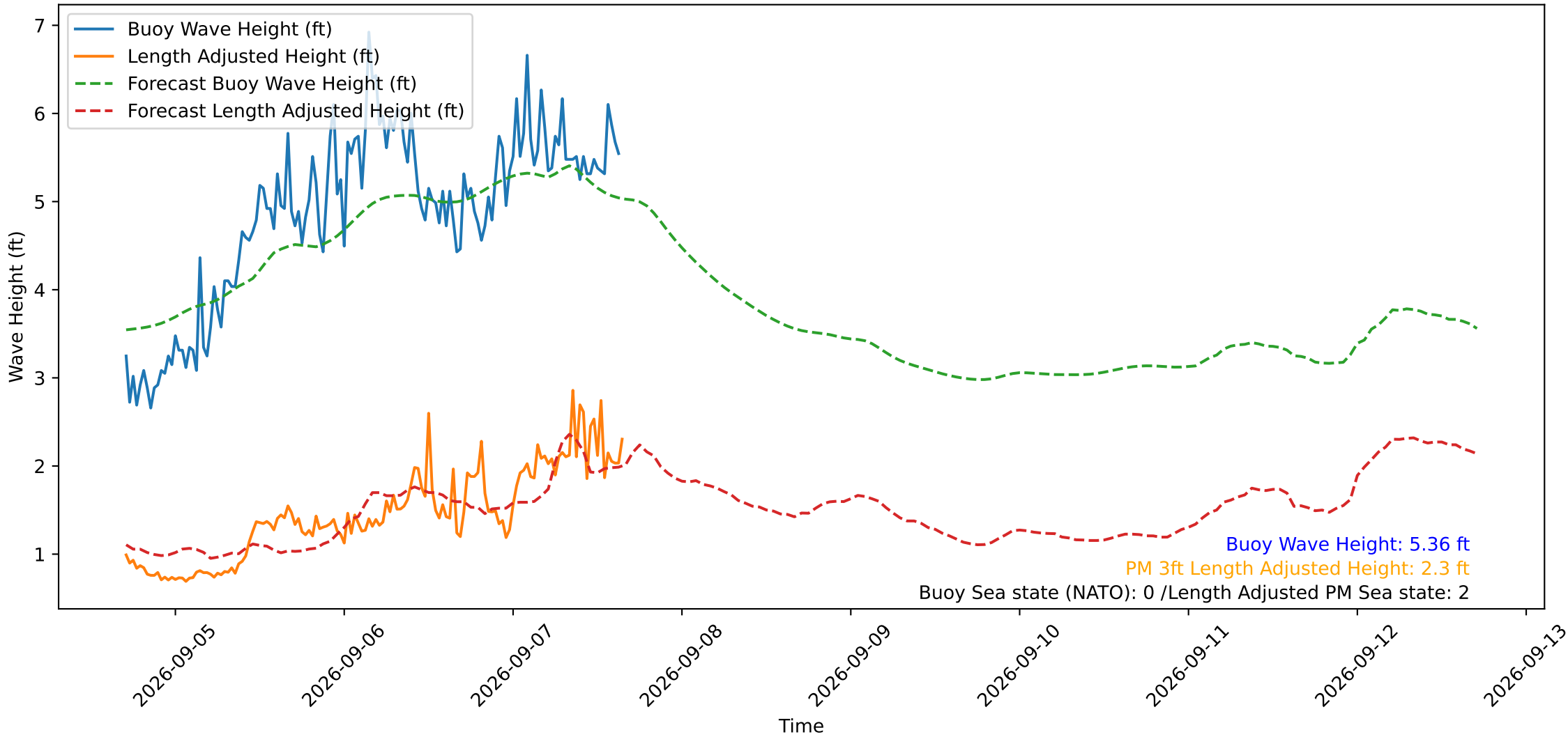
Wave Heights over Time for Red Beach at 2026-09-07 16:30:50
