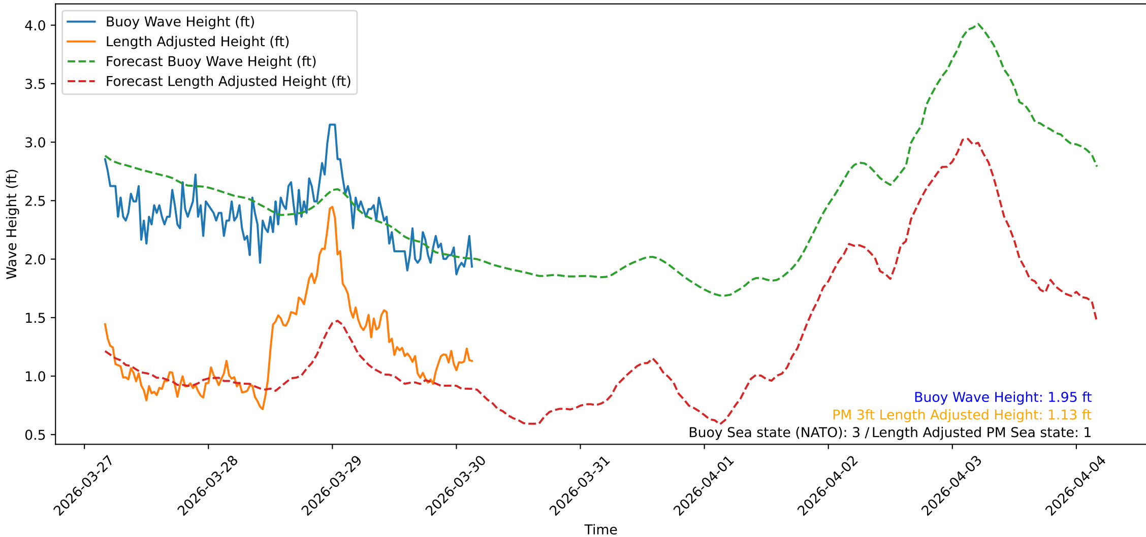
Wave Heights over Time for Oceanside Harbor at 2026-03-30 03:50:31
