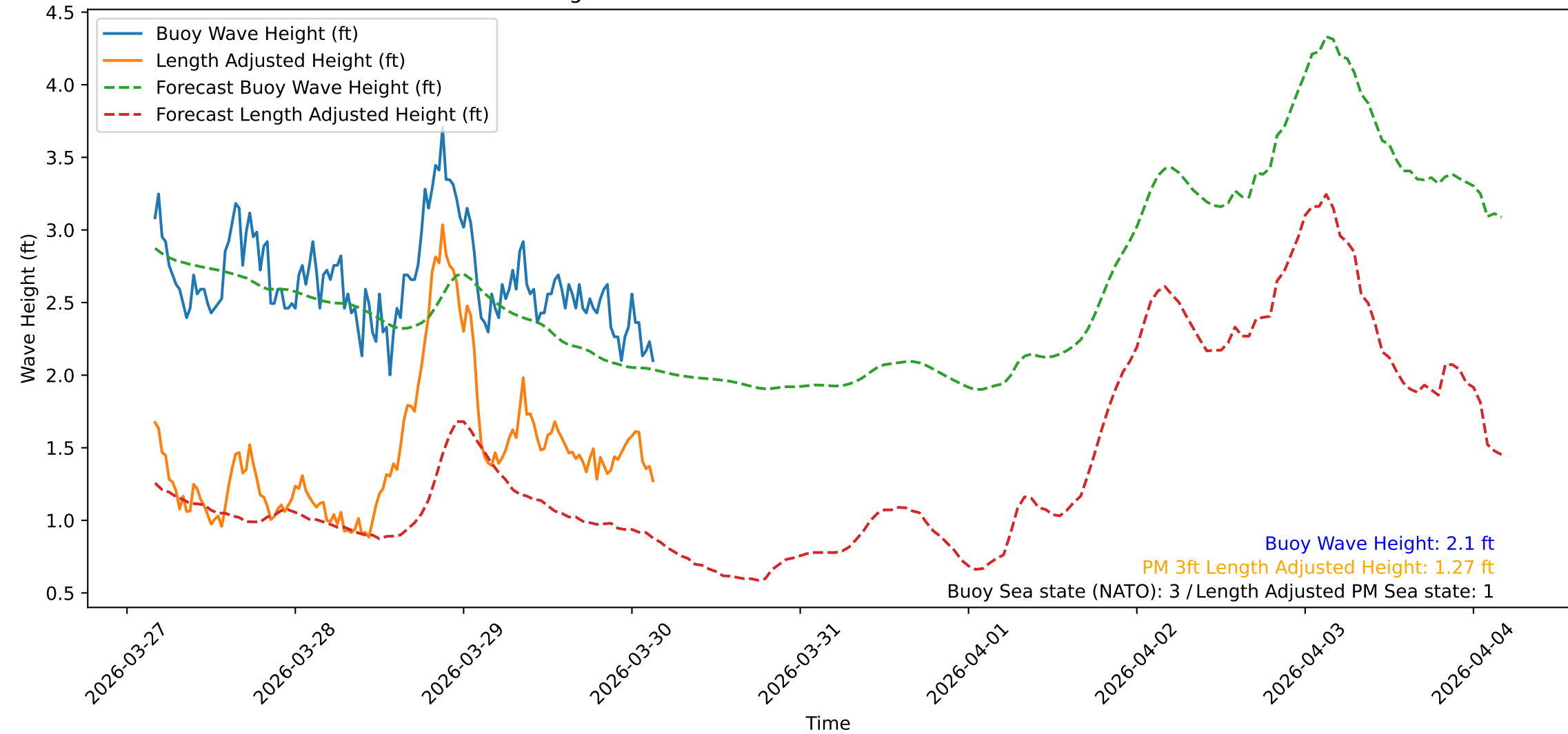
Wave Heights over Time for Green Beach at 2026-03-30 03:51:09
