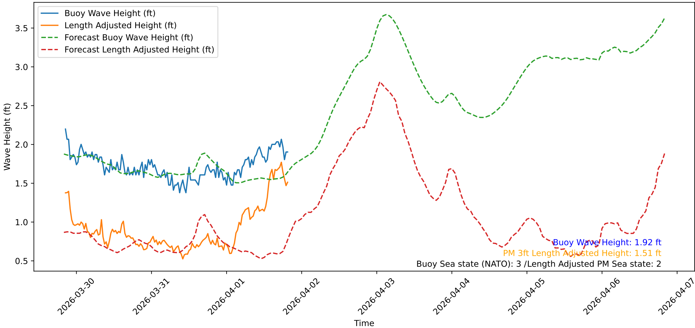
Wave Heights over Time for Red Beach at 2026-04-01 20:20:47
