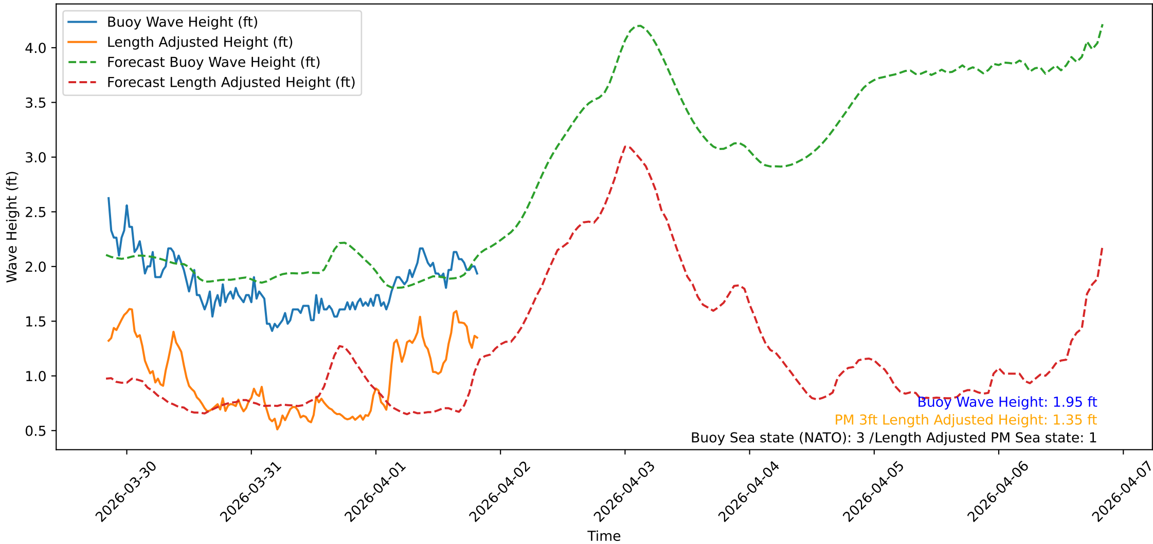
Wave Heights over Time for Green Beach at 2026-04-01 20:21:10
