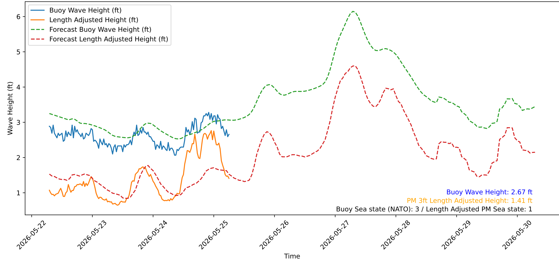
Wave Heights over Time for Green Beach at 2026-05-25 07:01:13
