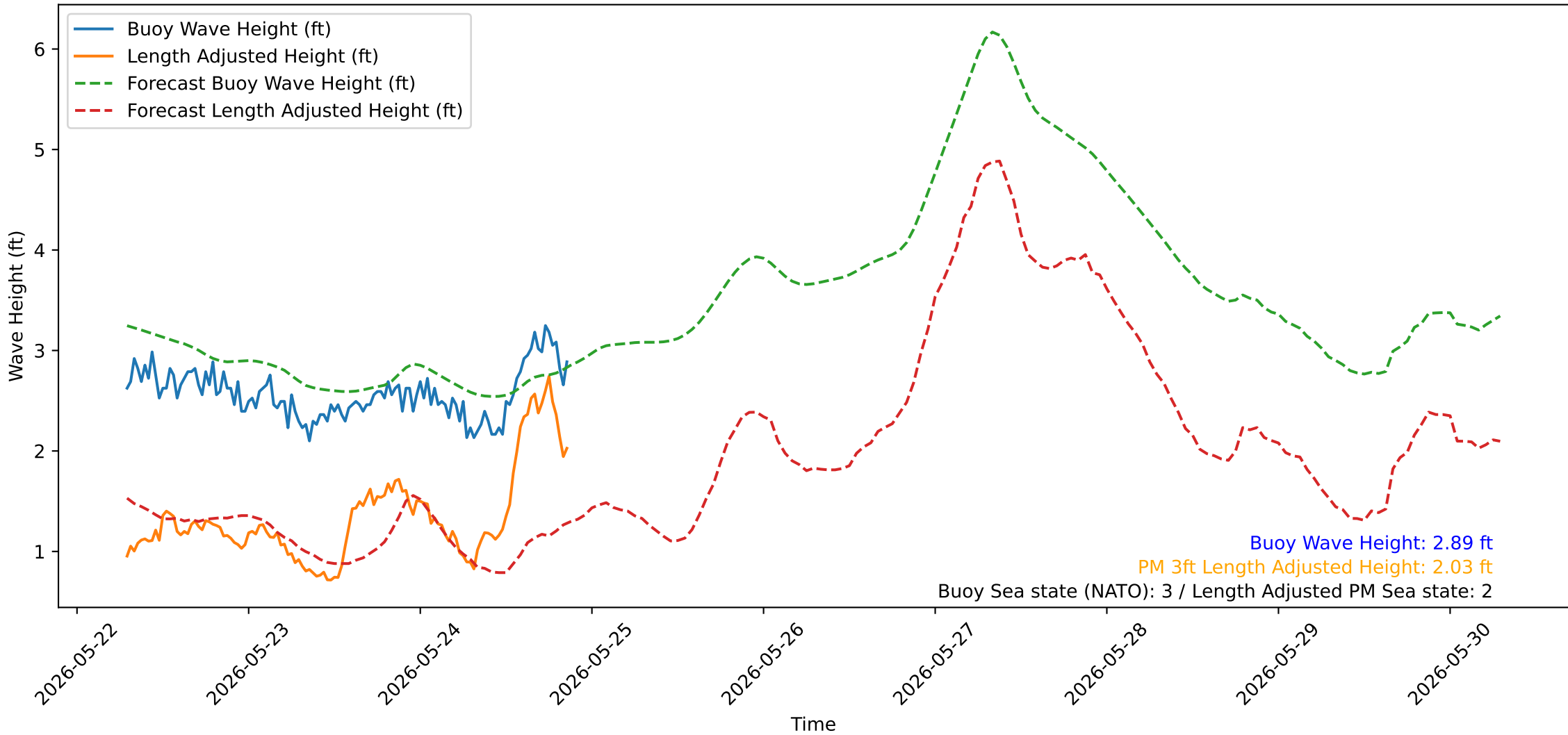
Wave Heights over Time for Oceanside Harbor at 2026-05-25 07:00:30
