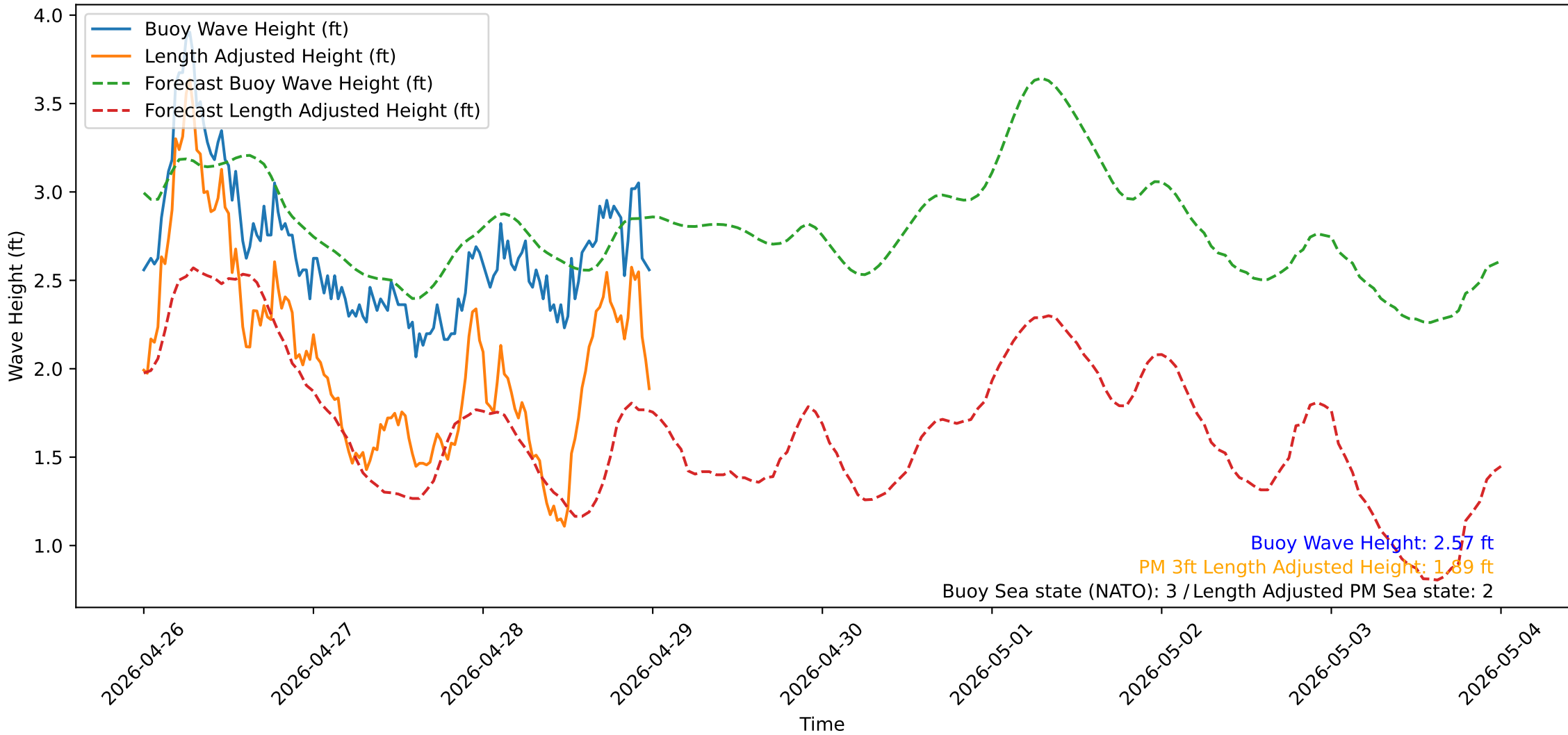
Wave Heights over Time for Oceanside Harbor at 2026-04-29 00:10:32
