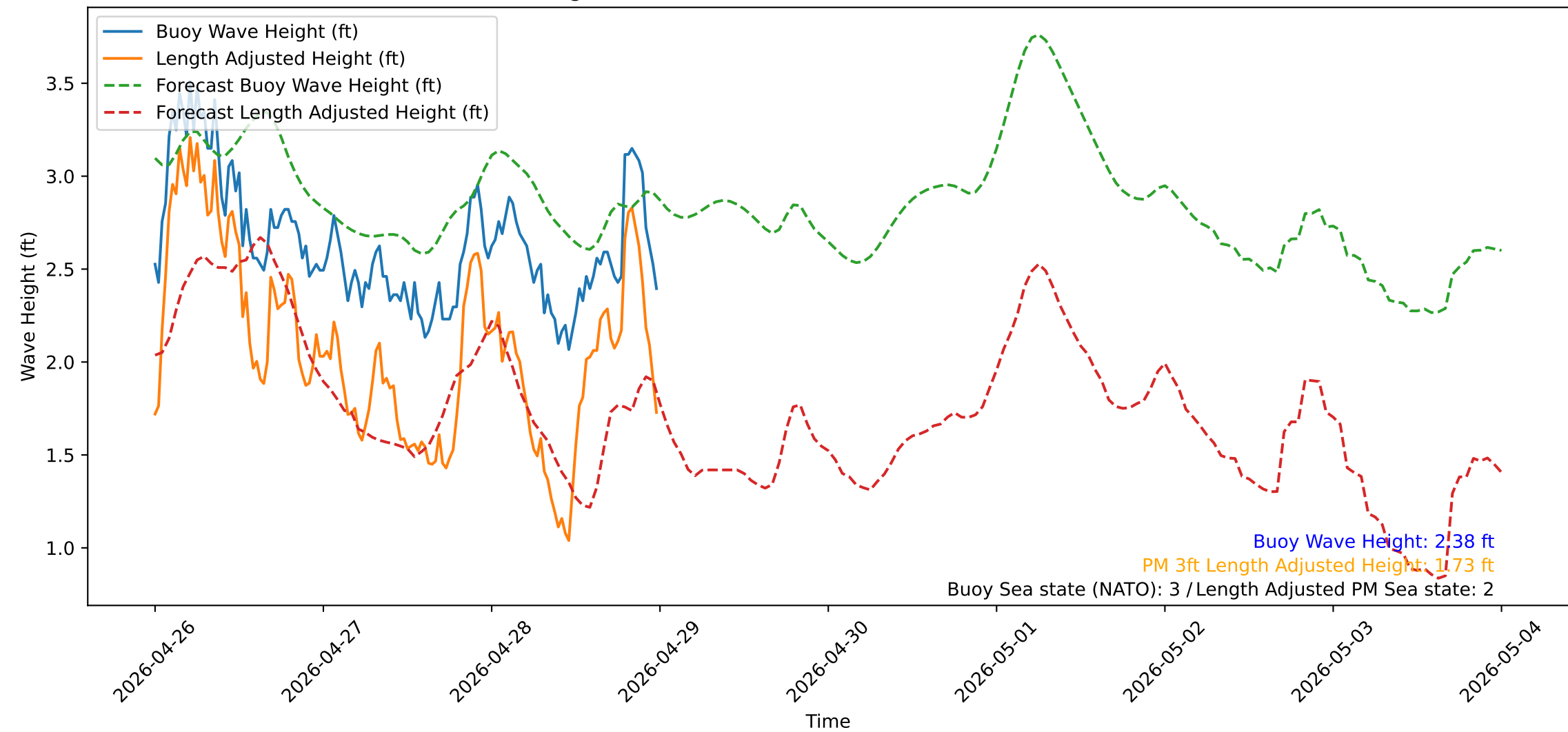
Wave Heights over Time for Green Beach at 2026-04-29 00:11:13
