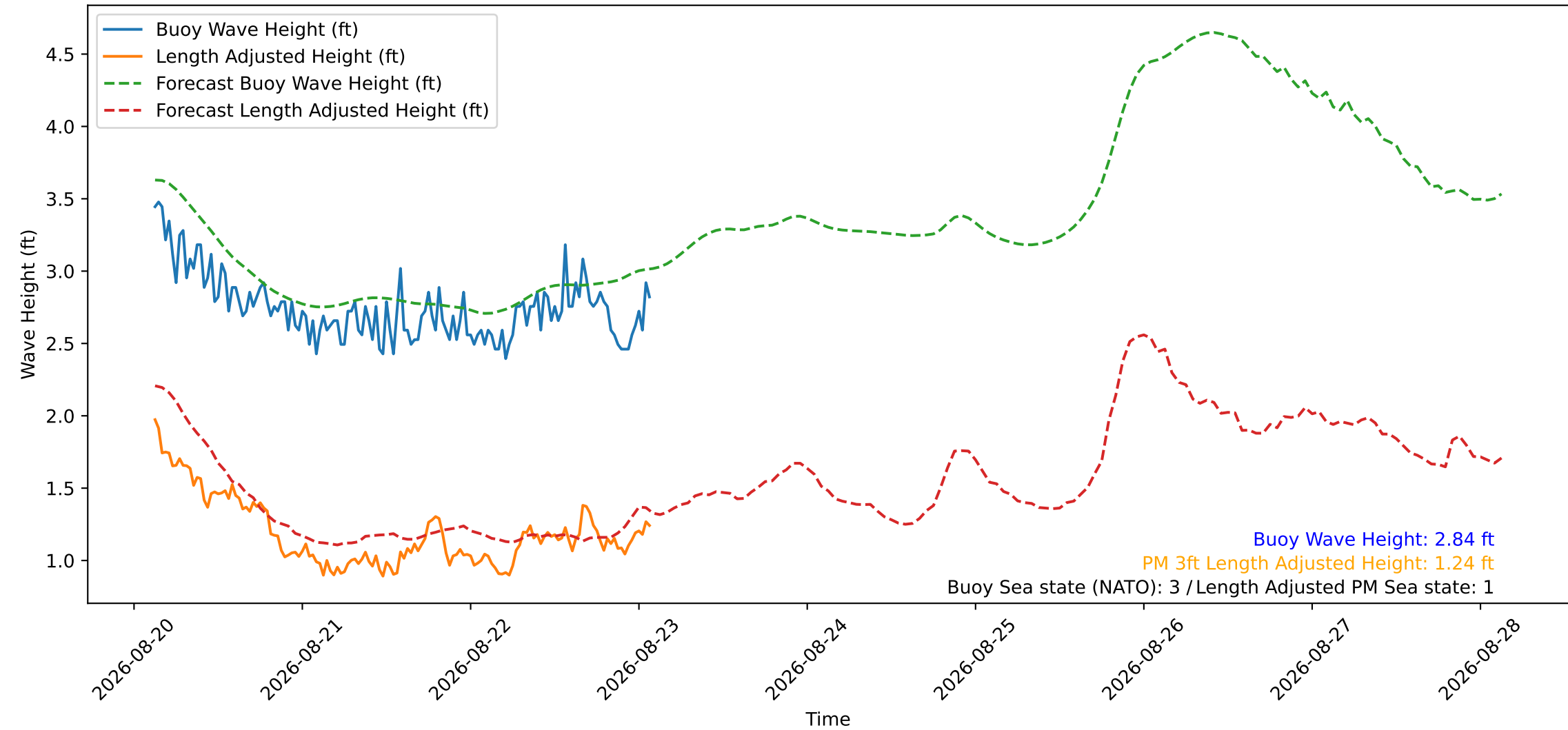
Wave Heights over Time for Green Beach at 2026-08-23 02:41:12
