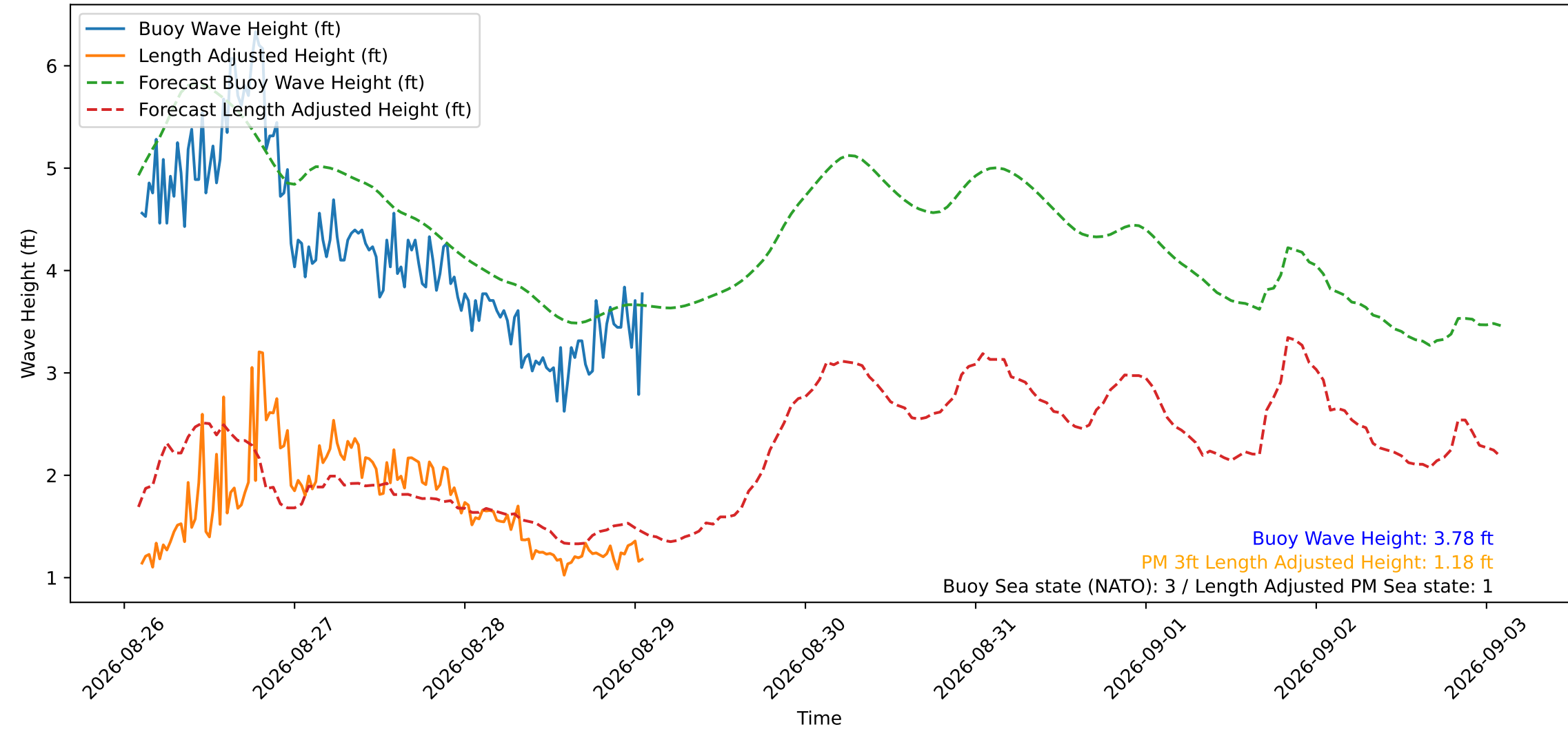
Wave Heights over Time for Green Beach at 2026-08-29 02:01:11
