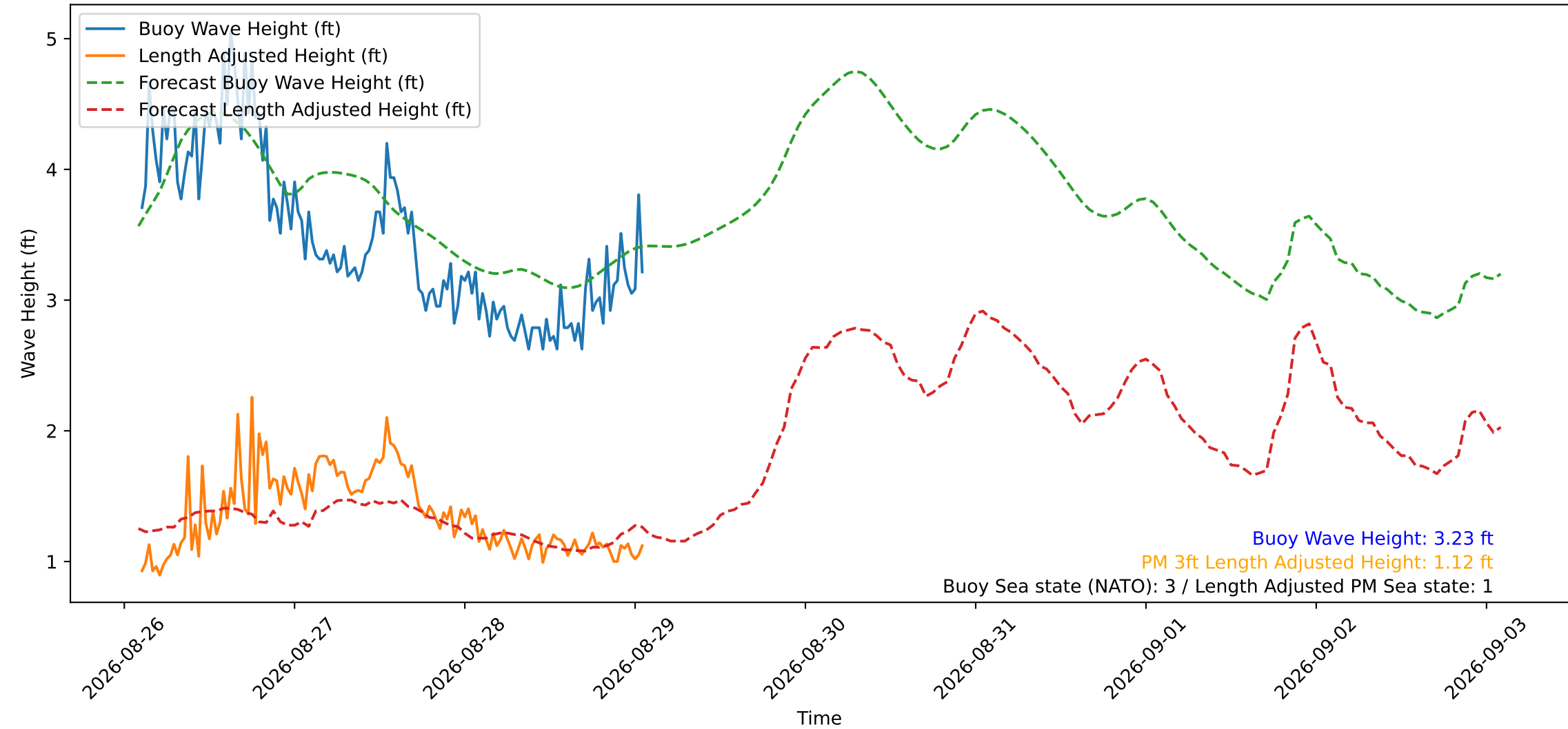
Wave Heights over Time for Red Beach at 2026-08-29 02:00:49
