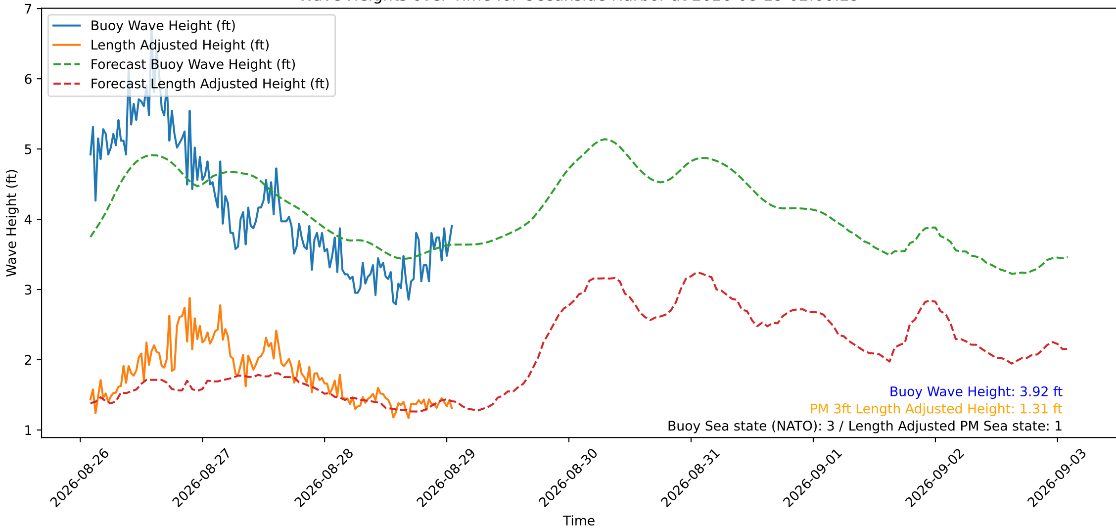
Wave Heights over Time for Oceanside Harbor at 2026-08-29 02:00:29
