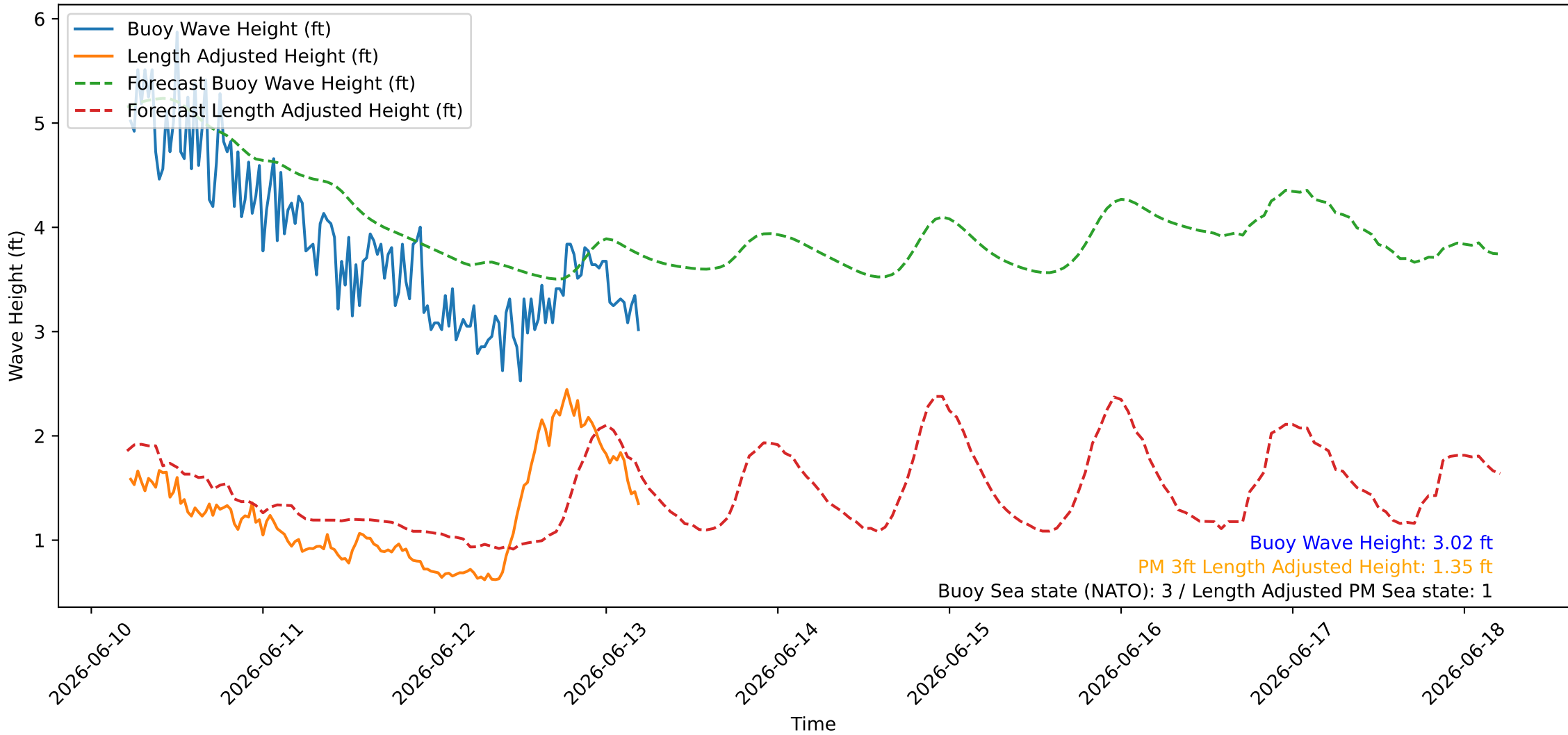
Wave Heights over Time for Red Beach at 2026-06-13 05:20:47
