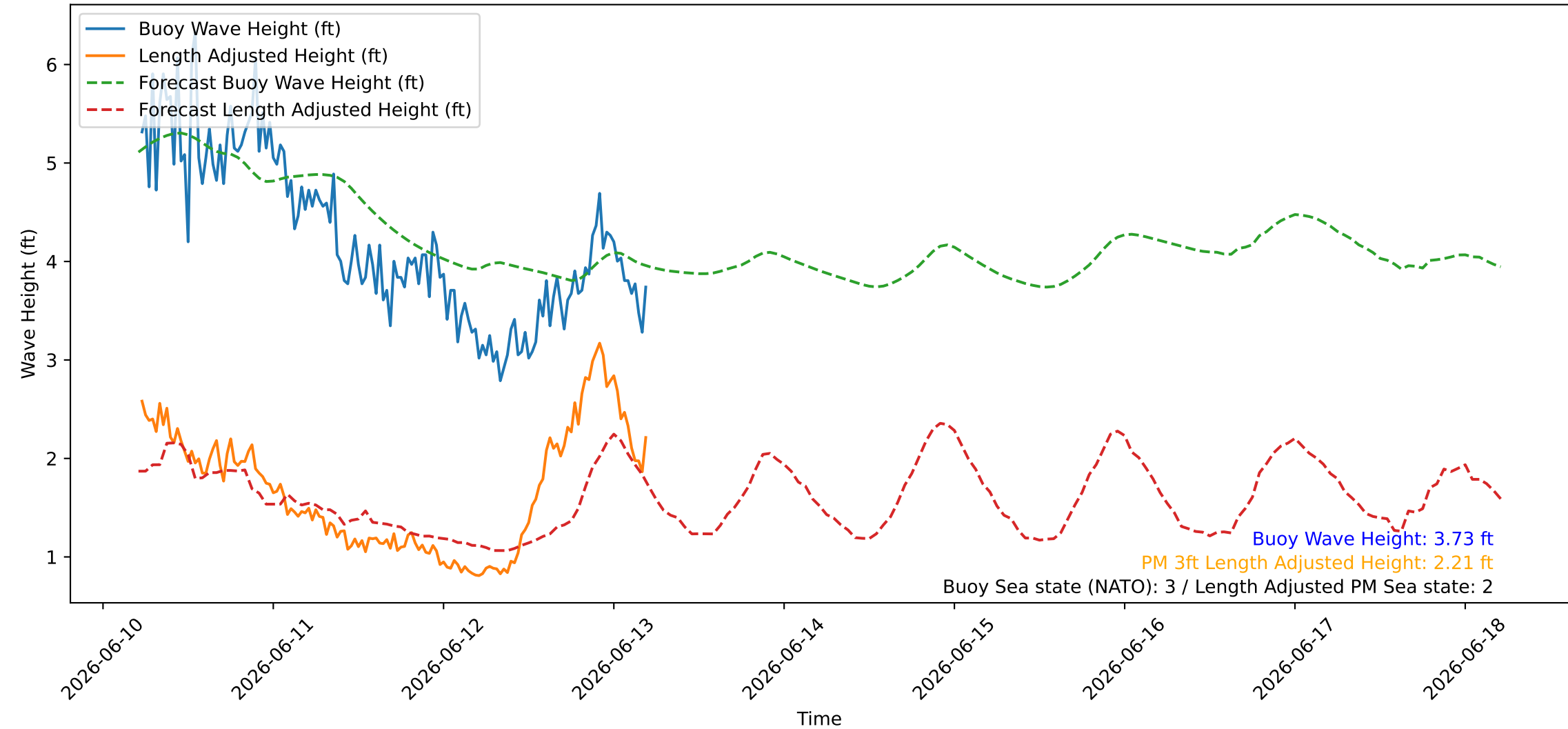
Wave Heights over Time for Oceanside Harbor at 2026-06-13 05:20:26
