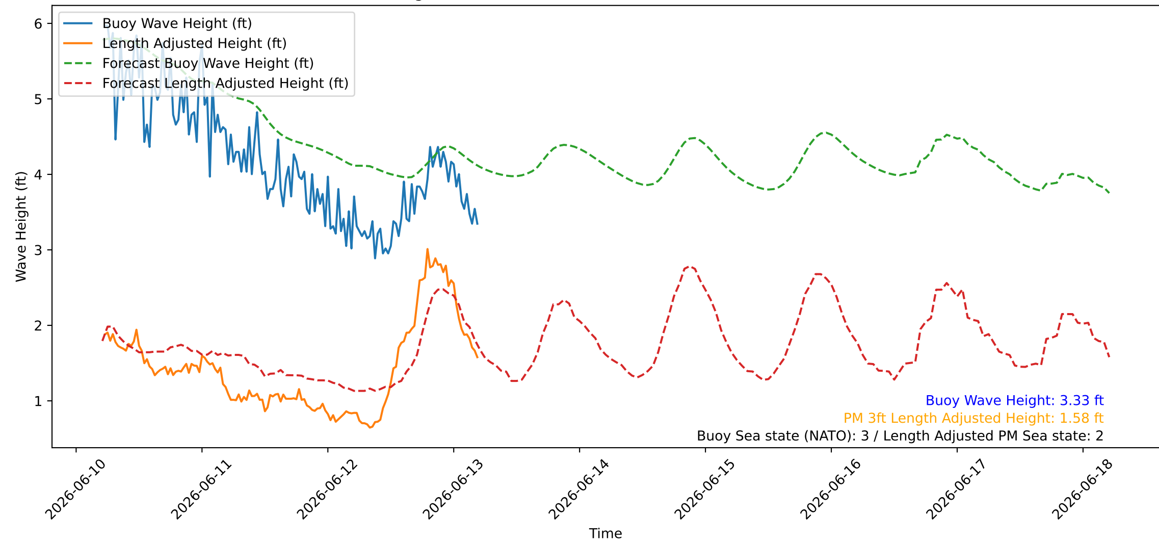
Wave Heights over Time for Green Beach at 2026-06-13 05:21:10
