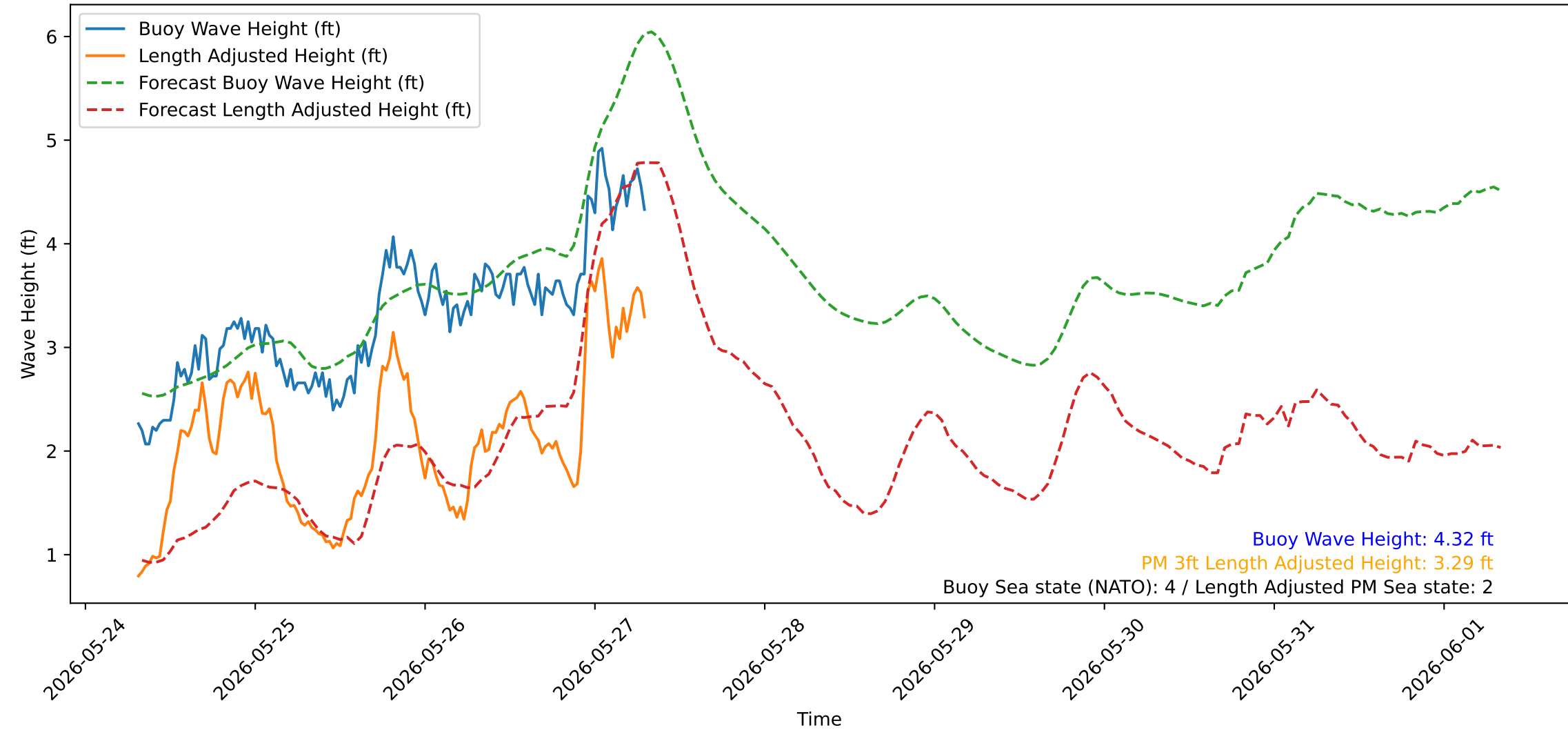
Wave Heights over Time for Green Beach at 2026-05-27 07:41:08
