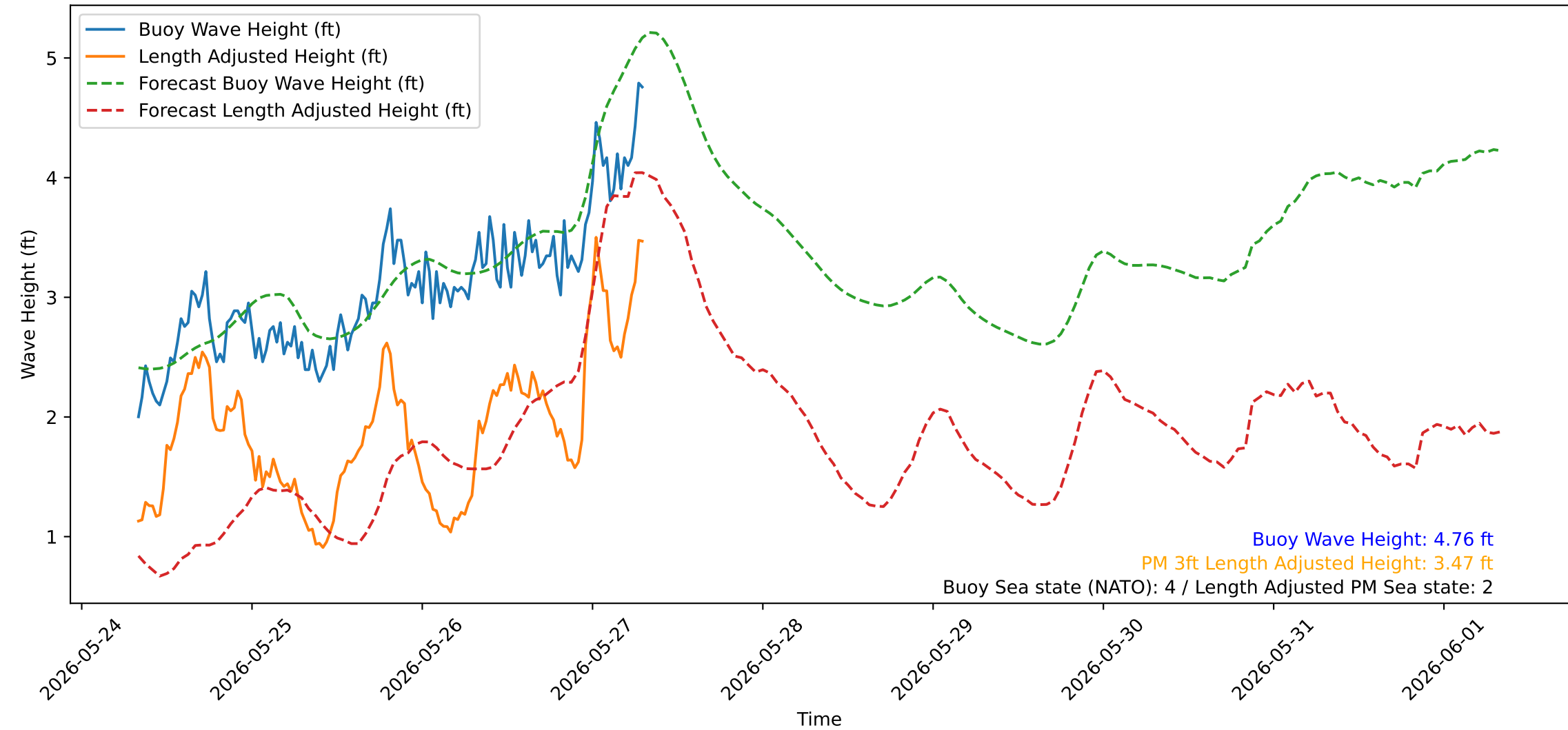
Wave Heights over Time for Red Beach at 2026-05-27 07:40:45
