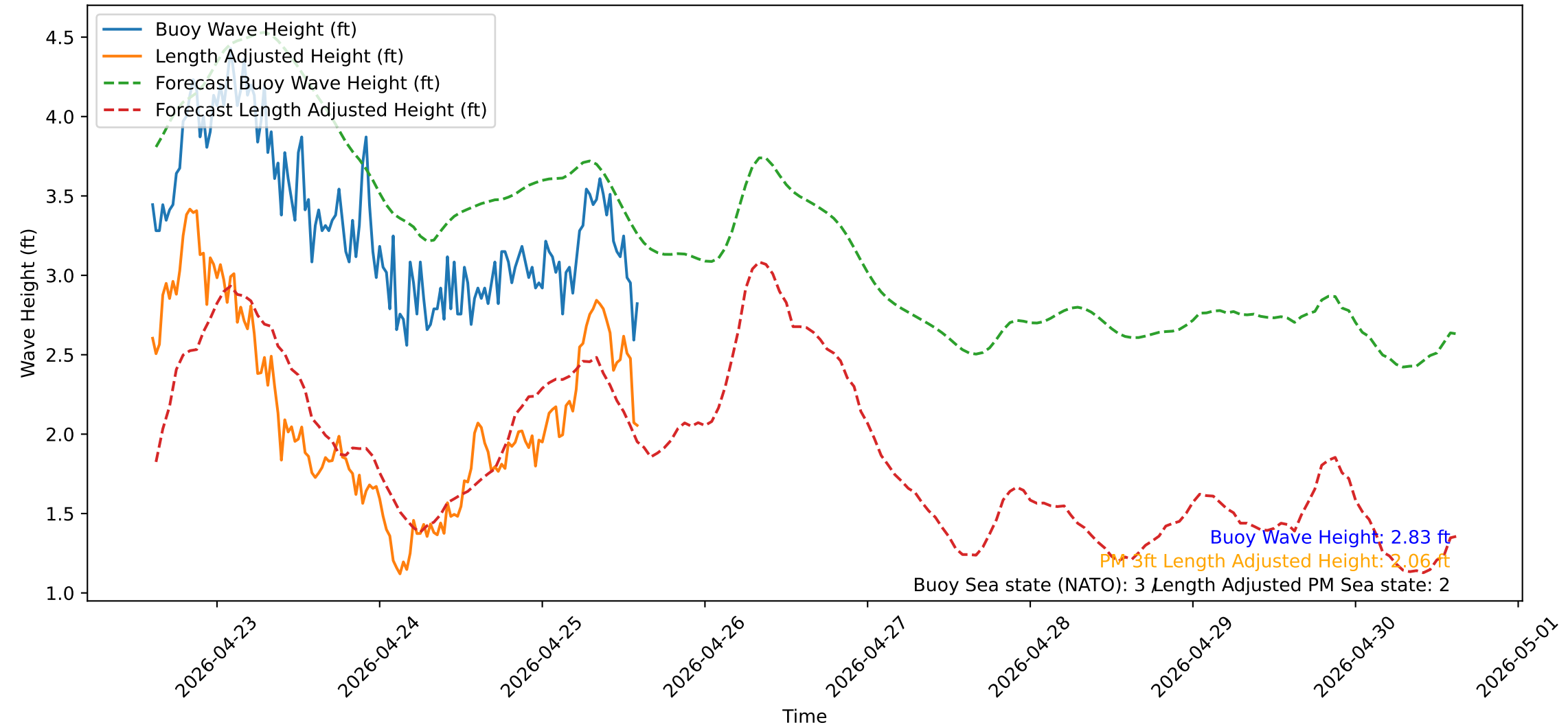
Wave Heights over Time for Oceanside Harbor at 2026-04-25 14:40:31
