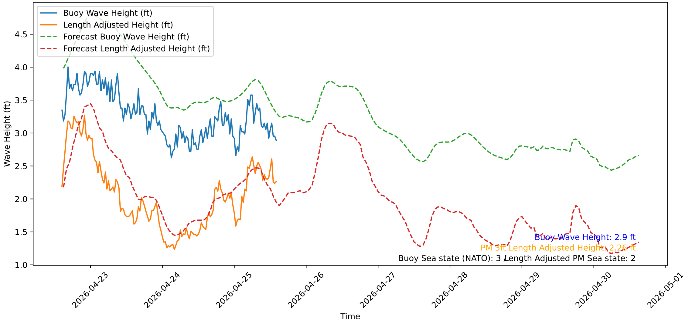
Wave Heights over Time for Green Beach at 2026-04-25 14:41:14
